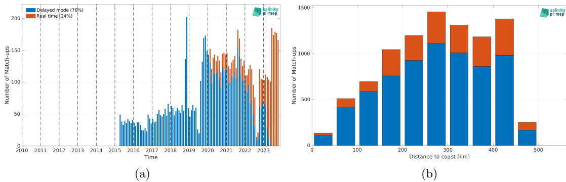
Figure 1: Number of match-ups between Argo and SMAP SSS L2 v5.0 (JPL) SSS as a function of time (a) and as function of the distance to coast (b) over the Gulf of Mexico Pi-MEP region and for the full satellite product period.
