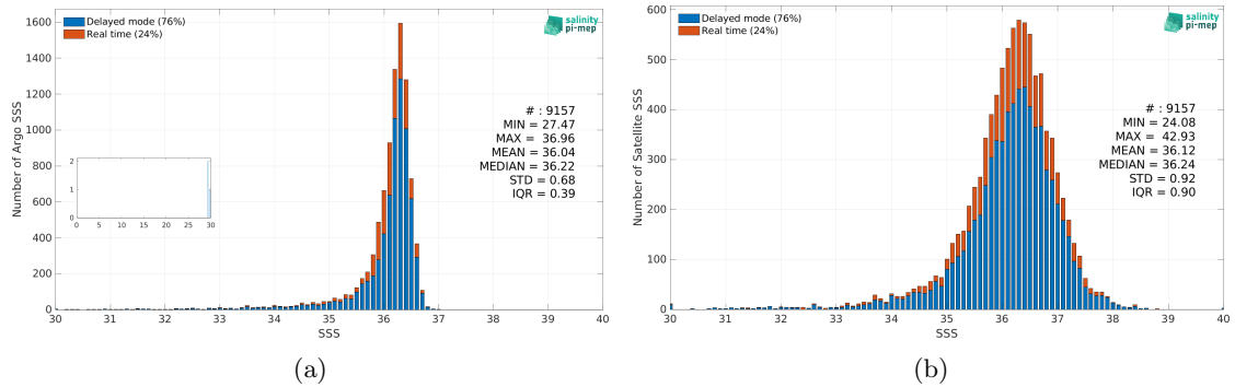
Figure 2: Histograms of SSS from Argo (a) and SMAP SSS L2 v5.0 (JPL) (b) considering all match-up pairs per bins of 0.1 over the Gulf of Mexico Pi-MEP region and for the full satellite product period.
