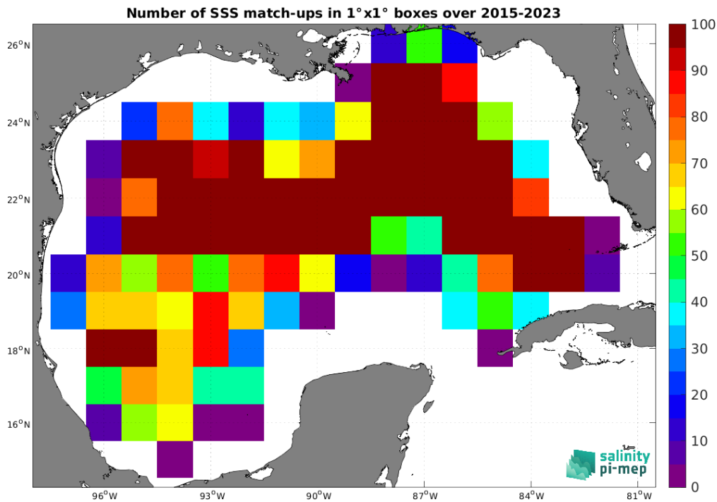
Figure 4: Number of SSS match-ups between Argo SSS and the SMAP SSS L2 v5.0 (JPL) SSS product for the Gulf of Mexico Pi-MEP region over 1^\circ \times 1^\circ boxes and for the full satellite product period.
