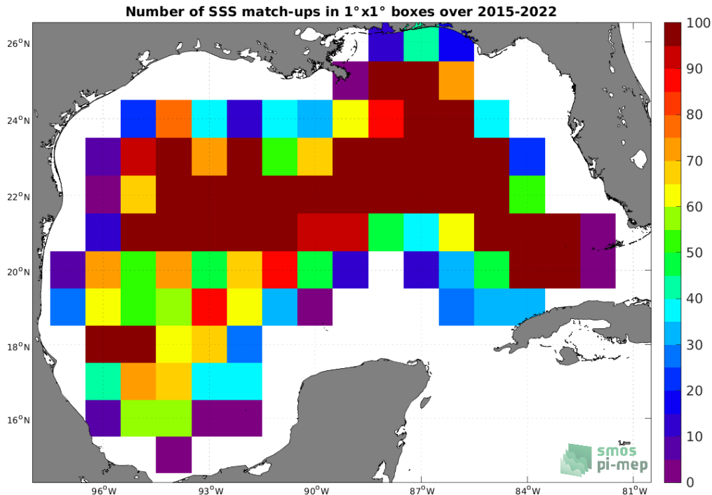
Figure 4: Number of SSS match-ups between Argo SSS and the SMAP SSS L2 v5.0 (JPL) SSS product for the Gulf of Mexico Pi-MEP region over 1^{\circ} \times 1^{\circ} boxes and for the full satellite product period.
