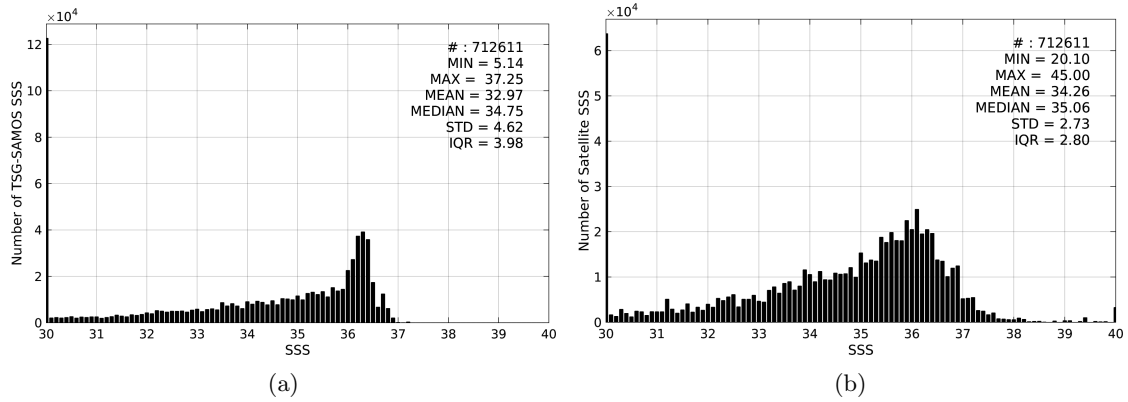
Figure 2: Histograms of SSS from TSG-SAMOS (a) and SMAP-L2-JPL-V4 (b) considering all match-up pairs per bins of 0.1 over the Gulf of Mexico Pi-MEP region and for the full satellite product period.
