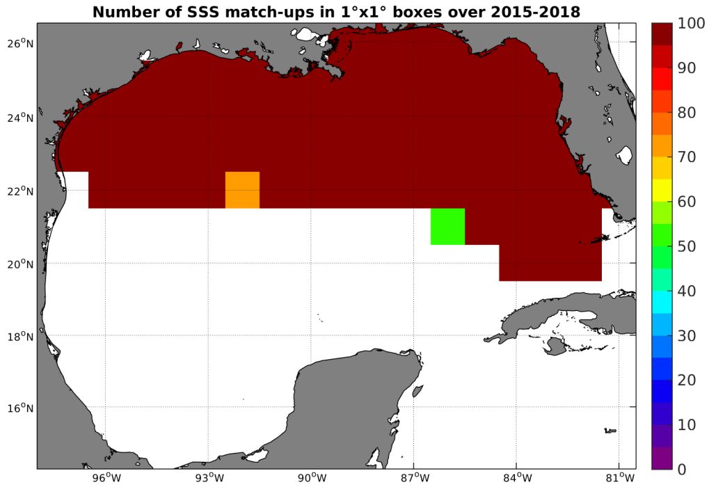
Figure 4: Number of SSS match-ups between TSG-SAMOS SSS and the SMAP-L2-JPL-V4 SSS product for the Gulf of Mexico Pi-MEP region over 1^\circ \times 1^\circ boxes and for the full satellite product period.
