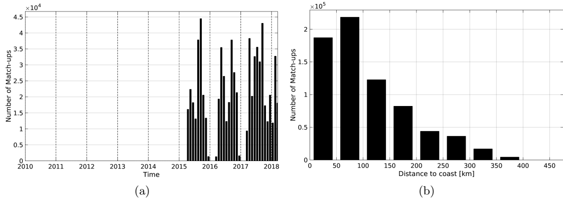
Figure 1: Number of match-ups between TSG-SAMOS and SMAP-L2-JPL-V4 SSS as a function of time (a) and as function of the distance to coast (b) over the Gulf of Mexico Pi-MEP region and for the full satellite product period.
