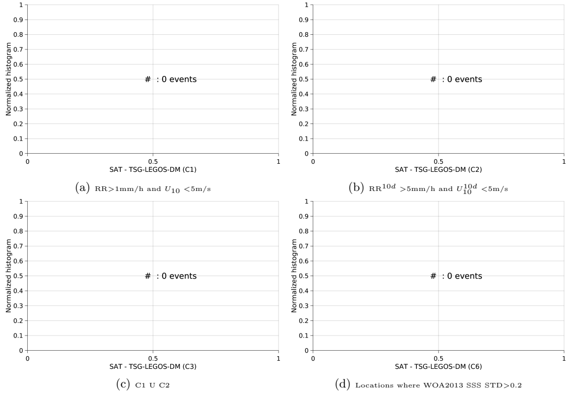
Figure 13: Normalized histogram of \Delta\text{SSS} (SMAP-L2-JPL-V4 - TSG-LEGOS-DM) for 6 different subdatasets corresponding to: RR > 1\text{mm/h} and U_{10} < 5\text{m/s} (a), RR^{10d} > 5\text{mm/h} and U_{10}^{10d} < 5\text{m/s} (b), C1 \cup C2 (c), Locations where WOA2013 SSS STD > 0.2 (d).
