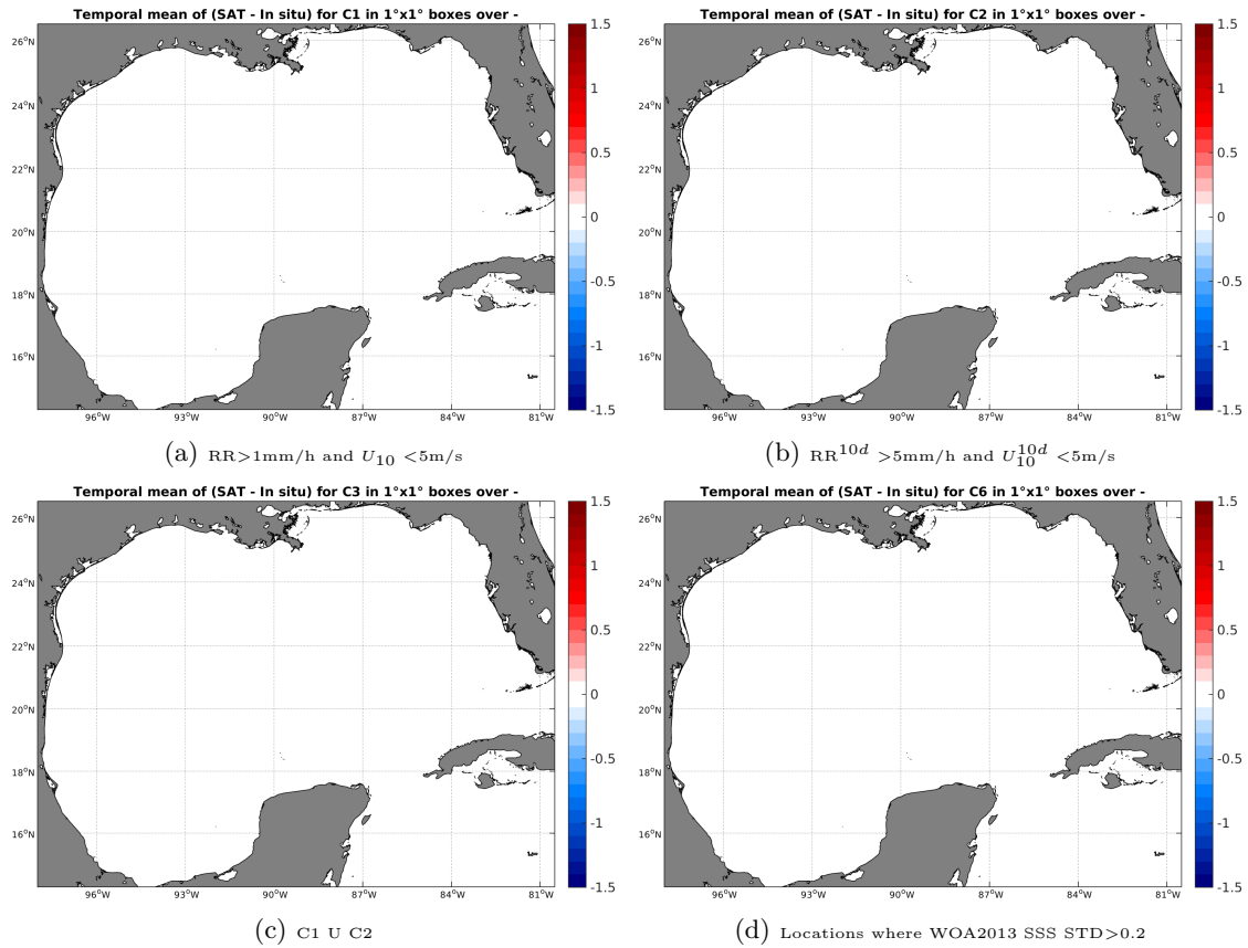
Figure 12: Temporal mean gridded over spatial boxes of size 1^\circ \times 1^\circ of \Delta SSS (SMAP-L2-JPL-V4 - TSG-LEGOS-DM) for 4 different subdatasets corresponding to:RR > 1mm/h and U_{10} < 5 m/s (a), RR 10d > 5mm/h and U_{10}^{10d} < 5 m/s (b), C1 U C2 (c),Locations where WOA2013 SSS STD > 0.2 (d).
