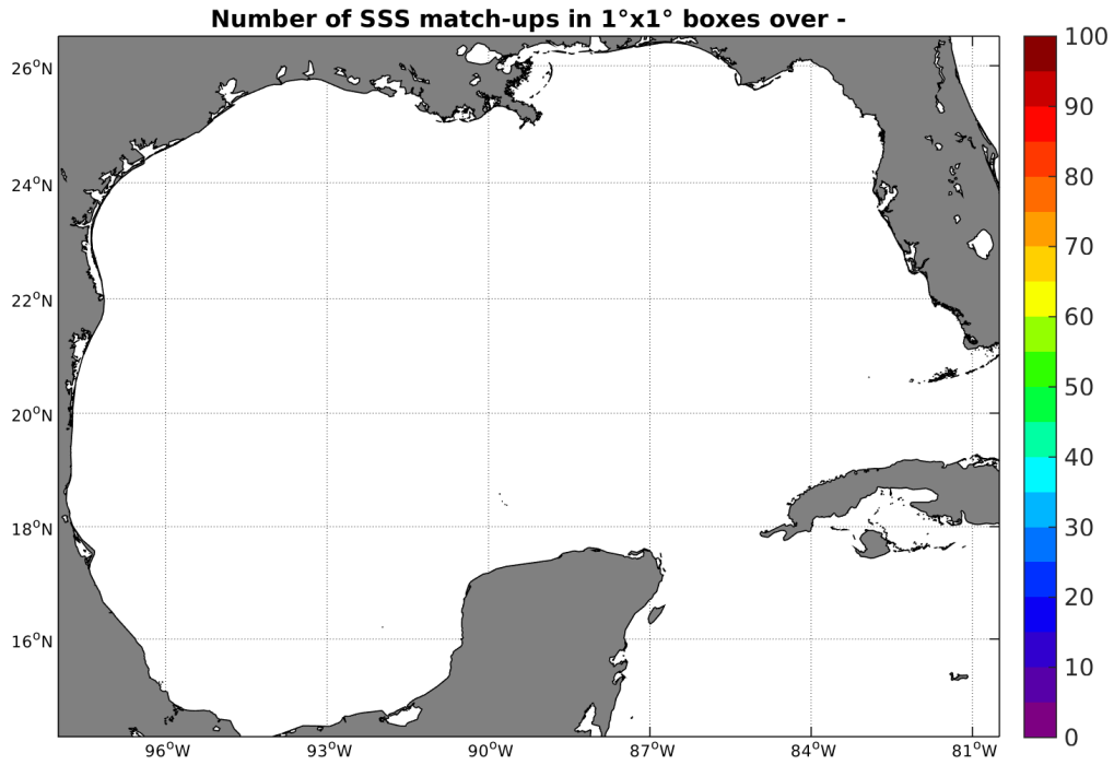
Figure 4: Number of SSS match-ups between TSG-LEGOS-DM SSS and the SMAP-L2-JPL-V4 SSS product for the Gulf of Mexico Pi-MEP region over 1°x1° boxes and for the full satellite product period.
