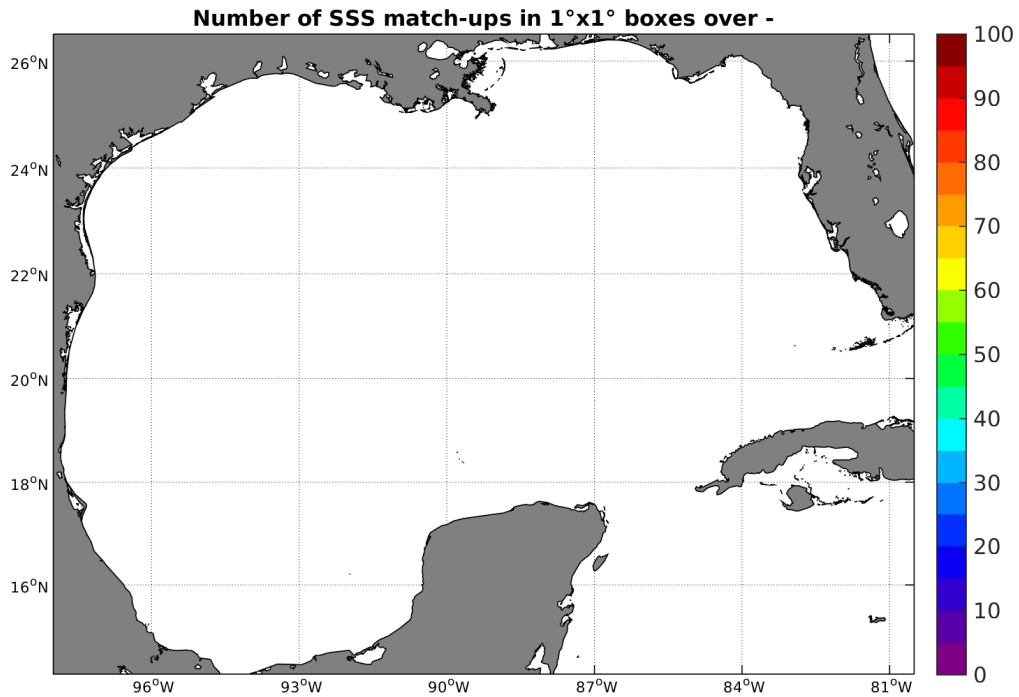
Figure 4: Number of SSS match-ups between TSG-LEGOS-DM SSS and the SMAP-L2-JPL-V4 SSS product for the Gulf of Mexico Pi-MEP region over 1^\circ \times 1^\circ boxes and for the full satellite product period.
