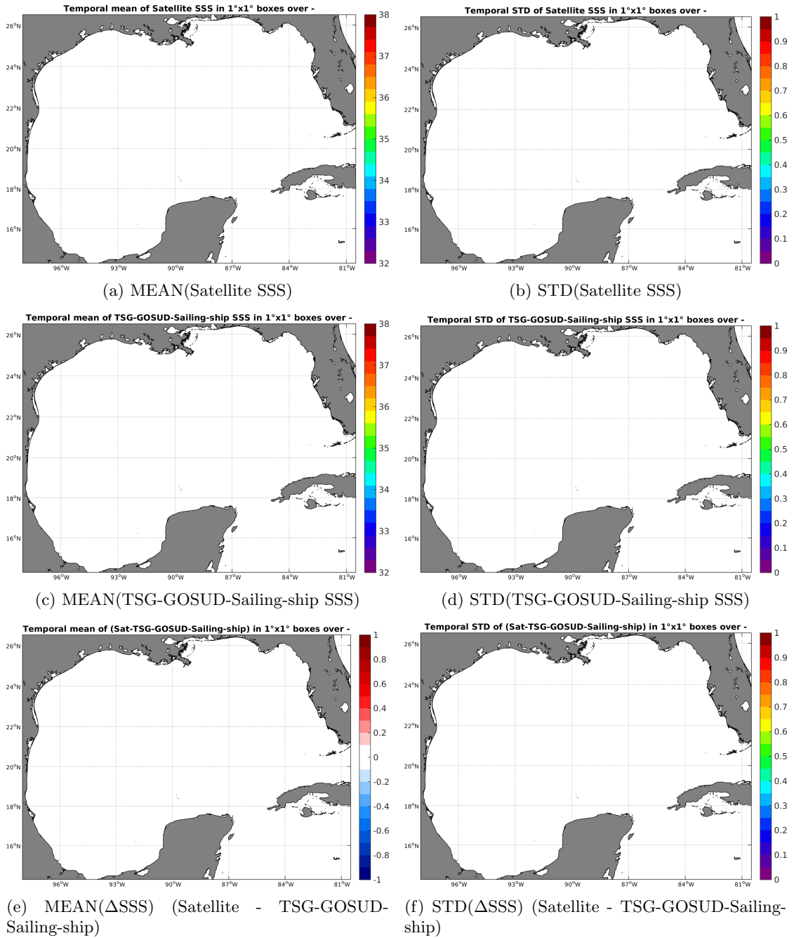
Figure 6: Temporal mean (left) and STD (right) of SSS from SMAP-L2-JPL-V4 (top), TSG-GOSUD-Sailing-ship (middle), and of \Delta SSS (Satellite - TSG-GOSUD-Sailing-ship). Only match-up pairs are used to generate these maps.
