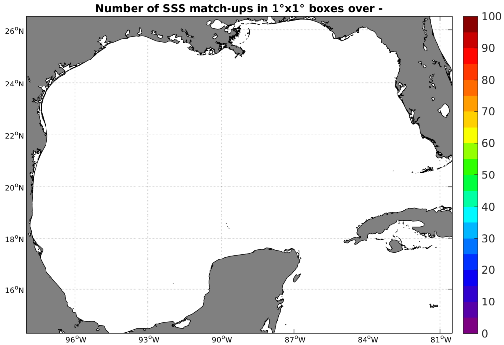
Figure 4: Number of SSS match-ups between TSG-GOSUD-Sailing-ship SSS and the SMAP-L2-JPL-V4 SSS product for the Gulf of Mexico Pi-MEP region over 1°x1° boxes and for the full satellite product period.
