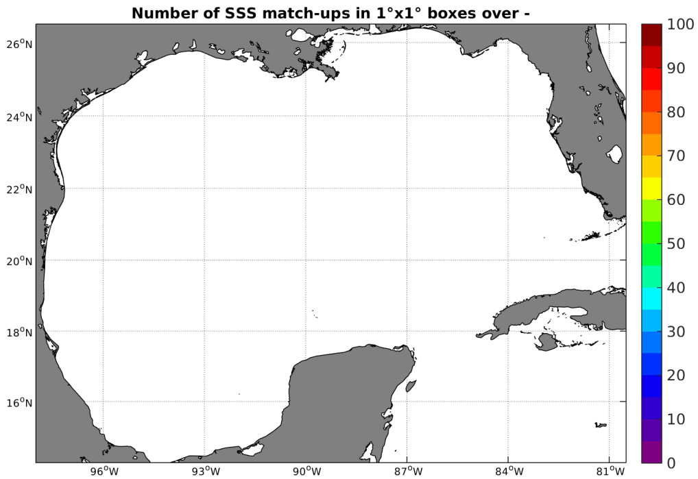
Figure 3: Number of SSS match-ups between Surface drifters SSS and the SMAP-L2-JPL-V4 SSS product for the Gulf of Mexico Pi-MEP region over 1°x1° boxes and for the full satellite product period.
