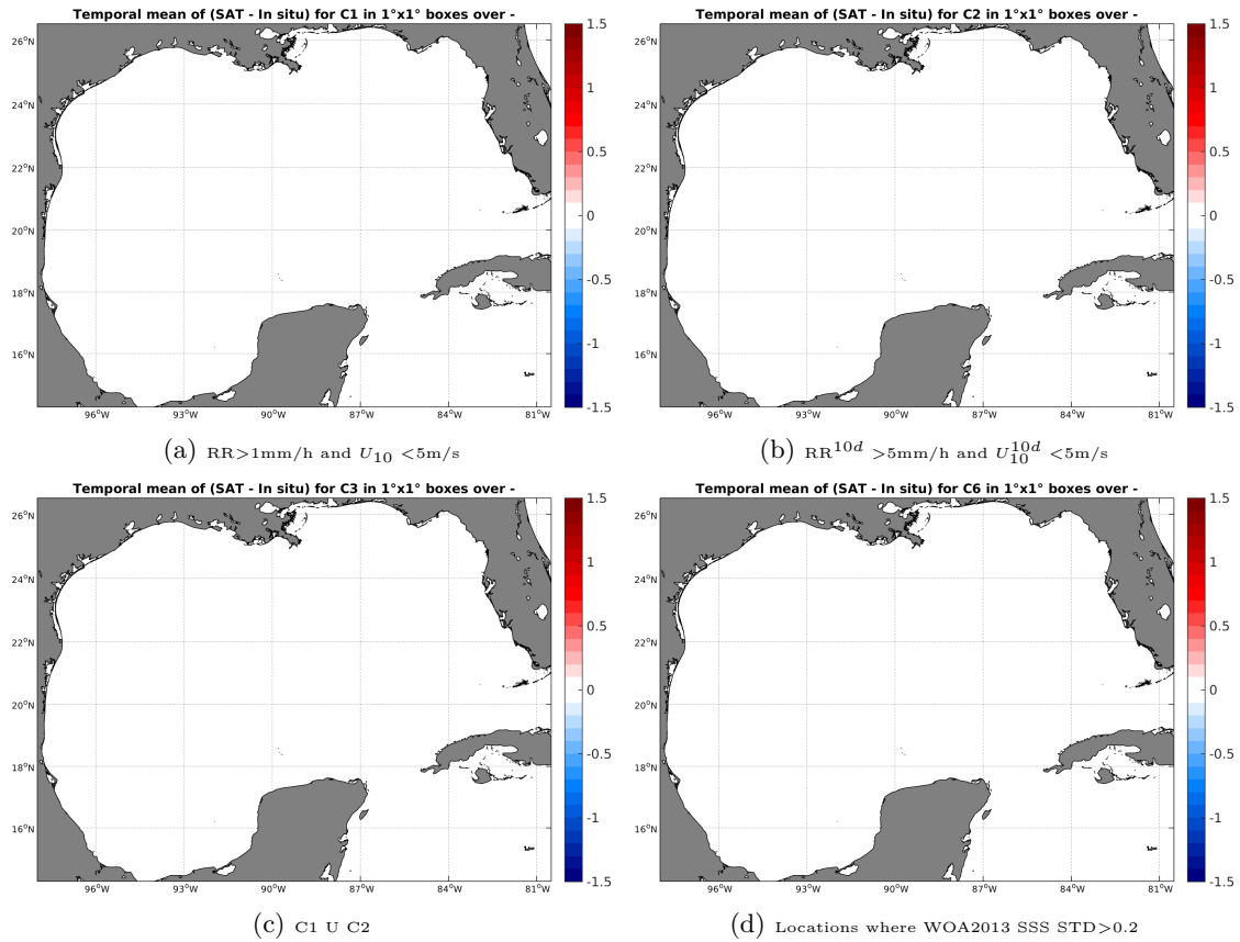
Figure 11: Temporal mean gridded over spatial boxes of size 1^\circ \times 1^\circ of \Delta SSS (SMAP-L2-JPL-V4 - Surface drifters) for 4 different subdatasets corresponding to: RR > 1mm/h and U_{10} < 5\text{m/s} (a), RR^{10d} > 5\text{mm/h} and U_{10}^{10d} < 5\text{m/s} (b), C1 U C2 (c), Locations where WOA2013 SSS STD > 0.2 (d).
