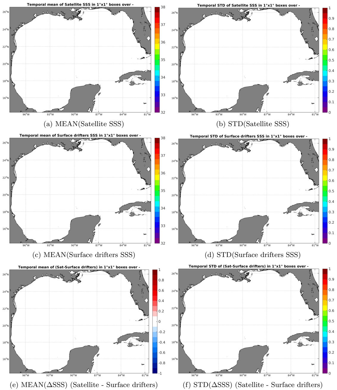
Figure 5: Temporal mean (left) and STD (right) of SSS from SMAP-L2-JPL-V4 (top), Surface drifters (middle), and of \Delta SSS (Satellite - Surface drifters). Only match-up pairs are used to generate these maps.
