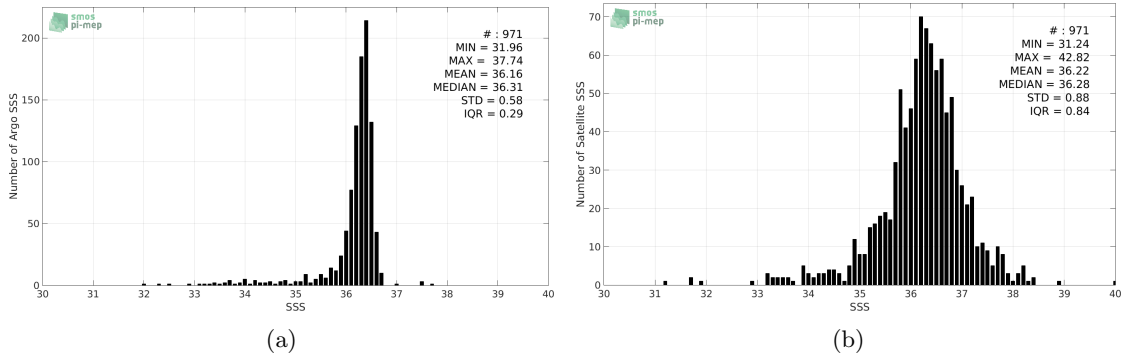
Figure 2: Histograms of SSS from Argo (a) and SMAP-L2-JPL-V4 (b) considering all match-up pairs per bins of 0.1 over the Gulf of Mexico Pi-MEP region and for the full satellite product period.
