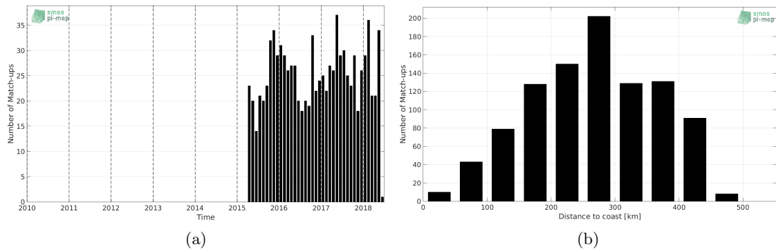
Figure 1: Number of match-ups between Argo and SMAP-L2-JPL-V4 SSS as a function of time (a) and as function of the distance to coast (b) over the Gulf of Mexico Pi-MEP region and for the full satellite product period.
