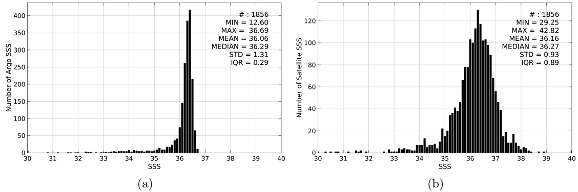
Figure 2: Histograms of SSS from Argo (a) and SMAP-L2-JPL-V4 (b) considering all match-up pairs per bins of 0.1 over the Gulf of Mexico Pi-MEP region and for the full satellite product period.
