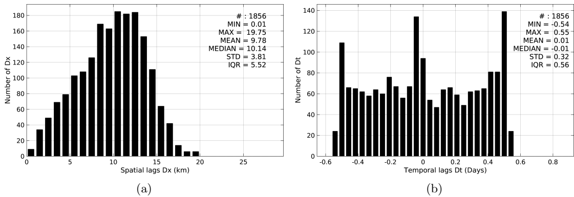
Figure 5: Histograms of the spatial (a) and temporal (b) lags between the time of the Argo measurements and the date of the corresponding SMAP-L2-JPL-V4 SSS product.
