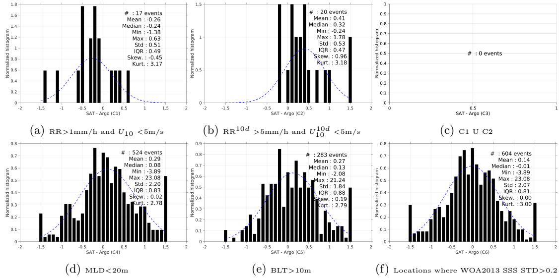
Figure 13: Normalized histogram of \Delta SSS (SMAP-L2-JPL-V4 - Argo) for 6 different subdatasets corresponding to: RR>1mm/h and U_{10} < 5\text{m/s} (a), RR^{10d} > 5\text{mm/h} and U_{10}^{10d} < 5\text{m/s} (b), C1 U C2 (c),MLD<20m (d),BLT>10m (e),Locations where WOA2013 SSS STD>0.2 (f).
