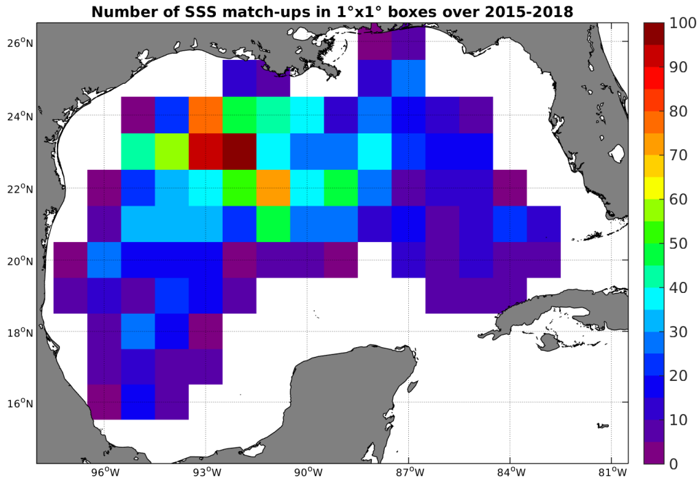
Figure 4: Number of SSS match-ups between Argo SSS and the SMAP-L2-JPL-V4 SSS product for the Gulf of Mexico Pi-MEP region over 1^\circ \times 1^\circ boxes and for the full satellite product period.
