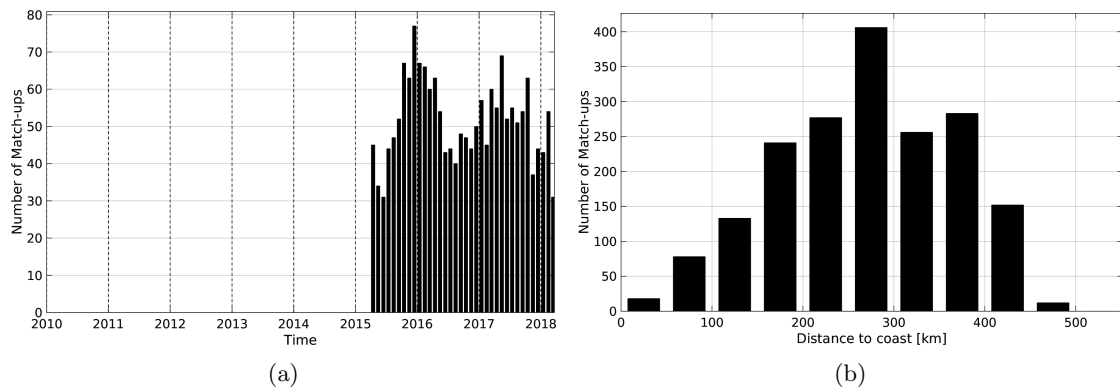
Figure 1: Number of match-ups between Argo and SMAP-L2-JPL-V4 SSS as a function of time (a) and as function of the distance to coast (b) over the Gulf of Mexico Pi-MEP region and for the full satellite product period.
