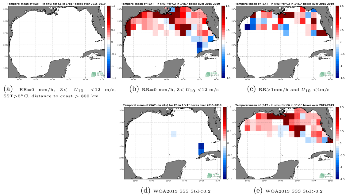
Figure 12: Temporal mean gridded over spatial boxes of size 1^\circ \times 1^\circ of \Delta SSS (SMAP-L2-JPL-V4.2 - TSG-SAMOS) for 5 different subdatasets corresponding to:RR=0 mm/h, 3 < U_{10} < 12 m/s, SST >5^\circ\text{C} , distance to coast > 800 km (a), RR=0 mm/h, 3 < U_{10} < 12 m/s (b), RR >1 mm/h and U_{10} < 4 m/s (c), WOA2013 SSS Std <0.2 (d), WOA2013 SSS Std >0.2 (e).
