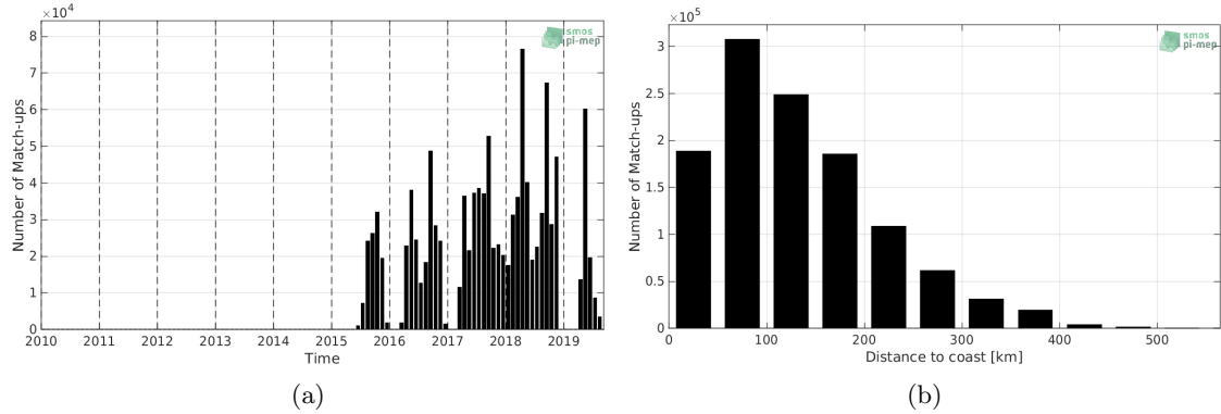
Figure 1: Number of match-ups between TSG-SAMOS and SMAP-L2-JPL-V4.2 SSS as a function of time (a) and as function of the distance to coast (b) over the Gulf of Mexico Pi-MEP region and for the full satellite product period.
