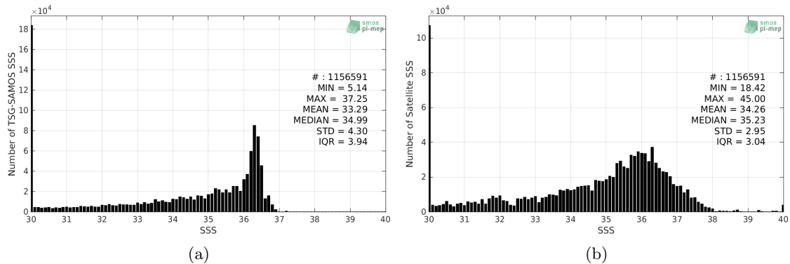
Figure 2: Histograms of SSS from TSG-SAMOS (a) and SMAP-L2-JPL-V4.2 (b) considering all match-up pairs per bins of 0.1 over the Gulf of Mexico Pi-MEP region and for the full satellite product period.
