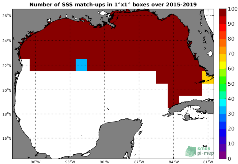
Figure 4: Number of SSS match-ups between TSG-SAMOS SSS and the SMAP-L2-JPL-V4.2 SSS product for the Gulf of Mexico Pi-MEP region over 1°x1° boxes and for the full satellite product period.
