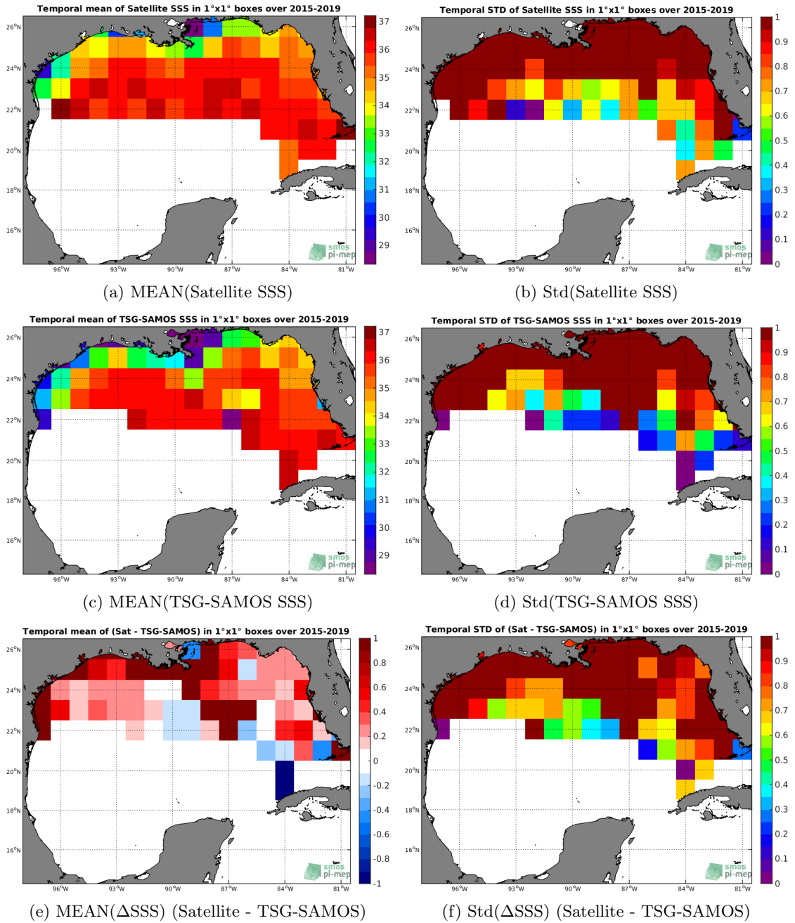
Figure 6: Temporal mean (left) and Std (right) of SSS from SMAP-L2-JPL-V4.2 (top), TSG-SAMOS (middle), and of \Delta SSS (Satellite - TSG-SAMOS). Only match-up pairs are used to generate these maps.
