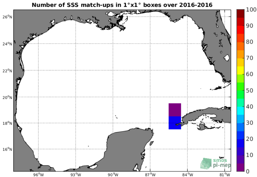
Figure 4: Number of SSS match-ups between TSG-LEGOS-DM SSS and the SMAP-L2-JPL-V4.2 SSS product for the Gulf of Mexico Pi-MEP region over 1°x1° boxes and for the full satellite product period.
