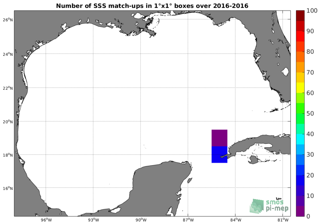
Figure 4: Number of SSS match-ups between TSG-LEGOS-DM SSS and the SMAP-L2-JPL-V4.2 SSS product for the Gulf of Mexico Pi-MEP region over 1^\circ \times 1^\circ boxes and for the full satellite product period.
