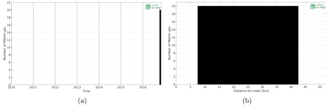
Figure 1: Number of match-ups between TSG-LEGOS-DM and SMAP-L2-JPL-V4.2 SSS as a function of time (a) and as function of the distance to coast (b) over the Gulf of Mexico Pi-MEP region and for the full satellite product period.
