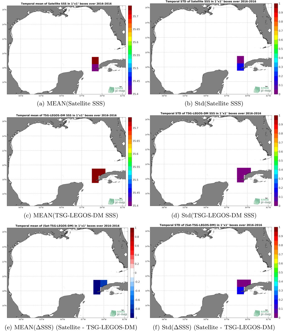
Figure 6: Temporal mean (left) and Std (right) of SSS from SMAP-L2-JPL-V4.2 (top), TSG-LEGOS-DM (middle), and of \Delta SSS (Satellite - TSG-LEGOS-DM). Only match-up pairs are used to generate these maps.
