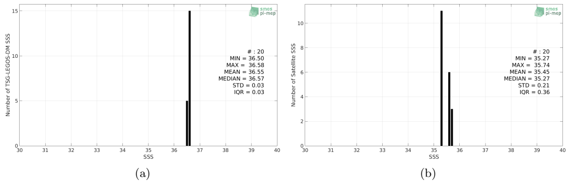
Figure 2: Histograms of SSS from TSG-LEGOS-DM (a) and SMAP-L2-JPL-V4.2 (b) considering all match-up pairs per bins of 0.1 over the Gulf of Mexico Pi-MEP region and for the full satellite product period.
