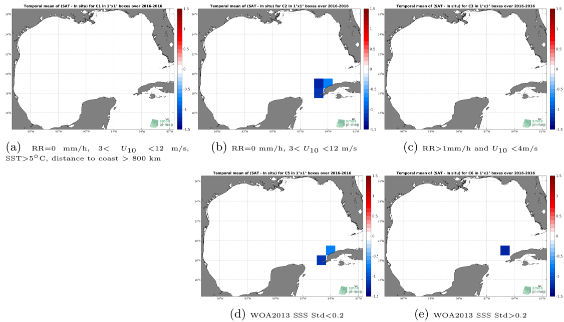
Figure 12: Temporal mean gridded over spatial boxes of size 1^\circ \times 1^\circ of \Delta SSS (SMAP-L2-JPL-V4.2 - TSG-LEGOS-DM) for 5 different subdatasets corresponding to:RR=0 mm/h, 3 < U_{10} < 12 m/s, SST >5^\circ\text{C} , distance to coast > 800 km (a), RR=0 mm/h, 3 < U_{10} < 12 m/s (b), RR >1 mm/h and U_{10} < 4 m/s (c), WOA2013 SSS Std <0.2 (d), WOA2013 SSS Std >0.2 (e).
