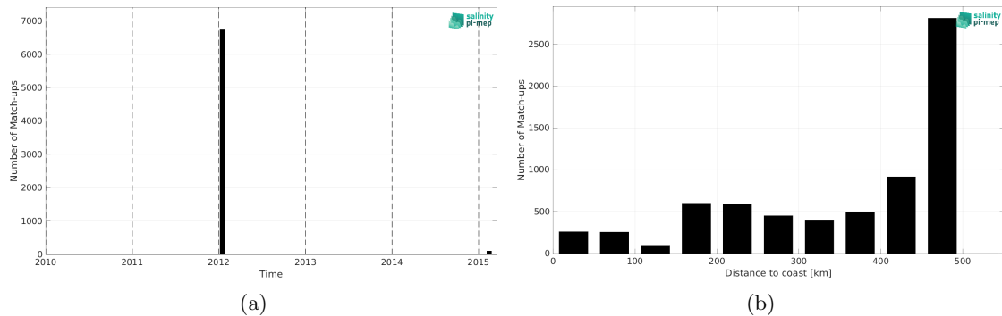
Figure 2: Number of match-ups between TSG (GOSUD-Sailing-ship) and ISAS v7 - Monthly (Ifremer-LOPS-CMEMS) SSS as a function of time (a) and as function of the distance to coast (b) over the Gulf of Mexico Pi-MEP region and for the full satellite product period.
