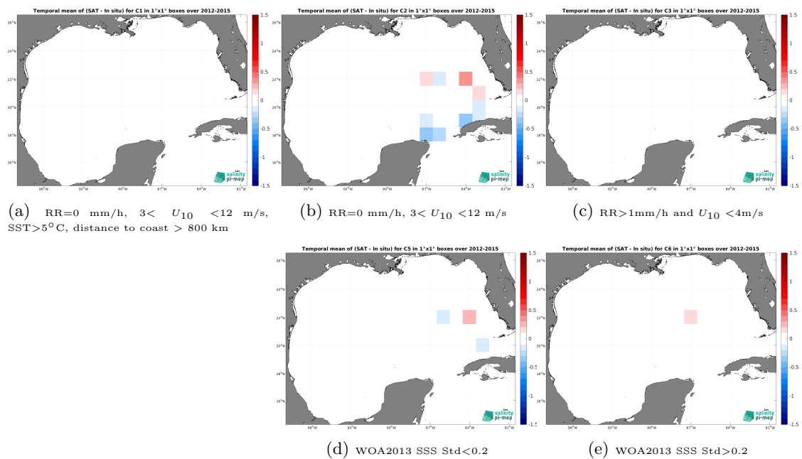
Figure 14: Temporal mean gridded over spatial boxes of size 1^\circ \times 1^\circ of \Delta SSS (ISAS v7 - Monthly (Ifremer-LOPS-CMEMS) - TSG (GOSUD-Sailing-ship)) for 5 different subdatasets corresponding to:RR=0 mm/h, 3 < U_{10} < 12 m/s, SST >5^\circ C, distance to coast > 800 km (a), RR=0 mm/h, 3 < U_{10} < 12 m/s (b), RR >1 mm/h and U_{10} < 4 m/s (c), WOA2013 SSS Std <0.2 (d), WOA2013 SSS Std >0.2 (e).
