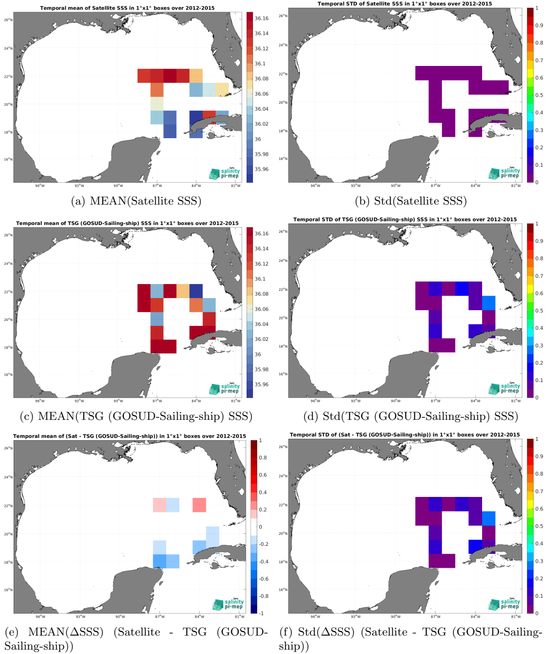
Figure 7: Temporal mean (left) and Std (right) of SSS from ISAS v7 - Monthly (Ifremer-LOPS-CMEMS) (top), TSG (GOSUD-Sailing-ship) (middle), and of \Delta SSS (Satellite - TSG (GOSUD-Sailing-ship)). Only match-up pairs are used to generate these maps.
