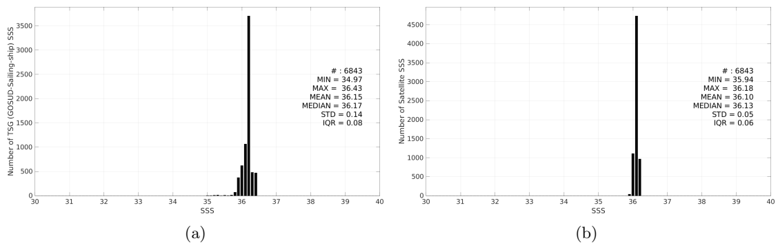
Figure 3: Histograms of SSS from TSG (GOSUD-Sailing-ship) (a) and ISAS v7 - Monthly (Ifremer-LOPS-CMEMS) (b) considering all match-up pairs per bins of 0.1 over the Gulf of Mexico Pi-MEP region and for the full satellite product period.
