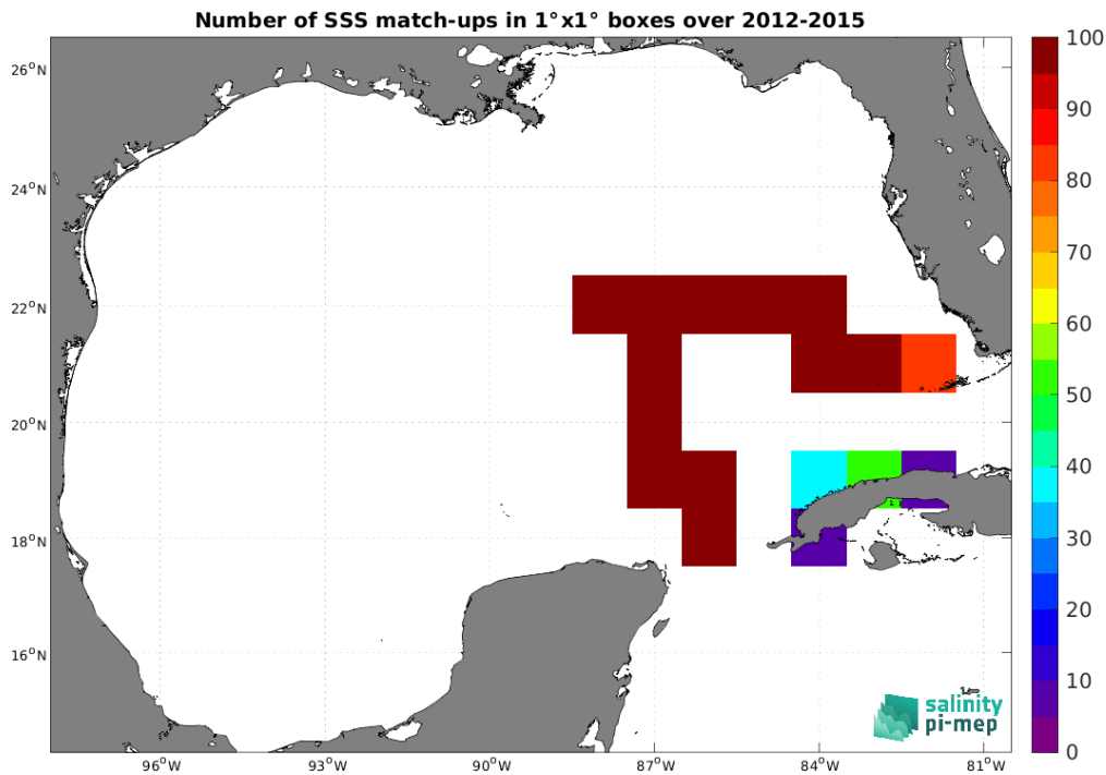
Figure 5: Number of SSS match-ups between TSG (GOSUD-Sailing-ship) SSS and the ISAS v7 - Monthly (Ifremer-LOPS-CMEMS) SSS product for the Gulf of Mexico Pi-MEP region over 1^\circ \times 1^\circ boxes and for the full satellite product period.
