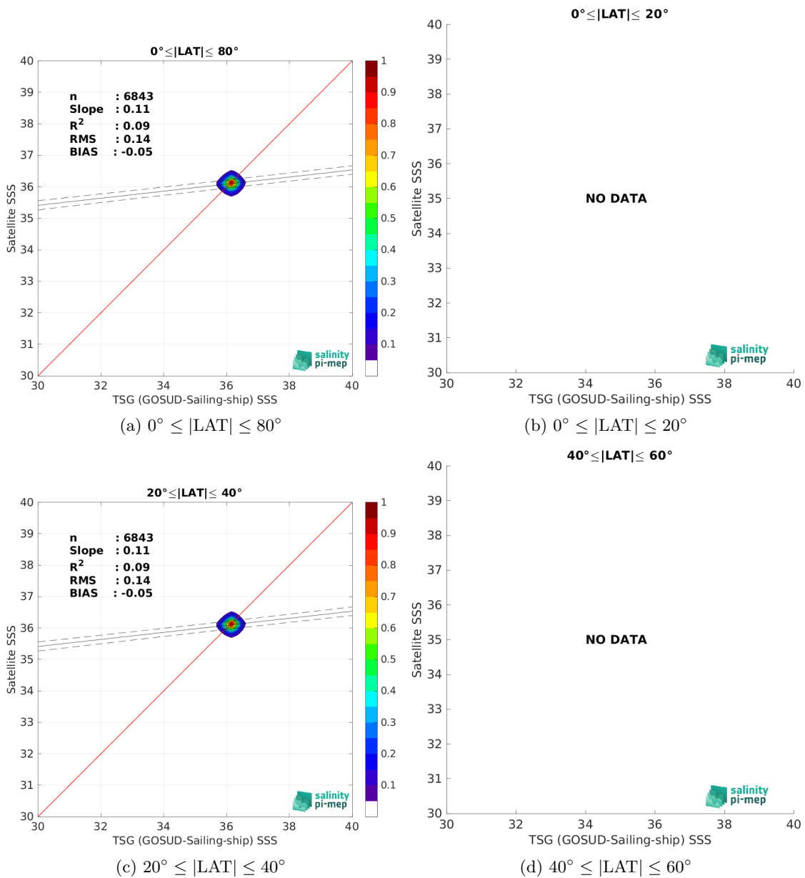
Figure 10: Contour maps of the concentration of ISAS SSS (y-axis) versus TSG (GOSUD-Sailing-ship) SSS (x-axis) at match-up pairs for different latitude bands. For each plot, the red line shows x=y . The black thin and dashed lines indicate a linear fit through the data cloud and the \pm 95\% confidence levels, respectively. The number match-up pairs n , the slope and R^2 coefficient of the linear fit, the root mean square (RMS) and the mean bias between satellite and in situ data are indicated for each latitude band in each plots.
