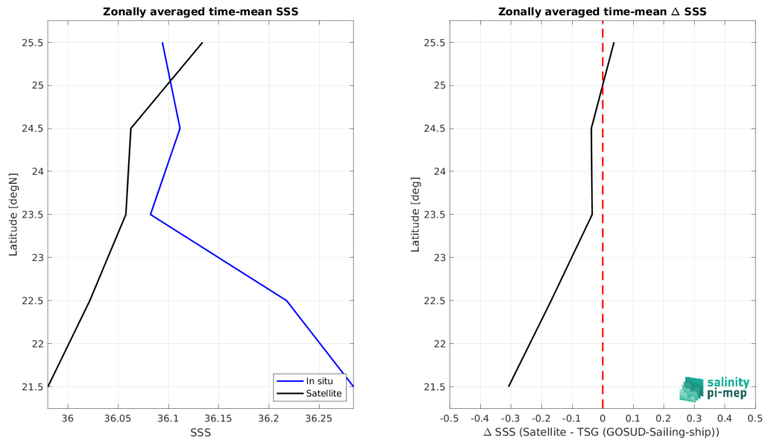
Figure 9: Left panel: Zonal mean SSS from ISAS satellite product (black) and from TSG (GOSUD-Sailing-ship) (blue). Right panel: Zonal mean of \Delta SSS (Satellite - TSG (GOSUD-Sailing-ship)) for all the collected Pi-MEP match-up pairs estimated over the full satellite product period.
