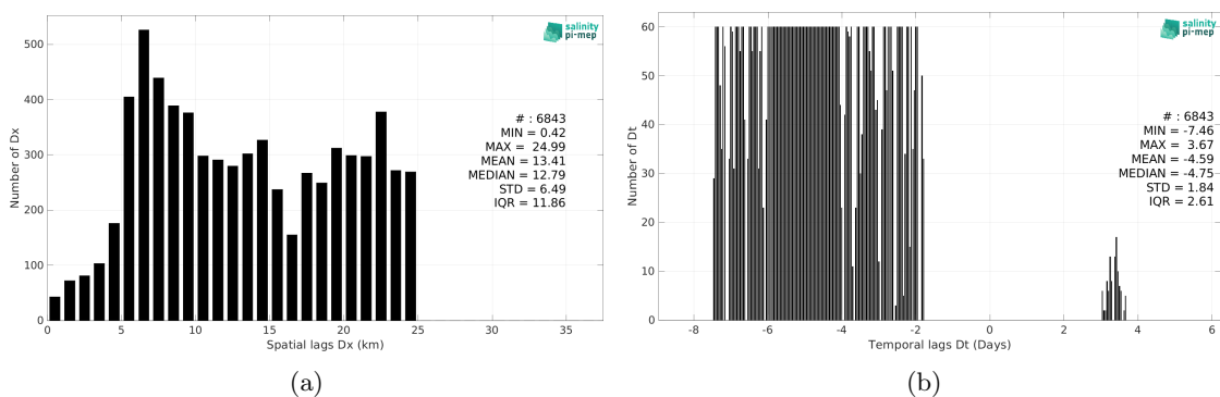
Figure 6: Histograms of the spatial (a) and temporal (b) lags between the location/time of the TSG (GOSUD-Sailing-ship) measurement and the date of the corresponding ISAS SSS pixel.
