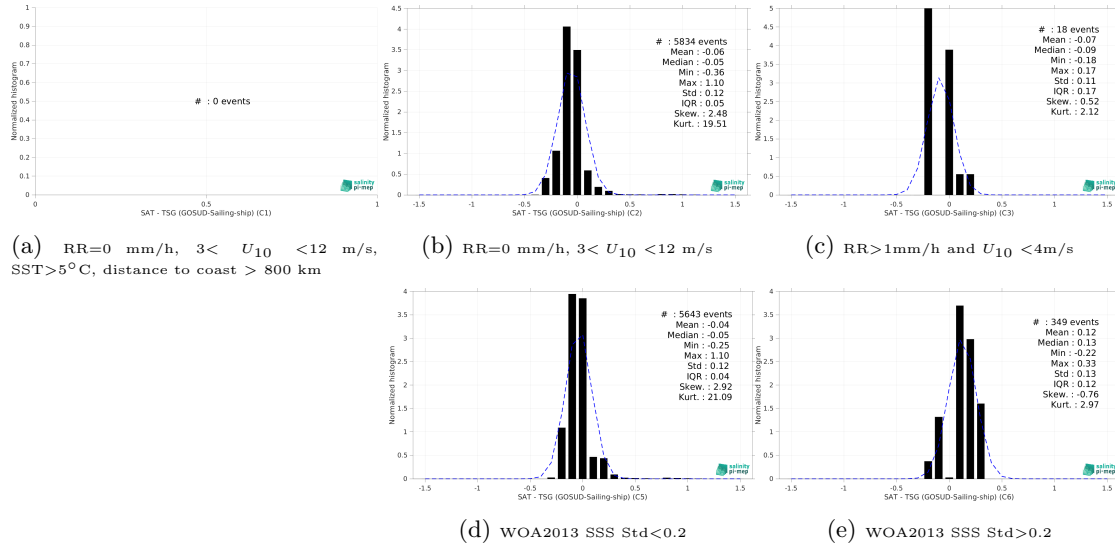
Figure 15: Normalized histogram of \Delta SSS (ISAS - TSG (GOSUD-Sailing-ship)) for 5 different subdatasets corresponding to: RR=0 mm/h, 3 < U_{10} < 12 m/s, SST > 5°C, distance to coast > 800 km (a), RR=0 mm/h, 3 < U_{10} < 12 m/s (b), RR > 1mm/h and U_{10} < 4 m/s (c), WOA2013 SSS Std < 0.2 (d), WOA2013 SSS Std > 0.2 (e).
