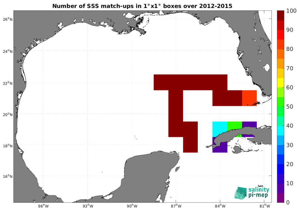
Figure 5: Number of SSS match-ups between TSG (GOSUD-Sailing-ship) SSS and the ISAS SSS product for the Gulf of Mexico Pi-MEP region over 1^\circ \times 1^\circ boxes and for the full satellite product period.
