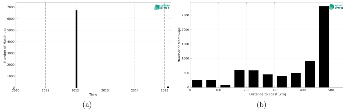
Figure 2: Number of match-ups between TSG (GOSUD-Sailing-ship) and ISAS SSS as a function of time (a) and as function of the distance to coast (b) over the Gulf of Mexico Pi-MEP region and for the full satellite product period.
