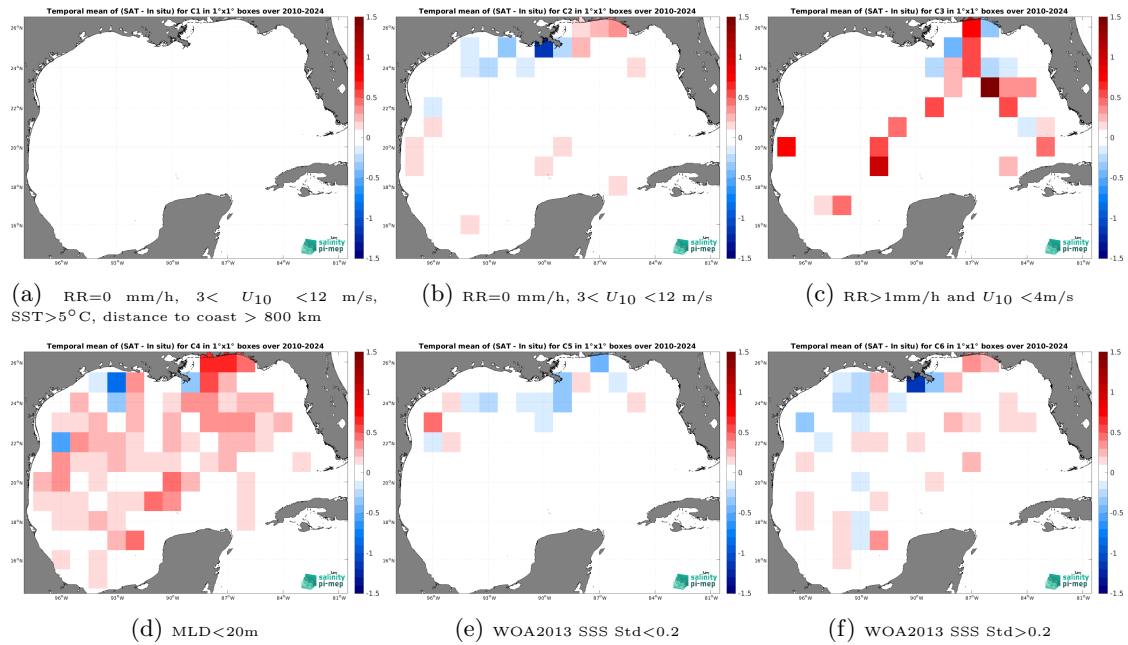
Figure 14: Temporal mean gridded over spatial boxes of size 1^\circ \times 1^\circ of \Delta SSS (ISAS v7 - Monthly (Ifremer-LOPS-CMEMS) - Argo) for 6 different subdatasets corresponding to:RR=0 mm/h, 3 < U_{10} < 12 m/s, SST > 5^\circ\text{C} , distance to coast > 800 km (a), RR=0 mm/h, 3 < U_{10} < 12 m/s (b), RR > 1 mm/h and U_{10} < 4 m/s (c),MLD < 20 m (d),WOA2013 SSS Std < 0.2 (e),WOA2013 SSS Std > 0.2 (f).
