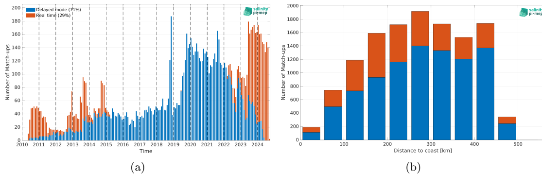
Figure 2: Number of match-ups between Argo and ISAS v7 - Monthly (Ifremer-LOPS-CMEMS) SSS as a function of time (a) and as function of the distance to coast (b) over the Gulf of Mexico Pi-MEP region and for the full satellite product period.
