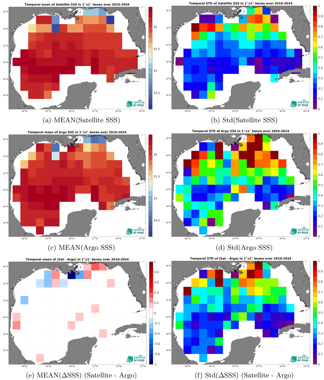
Figure 7: Temporal mean (left) and Std (right) of SSS from ISAS v7 - Monthly (Ifremer-LOPS-CMEMS) (top), Argo (middle), and of \Delta SSS (Satellite - Argo). Only match-up pairs are used to generate these maps.
