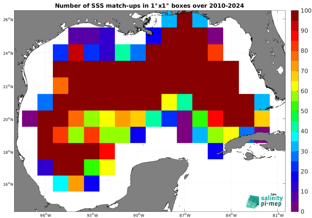
Figure 5: Number of SSS match-ups between Argo SSS and the ISAS v7 - Monthly (Ifremer-LOPS-CMEMS) SSS product for the Gulf of Mexico Pi-MEP region over 1^\circ \times 1^\circ boxes and for the full satellite product period.
