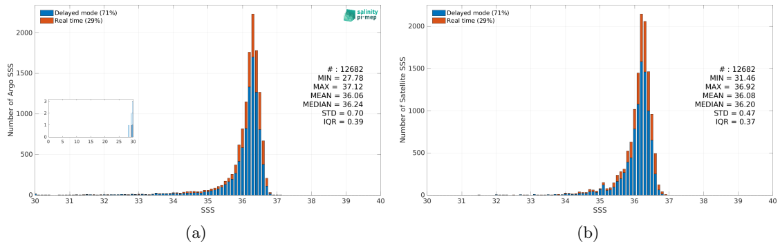
Figure 3: Histograms of SSS from Argo (a) and ISAS v7 - Monthly (Ifremer-LOPS-CMEMS) (b) considering all match-up pairs per bins of 0.1 over the Gulf of Mexico Pi-MEP region and for the full satellite product period.
