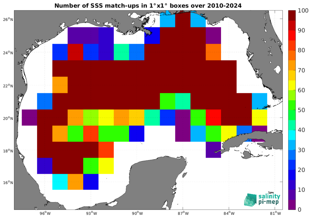
Figure 5: Number of SSS match-ups between Argo SSS and the ISAS SSS product for the Gulf of Mexico Pi-MEP region over 1^\circ \times 1^\circ boxes and for the full satellite product period.
