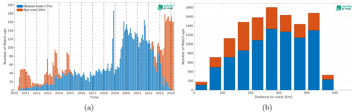
Figure 2: Number of match-ups between Argo and ISAS SSS as a function of time (a) and as a function of the distance to coast (b) over the Gulf of Mexico Pi-MEP region and for the full satellite product period.
