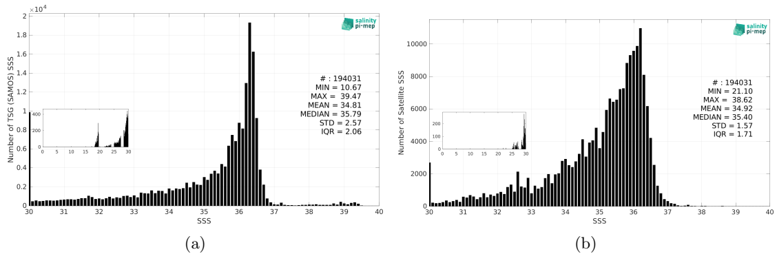
Figure 3: Histograms of SSS from TSG (SAMOS) (a) and CCI SSS L4 Merged-OI v5.5 - 7-day running (ESA) (b) considering all match-up pairs per bins of 0.1 over the Gulf of Mexico Pi-MEP region and for the full satellite product period.
