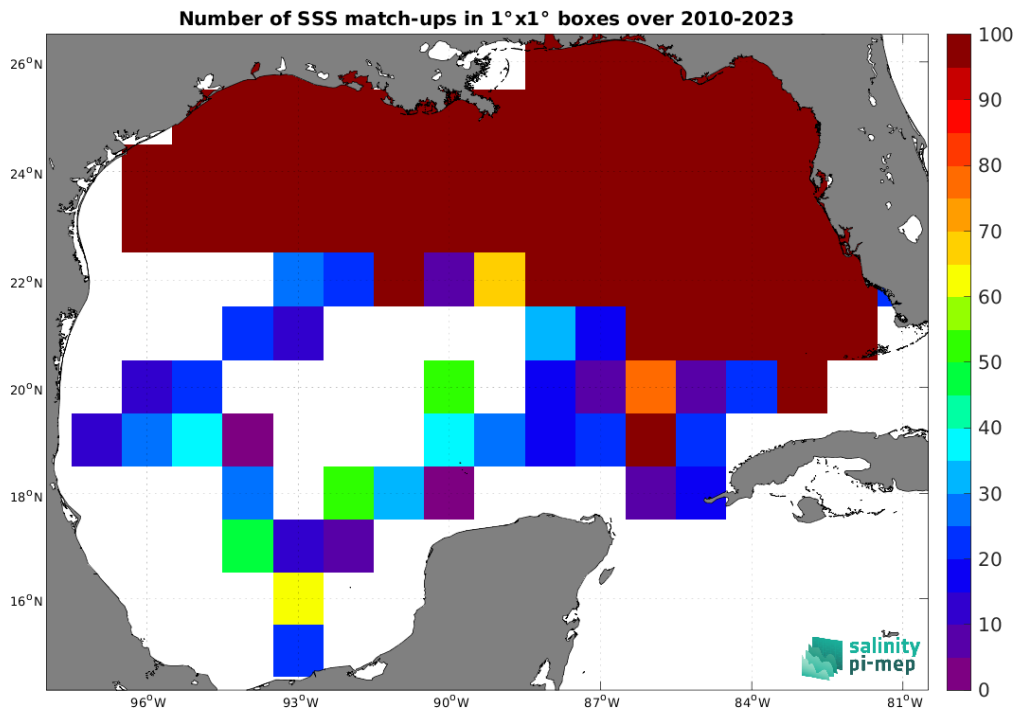
Figure 5: Number of SSS match-ups between TSG (SAMOS) SSS and the CCI SSS L4 Merged-OI v5.5 - 7-day running (ESA) SSS product for the Gulf of Mexico Pi-MEP region over 1^{\circ} \times 1^{\circ} boxes and for the full satellite product period.
