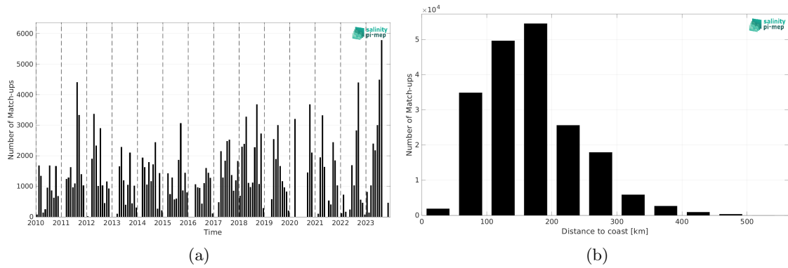
Figure 2: Number of match-ups between TSG (SAMOS) and CCI SSS L4 Merged-OI v5.5 - 7-day running (ESA) SSS as a function of time (a) and as function of the distance to coast (b) over the Gulf of Mexico Pi-MEP region and for the full satellite product period.
