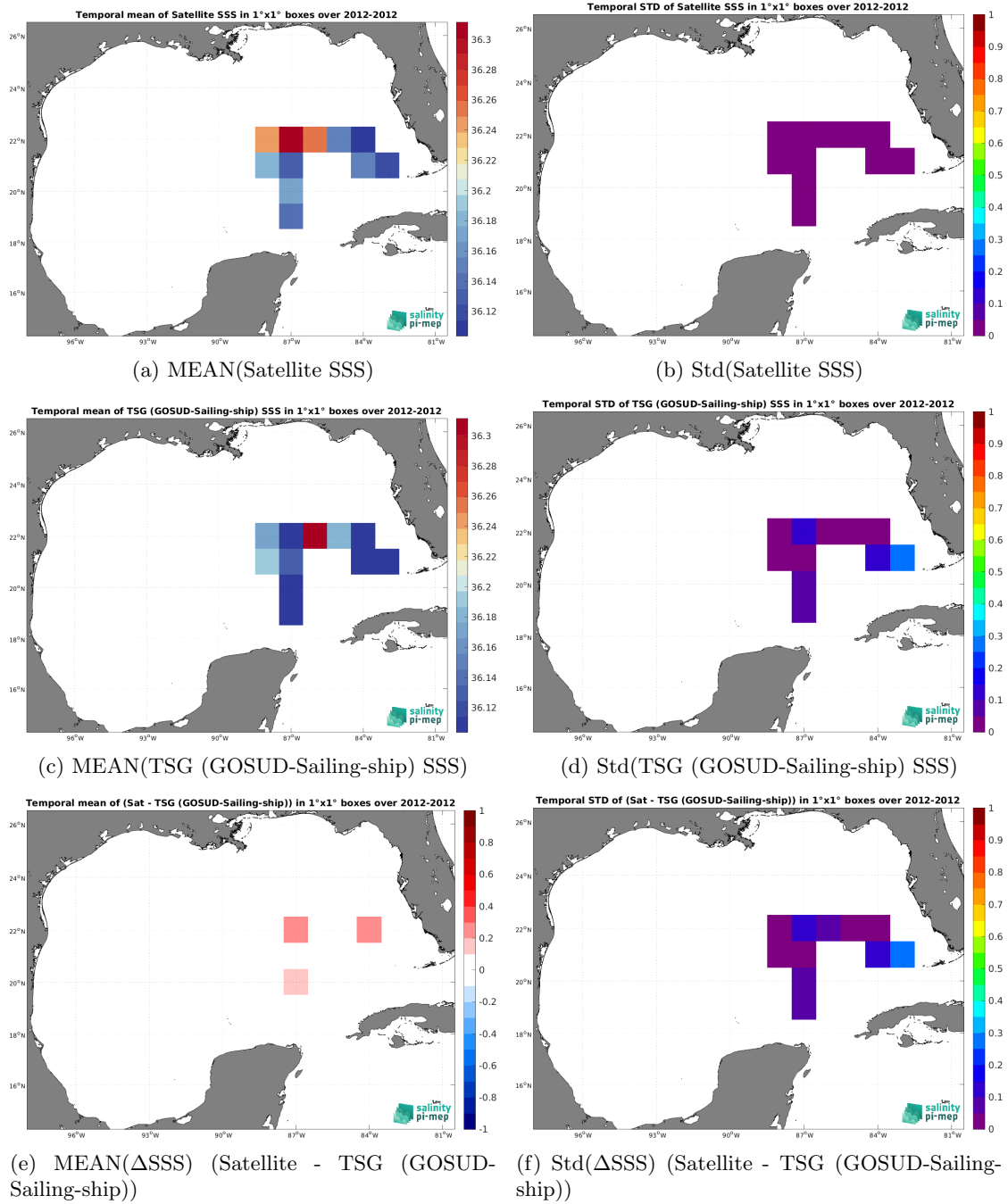
Figure 7: Temporal mean (left) and Std (right) of SSS from CCI SSS L4 Merged-OI v5.5 - 7-day running (ESA) (top), TSG (GOSUD-Sailing-ship) (middle), and of \Delta SSS (Satellite - TSG (GOSUD-Sailing-ship)). Only match-up pairs are used to generate these maps.
