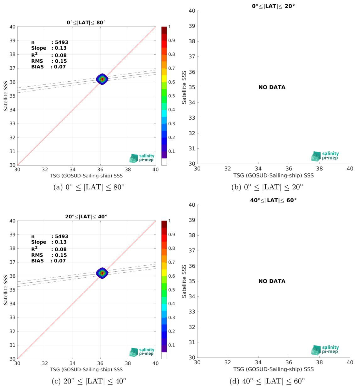
Figure 10: Contour maps of the concentration of CCI SSS L4 Merged-OI v5.5 - 7-day running (ESA) SSS (y-axis) versus TSG (GOSUD-Sailing-ship) SSS (x-axis) at match-up pairs for different latitude bands. For each plot, the red line shows x=y . The black thin and dashed lines indicate a linear fit through the data cloud and the \pm 95\% confidence levels, respectively. The number match-up pairs n , the slope and R^2 coefficient of the linear fit, the root mean square (RMS) and the mean bias between satellite and in situ data are indicated for each latitude band in each plots.
