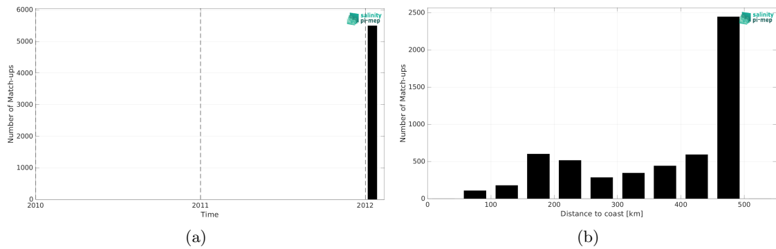
Figure 2: Number of match-ups between TSG (GOSUD-Sailing-ship) and CCI SSS L4 Merged-OI v5.5 - 7-day running (ESA) SSS as a function of time (a) and as function of the distance to coast (b) over the Gulf of Mexico Pi-MEP region and for the full satellite product period.
