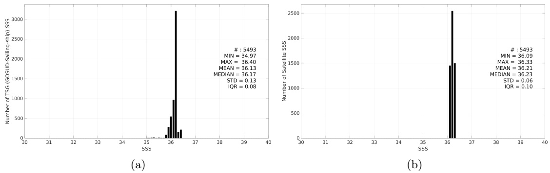
Figure 3: Histograms of SSS from TSG (GOSUD-Sailing-ship) (a) and CCI SSS L4 Merged-OI v5.5 - 7-day running (ESA) (b) considering all match-up pairs per bins of 0.1 over the Gulf of Mexico Pi-MEP region and for the full satellite product period.
