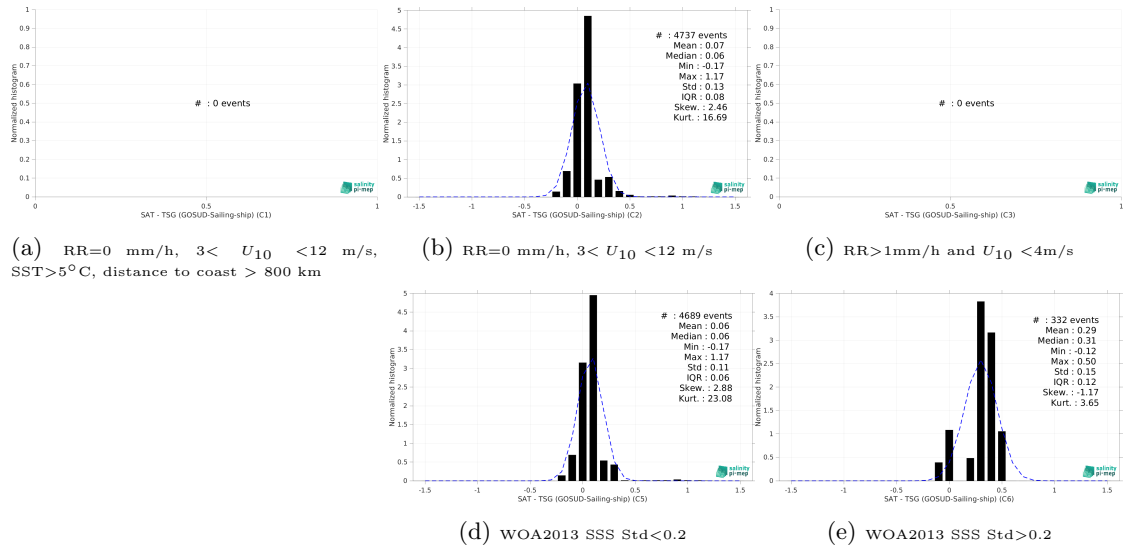
Figure 15: Normalized histogram of \Delta SSS (CCI SSS L4 Merged-OI v5.5 - 7-day running (ESA) - TSG (GOSUD-Sailing-ship)) for 5 different subdatasets corresponding to: RR=0 mm/h, 3 < U_{10} < 12 m/s, SST > 5°C, distance to coast > 800 km (a), RR=0 mm/h, 3 < U_{10} < 12 m/s (b), RR > 1mm/h and U_{10} < 4 m/s (c), WOA2013 SSS Std < 0.2 (d), WOA2013 SSS Std > 0.2 (e).
