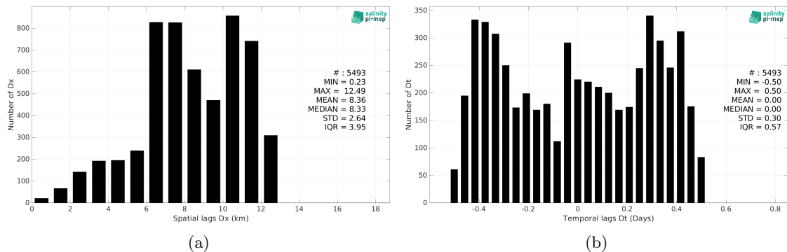
Figure 6: Histograms of the spatial (a) and temporal (b) lags between the location/time of the TSG (GOSUD-Sailing-ship) measurement and the date of the corresponding CCI SSS L4 Merged-OI v5.5 - 7-day running (ESA) SSS pixel.
