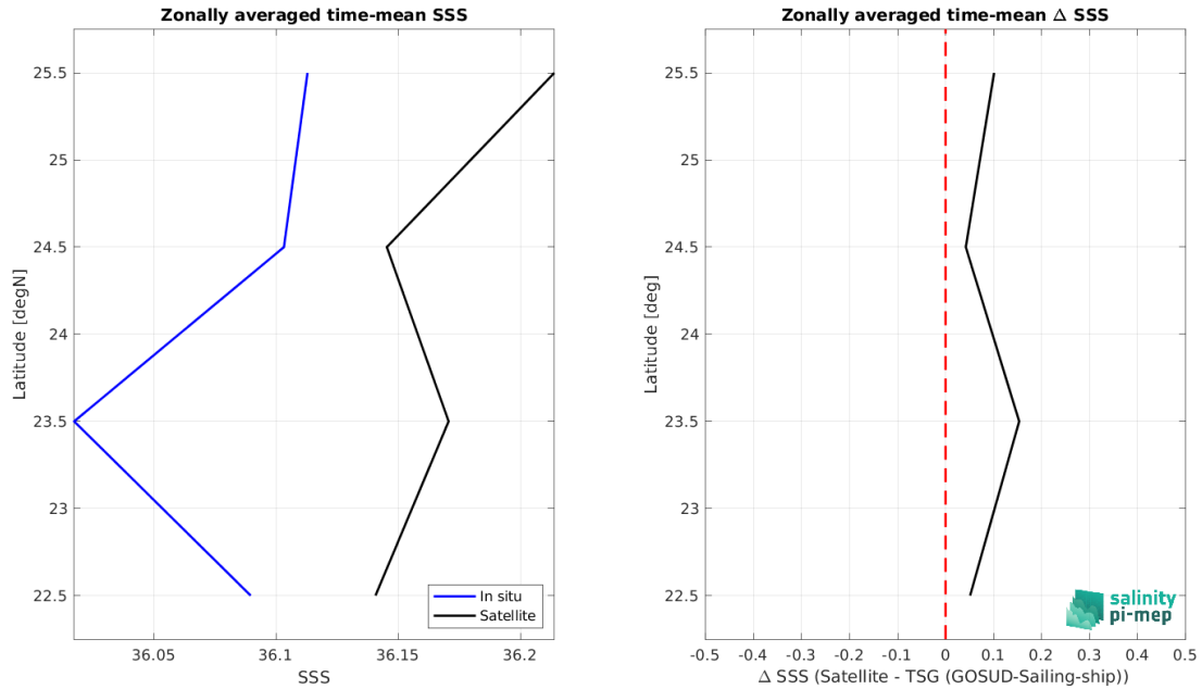
Figure 9: Left panel: Zonal mean SSS from CCI SSS L4 Merged-OI v5.5 - 7-day running (ESA) satellite product (black) and from TSG (GOSUD-Sailing-ship) (blue). Right panel: Zonal mean of \Delta SSS (Satellite - TSG (GOSUD-Sailing-ship)) for all the collected Pi-MEP match-up pairs estimated over the full satellite product period.
