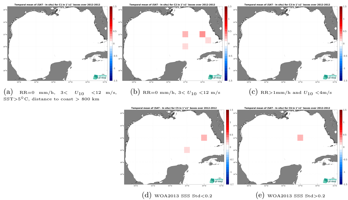
Figure 14: Temporal mean gridded over spatial boxes of size 1^\circ \times 1^\circ of \Delta\text{SSS} (CCI SSS L4 Merged-OI v5.5 - 7-day running (ESA) - TSG (GOSUD-Sailing-ship)) for 5 different subdatasets corresponding to:RR=0 mm/h, 3 < U_{10} < 12 m/s, SST >5^\circ\text{C} , distance to coast > 800 km (a), RR=0 mm/h, 3 < U_{10} < 12 m/s (b), RR >1 mm/h and U_{10} < 4 m/s (c), WOA2013 SSS Std <0.2 (d), WOA2013 SSS Std >0.2 (e).
