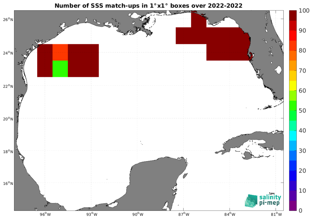
Figure 5: Number of SSS match-ups between Saildrone SSS and the CCI SSS L4 Merged-OI v5.5 - 7-day running (ESA) SSS product for the Gulf of Mexico Pi-MEP region over 1^\circ \times 1^\circ boxes and for the full satellite product period.
