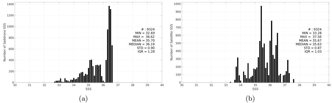
Figure 3: Histograms of SSS from Saildrone (a) and CCI SSS L4 Merged-OI v5.5 - 7-day running (ESA) (b) considering all match-up pairs per bins of 0.1 over the Gulf of Mexico Pi-MEP region and for the full satellite product period.
