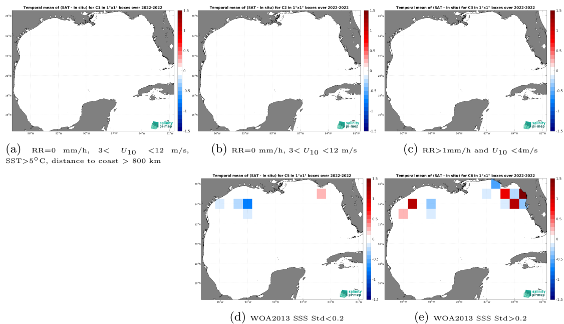
Figure 14: Temporal mean gridded over spatial boxes of size 1^\circ \times 1^\circ of \Delta SSS (CCI SSS L4 Merged-OI v5.5 - 7-day running (ESA) - Saildrone) for 5 different subdatasets corresponding to:RR=0 mm/h, 3 < U_{10} < 12 m/s, SST >5^\circ C, distance to coast > 800 km (a), RR=0 mm/h, 3 < U_{10} < 12 m/s (b), RR >1 mm/h and U_{10} < 4 m/s (c), WOA2013 SSS Std <0.2 (d), WOA2013 SSS Std >0.2 (e).
