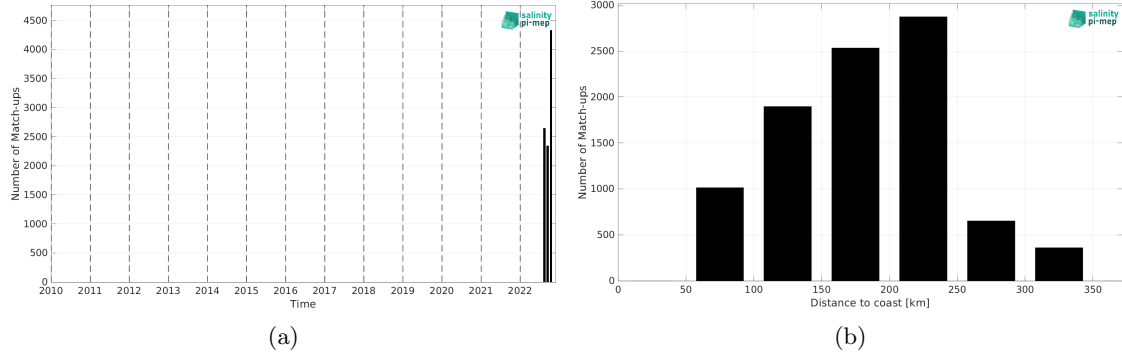
Figure 2: Number of match-ups between Saildrone and CCI SSS L4 Merged-OI v5.5 - 7-day running (ESA) SSS as a function of time (a) and as function of the distance to coast (b) over the Gulf of Mexico Pi-MEP region and for the full satellite product period.
