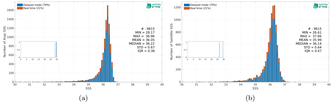
Figure 3: Histograms of SSS from Argo (a) and CCI SSS L4 Merged-OI v5.5 - 7-day running (ESA) (b) considering all match-up pairs per bins of 0.1 over the Gulf of Mexico Pi-MEP region and for the full satellite product period.
