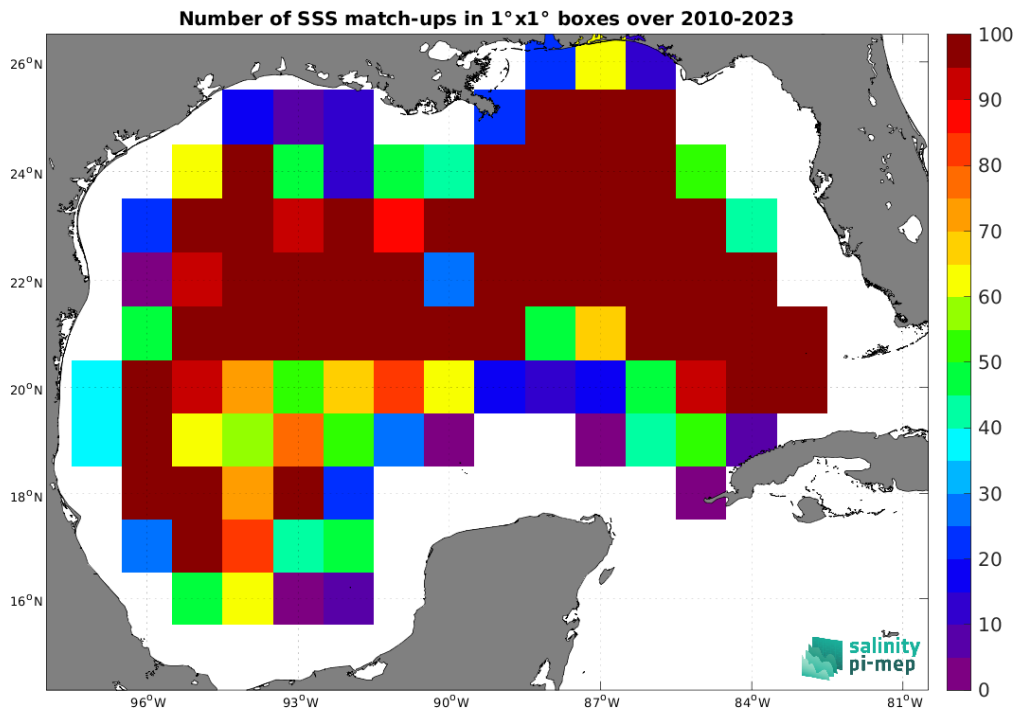
Figure 5: Number of SSS match-ups between Argo SSS and the CCI SSS L4 Merged-OI v5.5 - 7-day running (ESA) SSS product for the Gulf of Mexico Pi-MEP region over 1^\circ \times 1^\circ boxes and for the full satellite product period.
