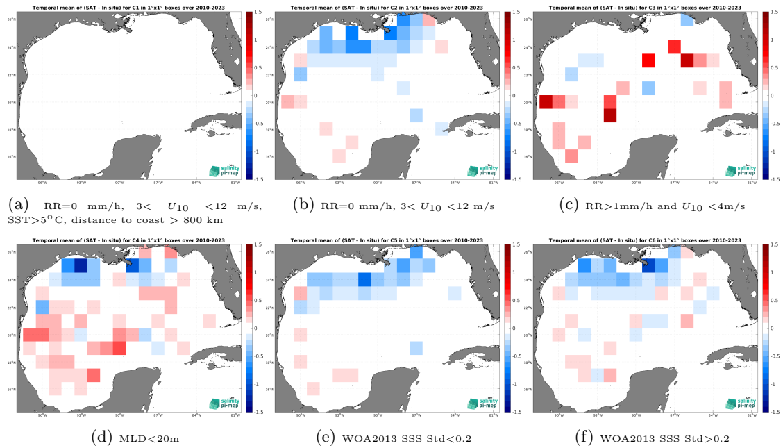
Figure 14: Temporal mean gridded over spatial boxes of size 1^\circ \times 1^\circ of \Delta SSS (CCI SSS L4 Merged-OI v5.5 - 7-day running (ESA) - Argo) for 6 different subdatasets corresponding to:RR=0 mm/h, 3 < U_{10} < 12 m/s, SST >5^\circ C, distance to coast > 800 km (a), RR=0 mm/h, 3 < U_{10} < 12 m/s (b), RR >1 mm/h and U_{10} < 4 m/s (c),MLD <20 m (d),WOA2013 SSS Std <0.2 (e),WOA2013 SSS Std >0.2 (f).
