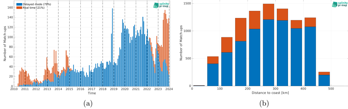
Figure 2: Number of match-ups between Argo and CCI SSS L4 Merged-OI v5.5 - 7-day running (ESA) SSS as a function of time (a) and as function of the distance to coast (b) over the Gulf of Mexico Pi-MEP region and for the full satellite product period.
