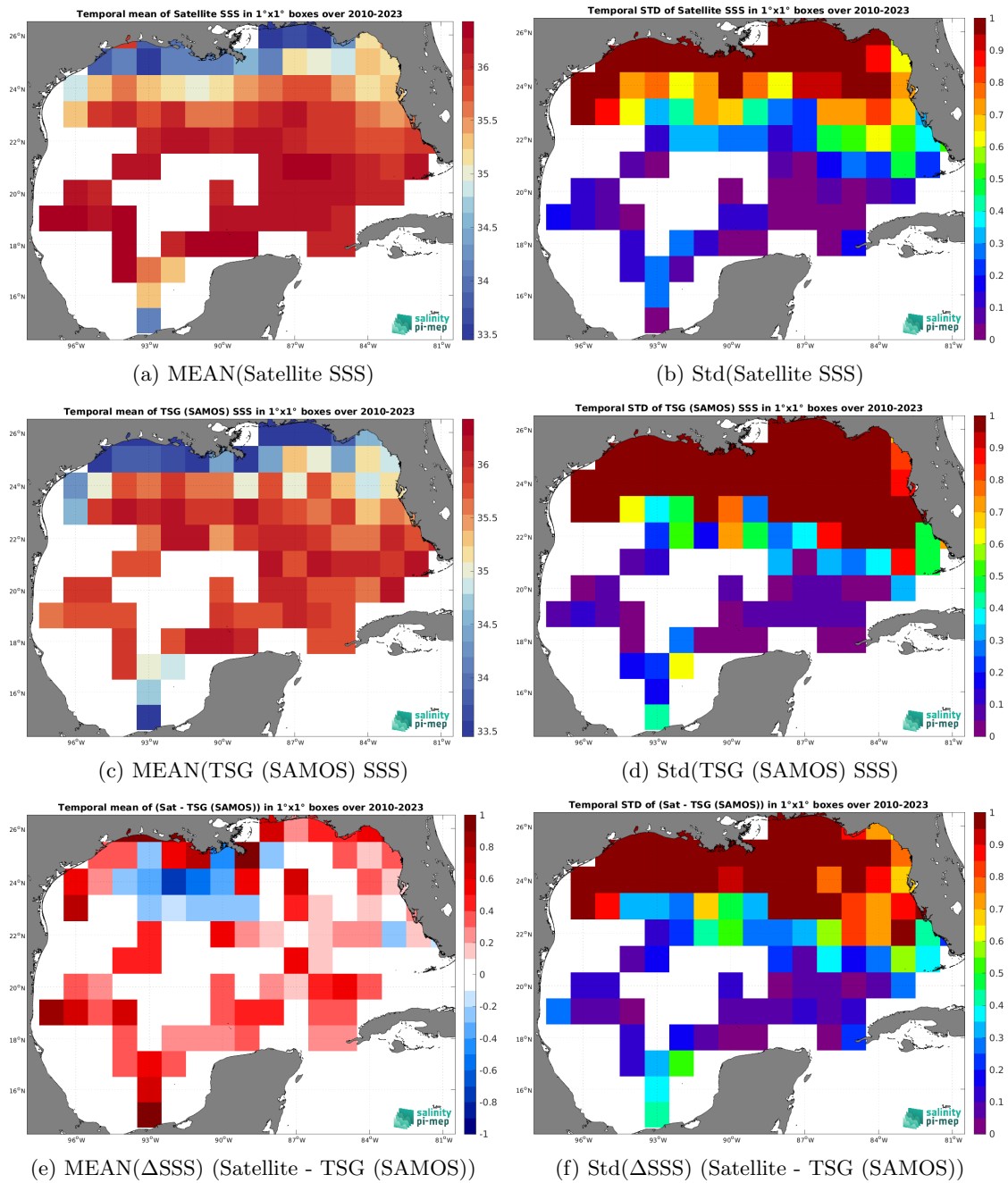
Figure 7: Temporal mean (left) and Std (right) of SSS from CCI SSS L4 Merged-OI v5.5 - 30-day running (ESA) (top), TSG (SAMOS) (middle), and of \Delta SSS (Satellite - TSG (SAMOS)). Only match-up pairs are used to generate these maps.
