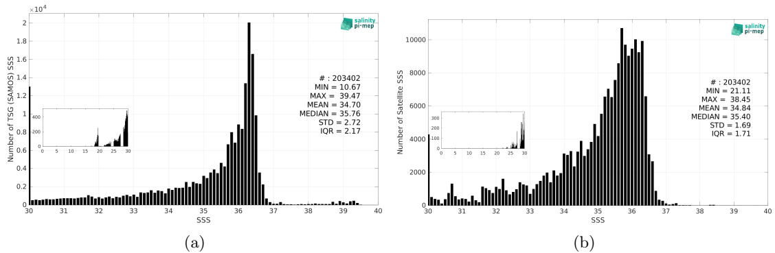
Figure 3: Histograms of SSS from TSG (SAMOS) (a) and CCI SSS L4 Merged-OI v5.5 - 30-day running (ESA) (b) considering all match-up pairs per bins of 0.1 over the Gulf of Mexico Pi-MEP region and for the full satellite product period.
