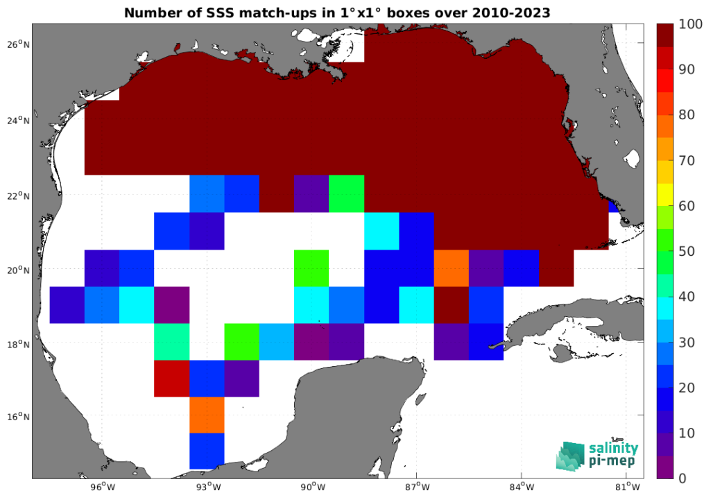
Figure 5: Number of SSS match-ups between TSG (SAMOS) SSS and the CCI SSS L4 Merged-OI v5.5 - 30-day running (ESA) SSS product for the Gulf of Mexico Pi-MEP region over 1°×1° boxes and for the full satellite product period.
