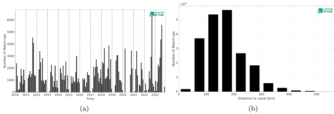
Figure 2: Number of match-ups between TSG (SAMOS) and CCI SSS L4 Merged-OI v5.5 - 30-day running (ESA) SSS as a function of time (a) and as function of the distance to coast (b) over the Gulf of Mexico Pi-MEP region and for the full satellite product period.
