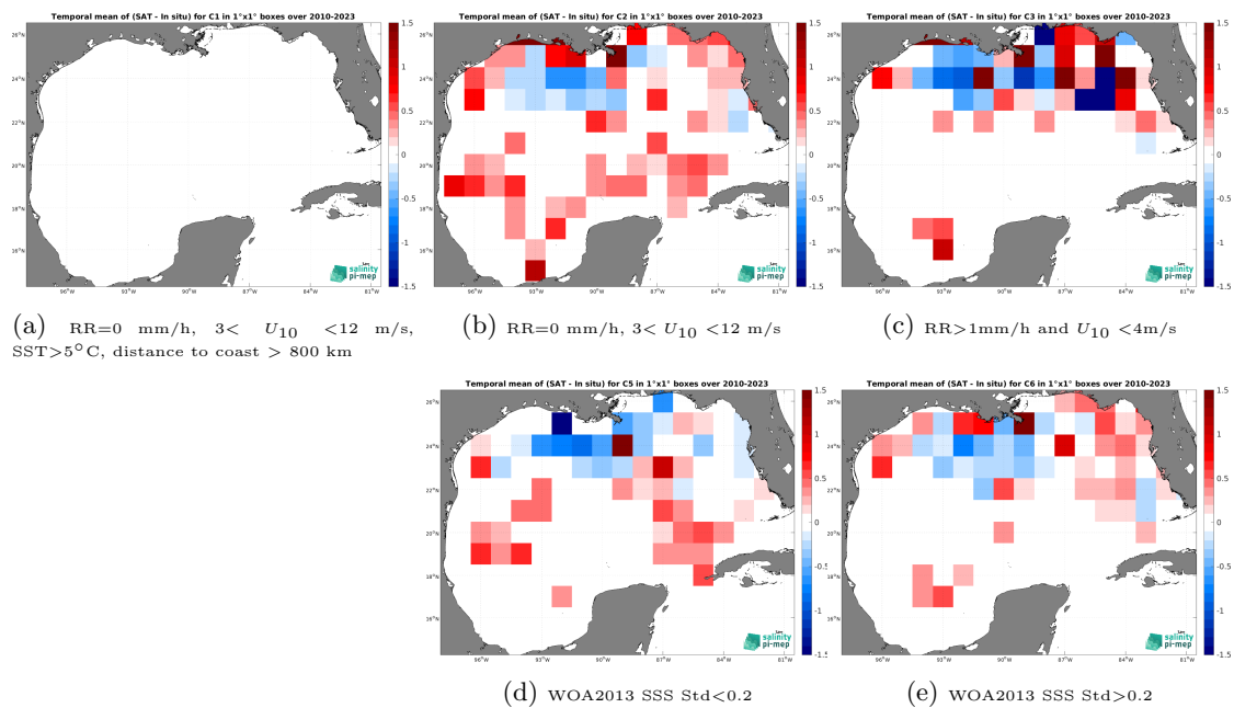
Figure 14: Temporal mean gridded over spatial boxes of size 1^\circ \times 1^\circ of \Delta SSS (CCI SSS L4 Merged-OI v5.5 - 30-day running (ESA) - TSG (SAMOS)) for 5 different subdatasets corresponding to:RR=0 mm/h, 3 < U_{10} < 12 m/s, SST >5^\circ C, distance to coast > 800 km (a), RR=0 mm/h, 3 < U_{10} < 12 m/s (b), RR >1 mm/h and U_{10} < 4 m/s (c), WOA2013 SSS Std <0.2 (d), WOA2013 SSS Std >0.2 (e).
