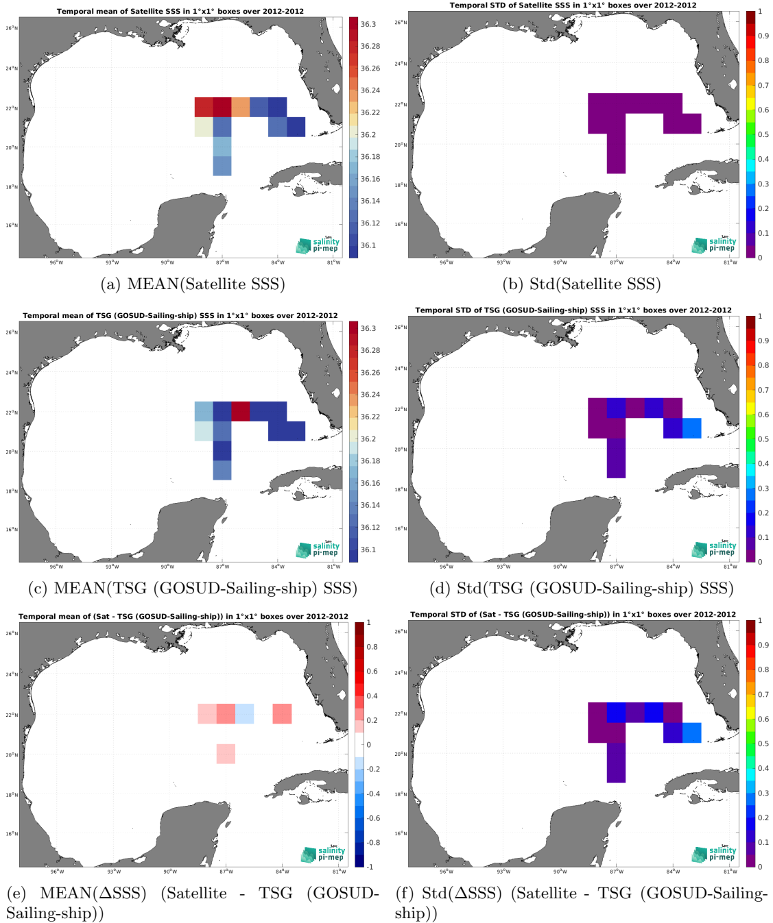
Figure 7: Temporal mean (left) and Std (right) of SSS from CCI SSS L4 Merged-OI v5.5 - 30-day running (ESA) (top), TSG (GOSUD-Sailing-ship) (middle), and of \Delta SSS (Satellite - TSG (GOSUD-Sailing-ship)). Only match-up pairs are used to generate these maps.
