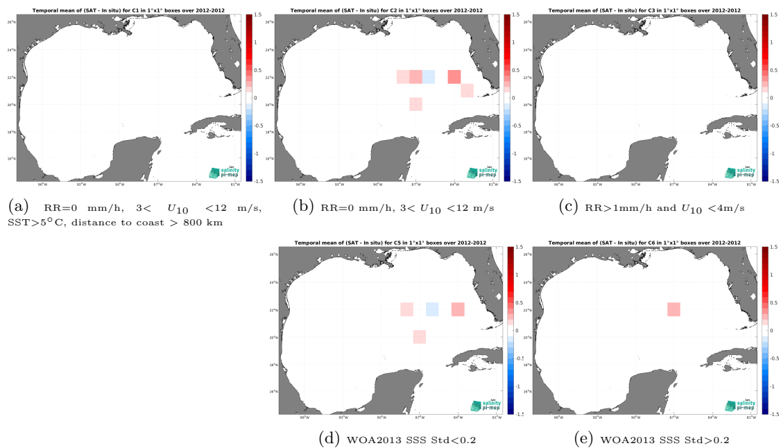
Figure 14: Temporal mean gridded over spatial boxes of size 1^\circ \times 1^\circ of \Delta\text{SSS} (CCI SSS L4 Merged-OI v5.5 - 30-day running (ESA) - TSG (GOSUD-Sailing-ship)) for 5 different subdatasets corresponding to:RR=0 mm/h, 3 < U_{10} < 12 m/s, SST >5^\circ\text{C} , distance to coast > 800 km (a), RR=0 mm/h, 3 < U_{10} < 12 m/s (b), RR >1 mm/h and U_{10} < 4 m/s (c), WOA2013 SSS Std <0.2 (d), WOA2013 SSS Std >0.2 (e).
