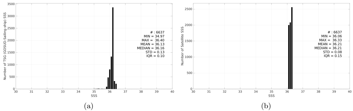
Figure 3: Histograms of SSS from TSG (GOSUD-Sailing-ship) (a) and CCI SSS L4 Merged-OI v5.5 - 30-day running (ESA) (b) considering all match-up pairs per bins of 0.1 over the Gulf of Mexico Pi-MEP region and for the full satellite product period.
