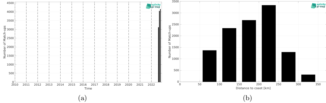
Figure 2: Number of match-ups between Saildrone and CCI SSS L4 Merged-OI v5.5 - 30-day running (ESA) SSS as a function of time (a) and as function of the distance to coast (b) over the Gulf of Mexico Pi-MEP region and for the full satellite product period.
