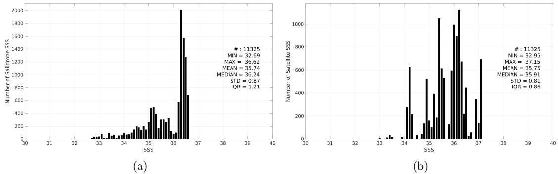
Figure 3: Histograms of SSS from Saildrone (a) and CCI SSS L4 Merged-OI v5.5 - 30-day running (ESA) (b) considering all match-up pairs per bins of 0.1 over the Gulf of Mexico Pi-MEP region and for the full satellite product period.
