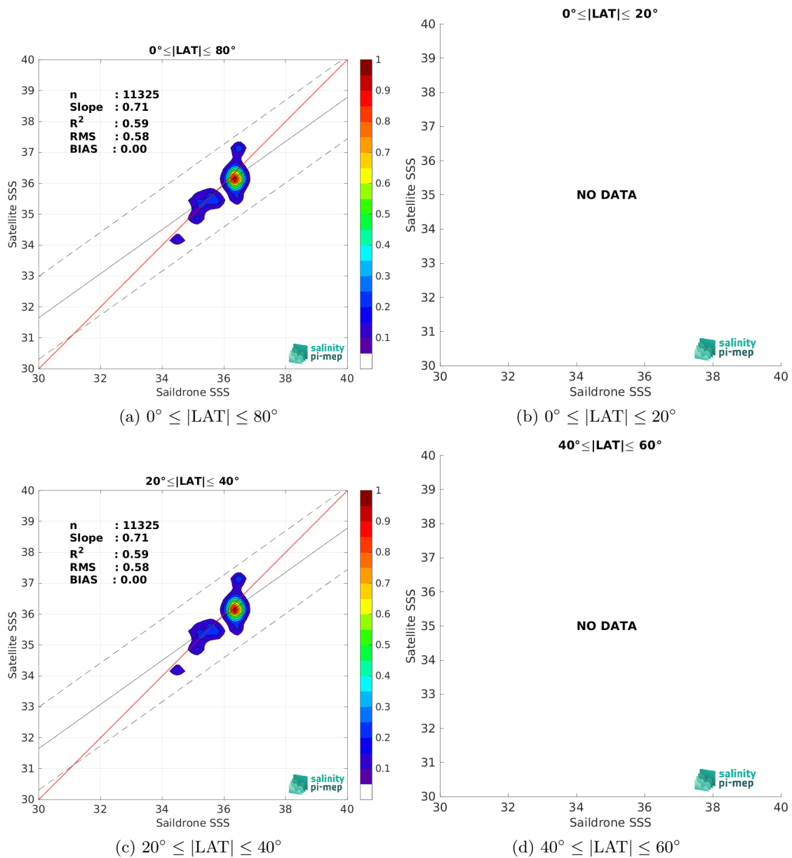
Figure 10: Contour maps of the concentration of CCI SSS L4 Merged-OI v5.5 - 30-day running (ESA) SSS (y-axis) versus Saildrone SSS (x-axis) at match-up pairs for different latitude bands. For each plot, the red line shows x=y . The black thin and dashed lines indicate a linear fit through the data cloud and the \pm 95\% confidence levels, respectively. The number match-up pairs n , the slope and R^2 coefficient of the linear fit, the root mean square (RMS) and the mean bias between satellite and in situ data are indicated for each latitude band in each plots.
