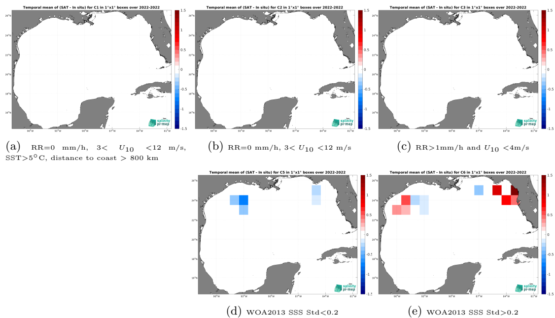
Figure 14: Temporal mean gridded over spatial boxes of size 1^\circ \times 1^\circ of \Delta SSS (CCI SSS L4 Merged-OI v5.5 - 30-day running (ESA) - Saildrone) for 5 different subdatasets corresponding to:RR=0 mm/h, 3 < U_{10} < 12 m/s, SST >5^\circ C, distance to coast > 800 km (a), RR=0 mm/h, 3 < U_{10} < 12 m/s (b), RR >1 mm/h and U_{10} < 4 m/s (c), WOA2013 SSS Std <0.2 (d), WOA2013 SSS Std >0.2 (e).
