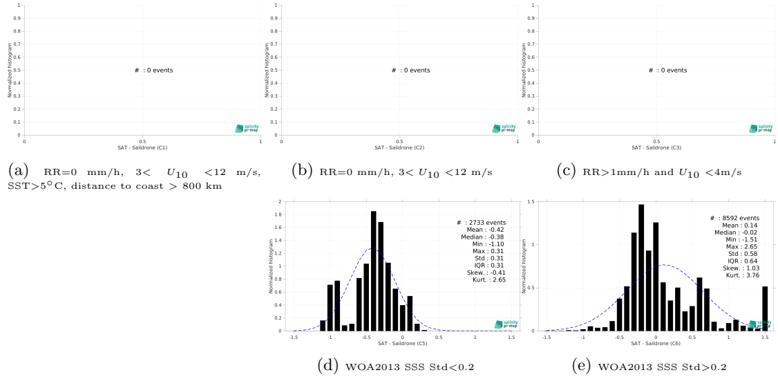
Figure 15: Normalized histogram of \Delta SSS (CCI SSS L4 Merged-OI v5.5 - 30-day running (ESA) - Saildrone) for 5 different subdatasets corresponding to: RR=0 mm/h, 3 < U_{10} < 12 m/s, SST>5°C, distance to coast > 800 km (a), RR=0 mm/h, 3 < U_{10} < 12 m/s (b), RR>1mm/h and U_{10} < 4 m/s (c), WOA2013 SSS Std<0.2 (d), WOA2013 SSS Std>0.2 (e).
