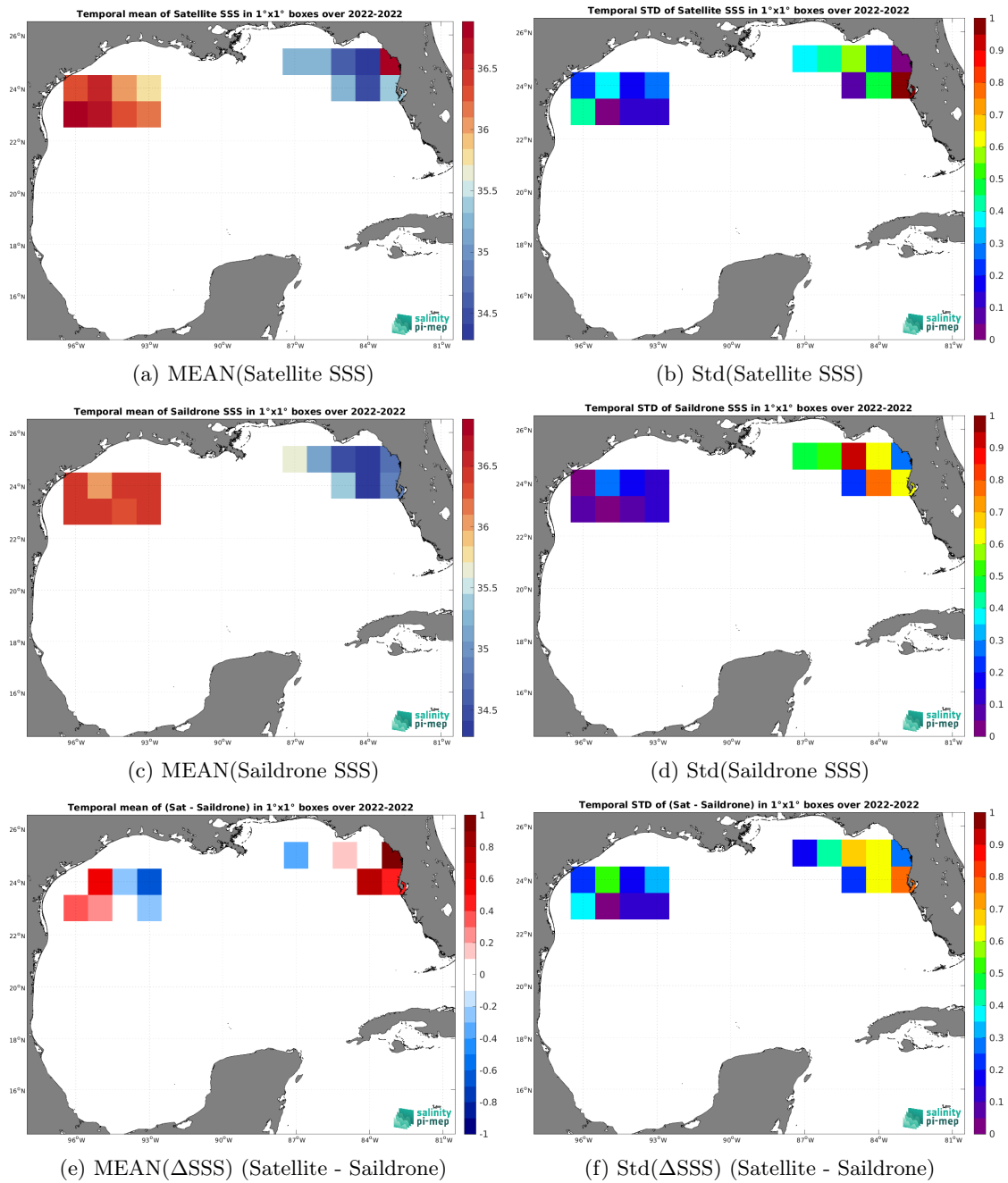
Figure 7: Temporal mean (left) and Std (right) of SSS from CCI SSS L4 Merged-OI v5.5 - 30-day running (ESA) (top), Saildrone (middle), and of \Delta SSS (Satellite - Saildrone). Only match-up pairs are used to generate these maps.
