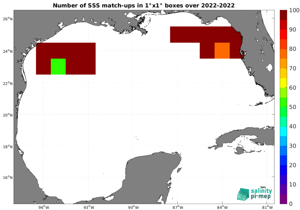
Figure 5: Number of SSS match-ups between Saildrone SSS and the CCI SSS L4 Merged-OI v5.5 - 30-day running (ESA) SSS product for the Gulf of Mexico Pi-MEP region over 1^\circ \times 1^\circ boxes and for the full satellite product period.
