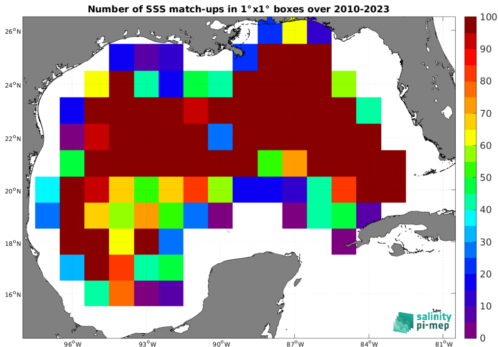
Figure 5: Number of SSS match-ups between Argo SSS and the CCI SSS L4 Merged-OI v5.5 - 30-day running (ESA) SSS product for the Gulf of Mexico Pi-MEP region over 1^\circ \times 1^\circ boxes and for the full satellite product period.
