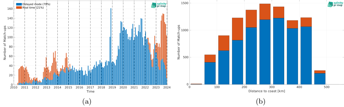
Figure 2: Number of match-ups between Argo and CCI SSS L4 Merged-OI v5.5 - 30-day running (ESA) SSS as a function of time (a) and as function of the distance to coast (b) over the Gulf of Mexico Pi-MEP region and for the full satellite product period.
