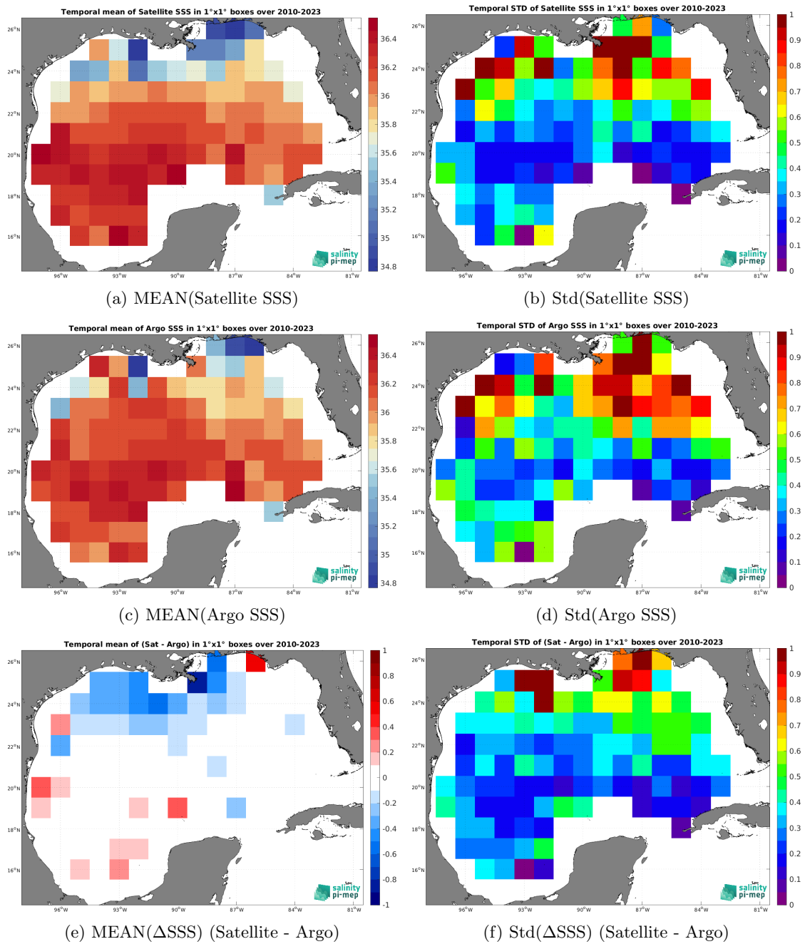
Figure 7: Temporal mean (left) and Std (right) of SSS from CCI SSS L4 Merged-OI v5.5 - 30-day running (ESA) (top), Argo (middle), and of \Delta SSS (Satellite - Argo). Only match-up pairs are used to generate these maps.
