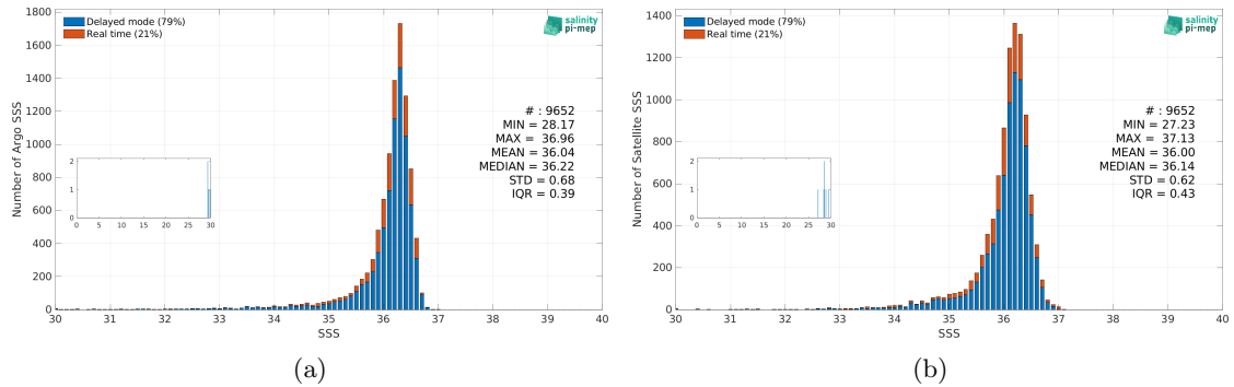
Figure 3: Histograms of SSS from Argo (a) and CCI SSS L4 Merged-OI v5.5 - 30-day running (ESA) (b) considering all match-up pairs per bins of 0.1 over the Gulf of Mexico Pi-MEP region and for the full satellite product period.
