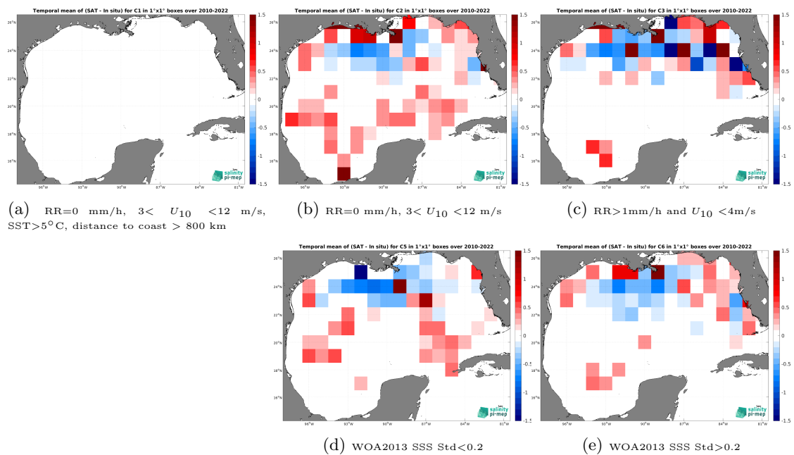
Figure 14: Temporal mean gridded over spatial boxes of size 1^\circ \times 1^\circ of \Delta\text{SSS} (CCI SSS L4 Merged-OI v4.41 - 7-day running (ESA) - TSG (SAMOS)) for 5 different subdatasets corresponding to:RR=0 mm/h, 3 < U_{10} < 12 m/s, SST>5°C, distance to coast > 800 km (a), RR=0 mm/h, 3 < U_{10} < 12 m/s (b), RR>1mm/h and U_{10} < 4 m/s (c), WOA2013 SSS Std<0.2 (d), WOA2013 SSS Std>0.2 (e).
