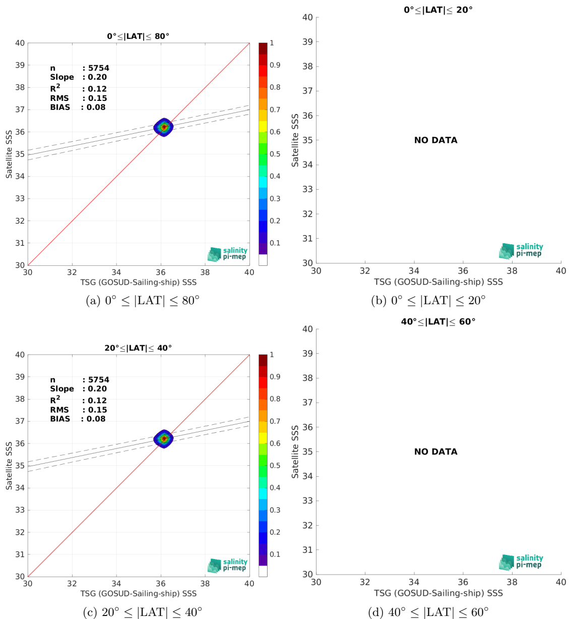
Figure 10: Contour maps of the concentration of CCI SSS L4 Merged-OI v4.41 - 7-day running (ESA) SSS (y-axis) versus TSG (GOSUD-Sailing-ship) SSS (x-axis) at match-up pairs for different latitude bands. For each plot, the red line shows x=y . The black thin and dashed lines indicate a linear fit through the data cloud and the \pm 95\% confidence levels, respectively. The number match-up pairs n , the slope and R^2 coefficient of the linear fit, the root mean square (RMS) and the mean bias between satellite and in situ data are indicated for each latitude band in each plots.
