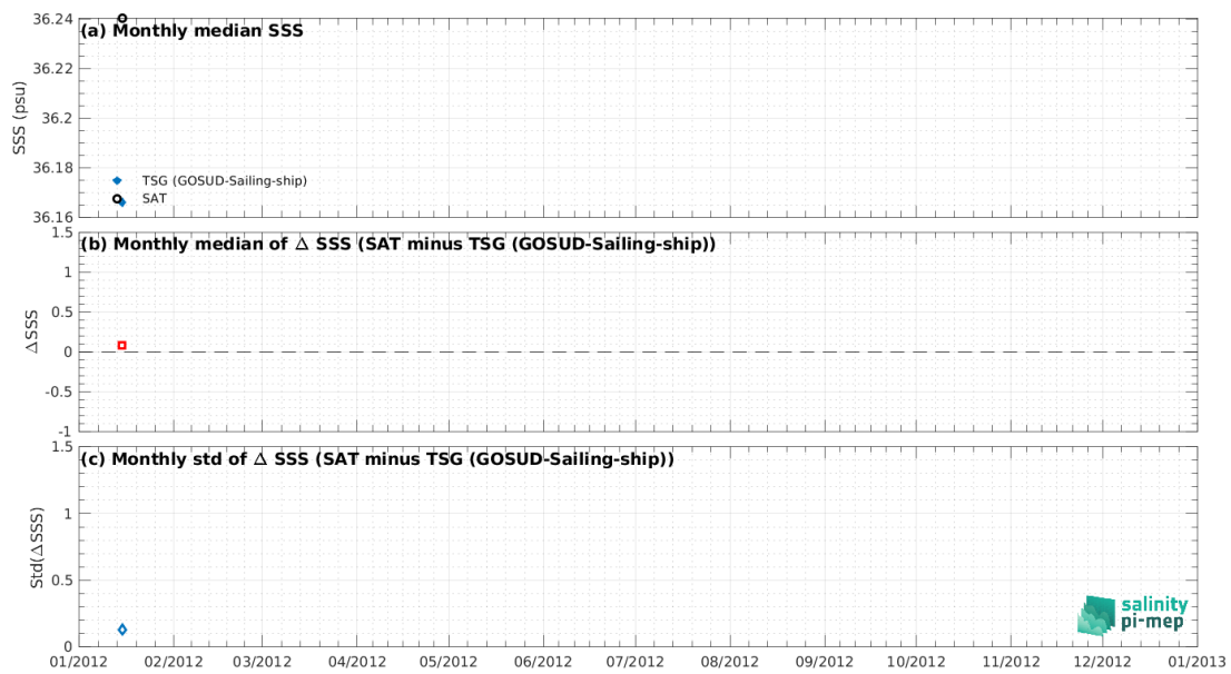
Figure 8: Time series of the monthly median SSS (top), median of \Delta SSS (Satellite - TSG (GOSUD-Sailing-ship)) and Std of \Delta SSS (Satellite - TSG (GOSUD-Sailing-ship)) over the Gulf of Mexico Pi-MEP region considering all match-ups collected by the Pi-MEP.
