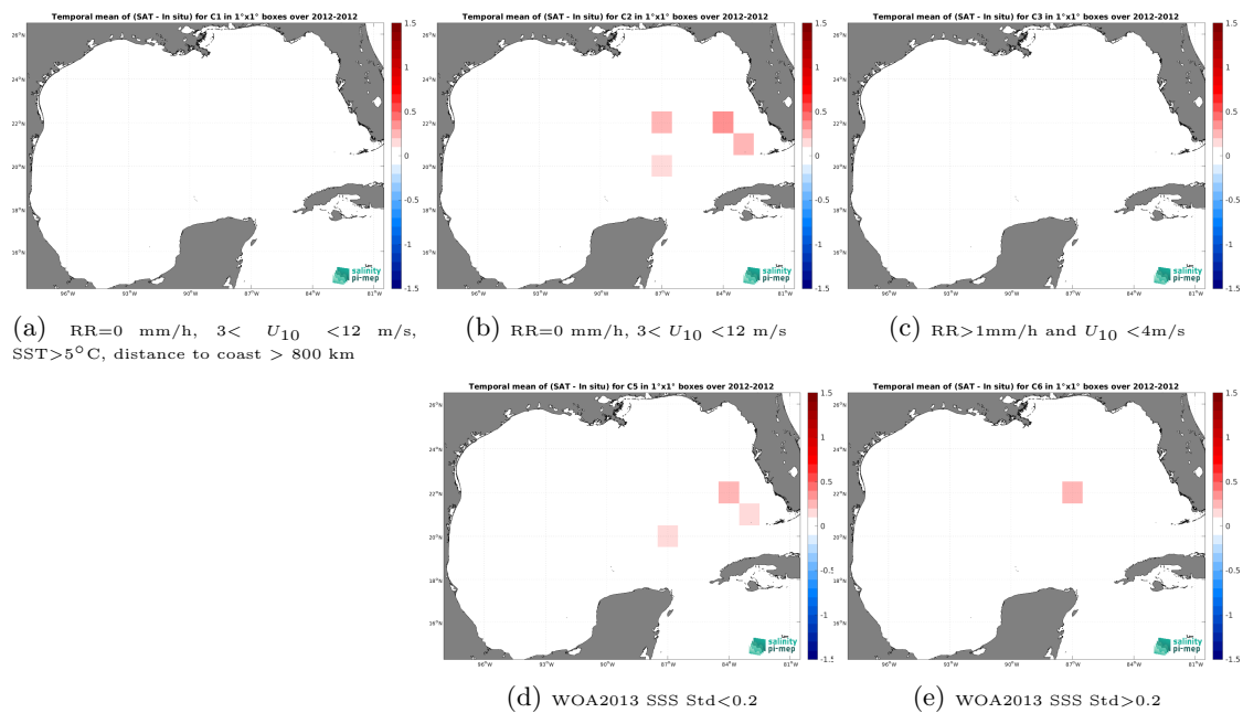
Figure 14: Temporal mean gridded over spatial boxes of size 1^\circ \times 1^\circ of \Delta\text{SSS} (CCI SSS L4 Merged-OI v4.41 - 7-day running (ESA) - TSG (GOSUD-Sailing-ship)) for 5 different subdatasets corresponding to:RR=0 mm/h, 3 < U_{10} < 12 m/s, SST >5^\circ\text{C} , distance to coast > 800 km (a), RR=0 mm/h, 3 < U_{10} < 12 m/s (b), RR >1 mm/h and U_{10} < 4 m/s (c), WOA2013 SSS Std <0.2 (d), WOA2013 SSS Std >0.2 (e).
