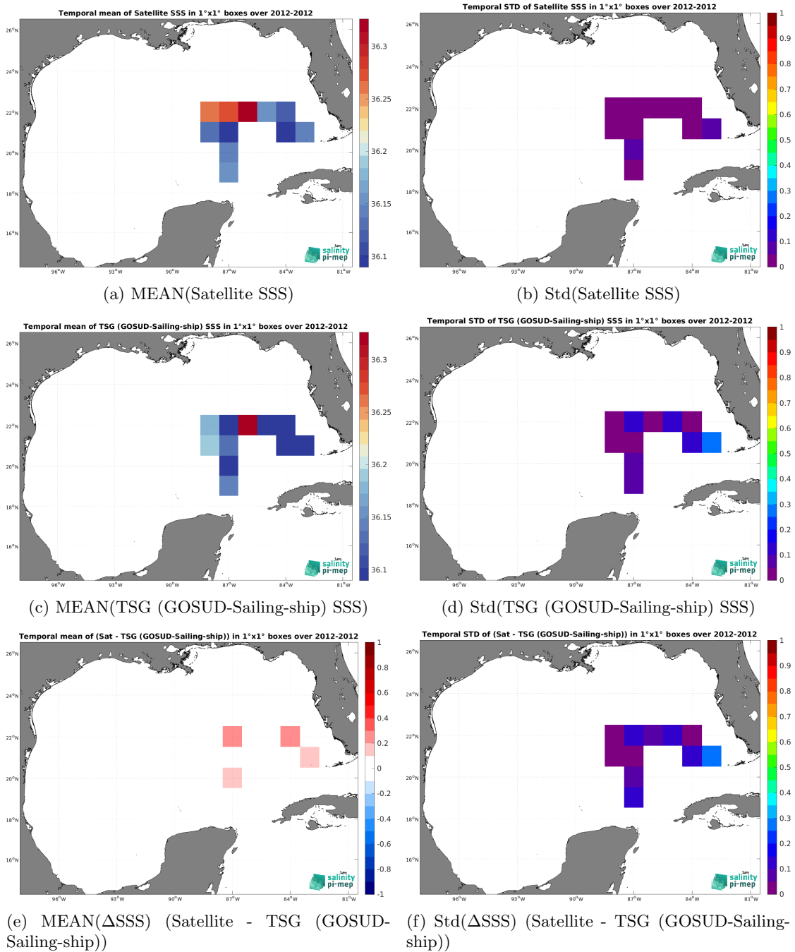
Figure 7: Temporal mean (left) and Std (right) of SSS from CCI SSS L4 Merged-OI v4.41 - 7-day running (ESA) (top), TSG (GOSUD-Sailing-ship) (middle), and of \Delta SSS (Satellite - TSG (GOSUD-Sailing-ship)). Only match-up pairs are used to generate these maps.
