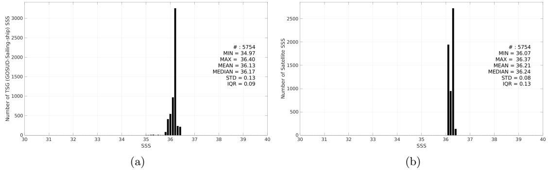
Figure 3: Histograms of SSS from TSG (GOSUD-Sailing-ship) (a) and CCI SSS L4 Merged-OI v4.41 - 7-day running (ESA) (b) considering all match-up pairs per bins of 0.1 over the Gulf of Mexico Pi-MEP region and for the full satellite product period.
