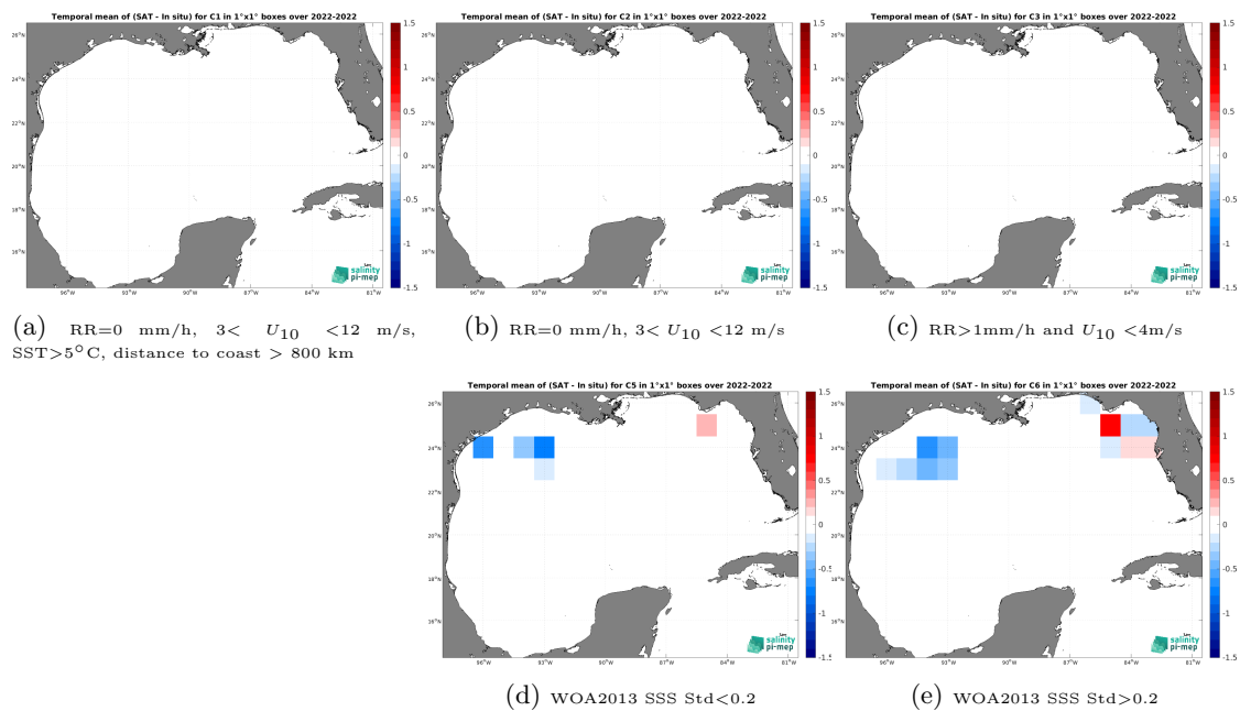
Figure 14: Temporal mean gridded over spatial boxes of size 1^\circ \times 1^\circ of \Delta\text{SSS} (CCI SSS L4 Merged-OI v4.41 - 7-day running (ESA) - Saildrone) for 5 different subdatasets corresponding to:RR=0 mm/h, 3 < U_{10} < 12 m/s, SST>5°C, distance to coast > 800 km (a), RR=0 mm/h, 3 < U_{10} < 12 m/s (b), RR>1mm/h and U_{10} < 4 m/s (c), WOA2013 SSS Std<0.2 (d), WOA2013 SSS Std>0.2 (e).
