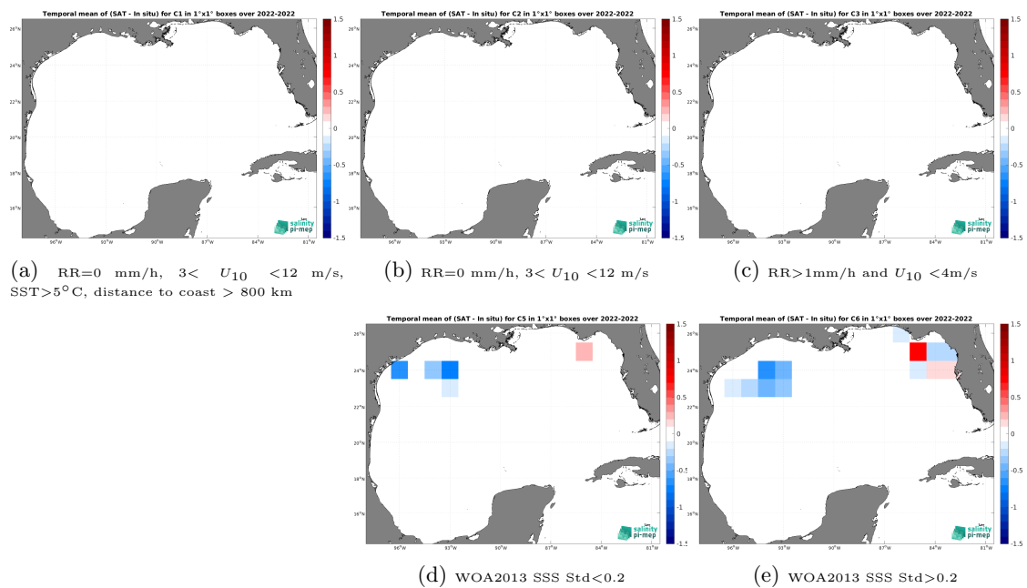
Figure 14: Temporal mean gridded over spatial boxes of size 1^\circ \times 1^\circ of \Delta SSS (CCI SSS L4 Merged-OI v4.41 - 7-day running (ESA) - Saildrone) for 5 different subdatasets corresponding to:RR=0 mm/h, 3 < U_{10} < 12 m/s, SST >5^\circ C, distance to coast > 800 km (a), RR=0 mm/h, 3 < U_{10} < 12 m/s (b), RR >1 mm/h and U_{10} < 4 m/s (c), WOA2013 SSS Std <0.2 (d), WOA2013 SSS Std >0.2 (e).
