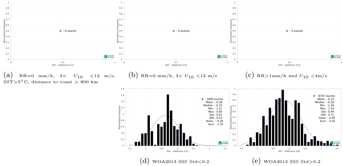
Figure 15: Normalized histogram of \Delta SSS (CCI SSS L4 Merged-OI v4.41 - 7-day running (ESA) - Saildrone) for 5 different subdatasets corresponding to: RR=0 mm/h, 3 < U_{10} < 12 m/s, SST>5°C, distance to coast > 800 km (a), RR=0 mm/h, 3 < U_{10} < 12 m/s (b), RR>1mm/h and U_{10} < 4 m/s (c), WOA2013 SSS Std<0.2 (d), WOA2013 SSS Std>0.2 (e).
