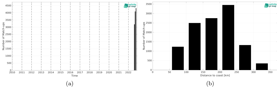
Figure 2: Number of match-ups between Saildrone and CCI SSS L4 Merged-OI v4.41 - 7-day running (ESA) SSS as a function of time (a) and as function of the distance to coast (b) over the Gulf of Mexico Pi-MEP region and for the full satellite product period.
