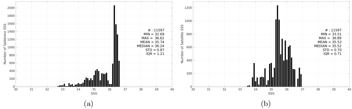
Figure 3: Histograms of SSS from Saildrone (a) and CCI SSS L4 Merged-OI v4.41 - 7-day running (ESA) (b) considering all match-up pairs per bins of 0.1 over the Gulf of Mexico Pi-MEP region and for the full satellite product period.
