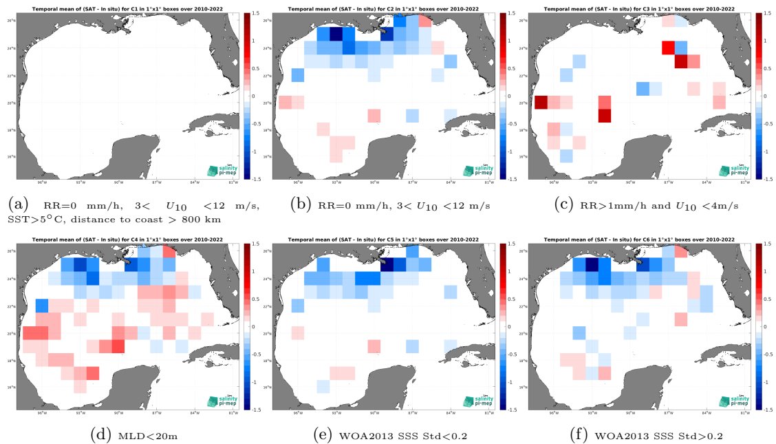
Figure 14: Temporal mean gridded over spatial boxes of size 1^\circ \times 1^\circ of \Delta\text{SSS} (CCI SSS L4 Merged-OI v4.41 - 7-day running (ESA) - Argo) for 6 different subdatasets corresponding to: RR=0 mm/h, 3 < U_{10} < 12 m/s, SST > 5°C, distance to coast > 800 km (a), RR=0 mm/h, 3 < U_{10} < 12 m/s (b), RR > 1mm/h and U_{10} < 4 m/s (c), MLD < 20m (d), WOA2013 SSS Std < 0.2 (e), WOA2013 SSS Std > 0.2 (f).
