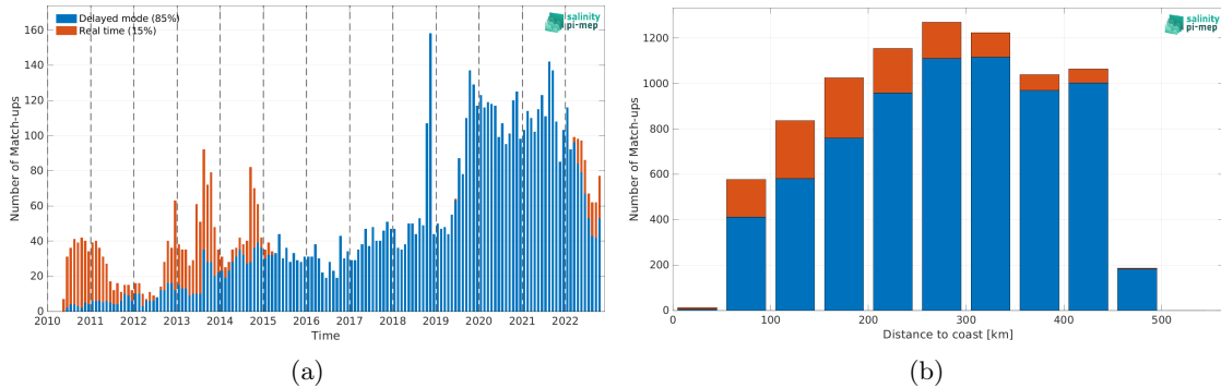
Figure 2: Number of match-ups between Argo and CCI SSS L4 Merged-OI v4.41 - 7-day running (ESA) SSS as a function of time (a) and as function of the distance to coast (b) over the Gulf of Mexico Pi-MEP region and for the full satellite product period.
