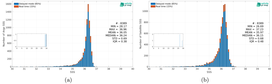
Figure 3: Histograms of SSS from Argo (a) and CCI SSS L4 Merged-OI v4.41 - 7-day running (ESA) (b) considering all match-up pairs per bins of 0.1 over the Gulf of Mexico Pi-MEP region and for the full satellite product period.
