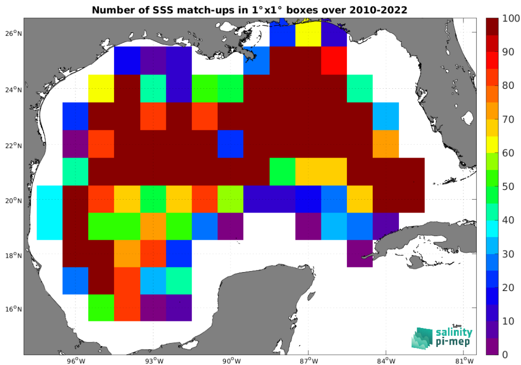
Figure 5: Number of SSS match-ups between Argo SSS and the CCI SSS L4 Merged-OI v4.41 - 7-day running (ESA) SSS product for the Gulf of Mexico Pi-MEP region over 1^\circ \times 1^\circ boxes and for the full satellite product period.
