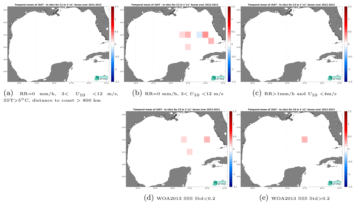
Figure 14: Temporal mean gridded over spatial boxes of size 1^\circ \times 1^\circ of \Delta\text{SSS} (CCI SSS L4 Merged-OI v4.41 - 30-day running (ESA) - TSG (GOSUD-Sailing-ship)) for 5 different subdatasets corresponding to:RR=0 mm/h, 3 < U_{10} < 12 m/s, SST >5^\circ\text{C} , distance to coast > 800 km (a), RR=0 mm/h, 3 < U_{10} < 12 m/s (b), RR >1 mm/h and U_{10} < 4 m/s (c), WOA2013 SSS Std <0.2 (d), WOA2013 SSS Std >0.2 (e).
