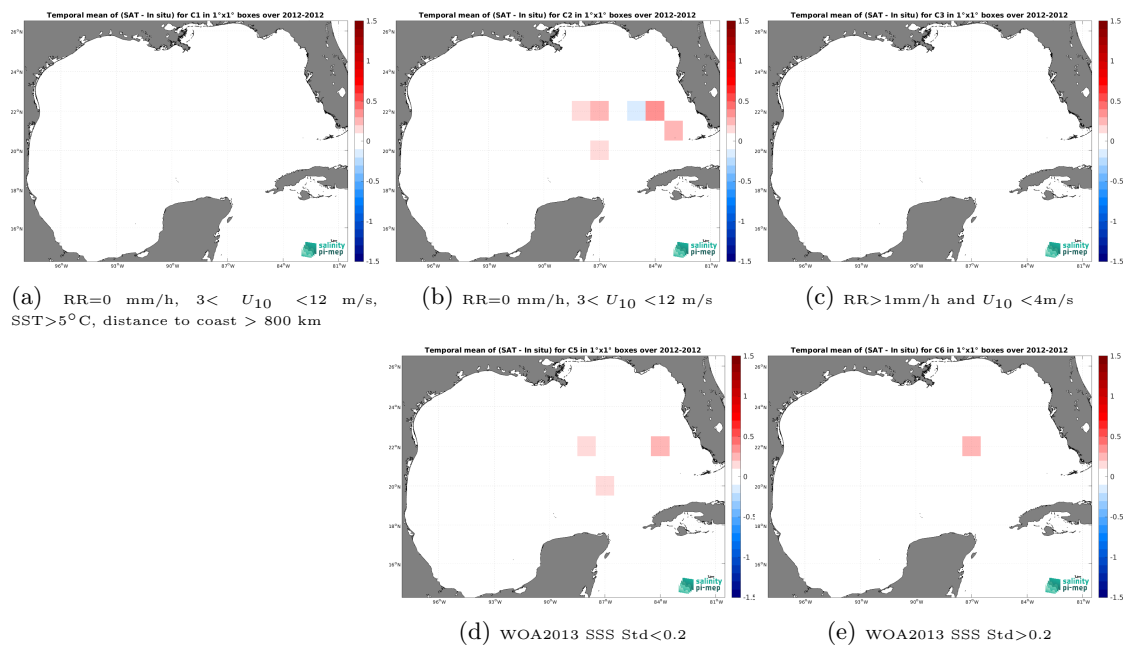
Figure 14: Temporal mean gridded over spatial boxes of size 1^\circ \times 1^\circ of \Delta SSS (CCI SSS L4 Merged-OI v4.41 - 30-day running (ESA) - TSG (GOSUD-Sailing-ship)) for 5 different subdatasets corresponding to:RR=0 mm/h, 3 < U_{10} < 12 m/s, SST >5^\circ C, distance to coast > 800 km (a), RR=0 mm/h, 3 < U_{10} < 12 m/s (b), RR >1 mm/h and U_{10} < 4 m/s (c), WOA2013 SSS Std <0.2 (d), WOA2013 SSS Std >0.2 (e).
