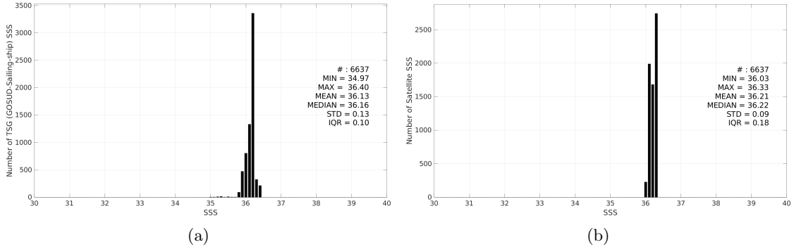
Figure 3: Histograms of SSS from TSG (GOSUD-Sailing-ship) (a) and CCI SSS L4 Merged-OI v4.41 - 30-day running (ESA) (b) considering all match-up pairs per bins of 0.1 over the Gulf of Mexico Pi-MEP region and for the full satellite product period.
