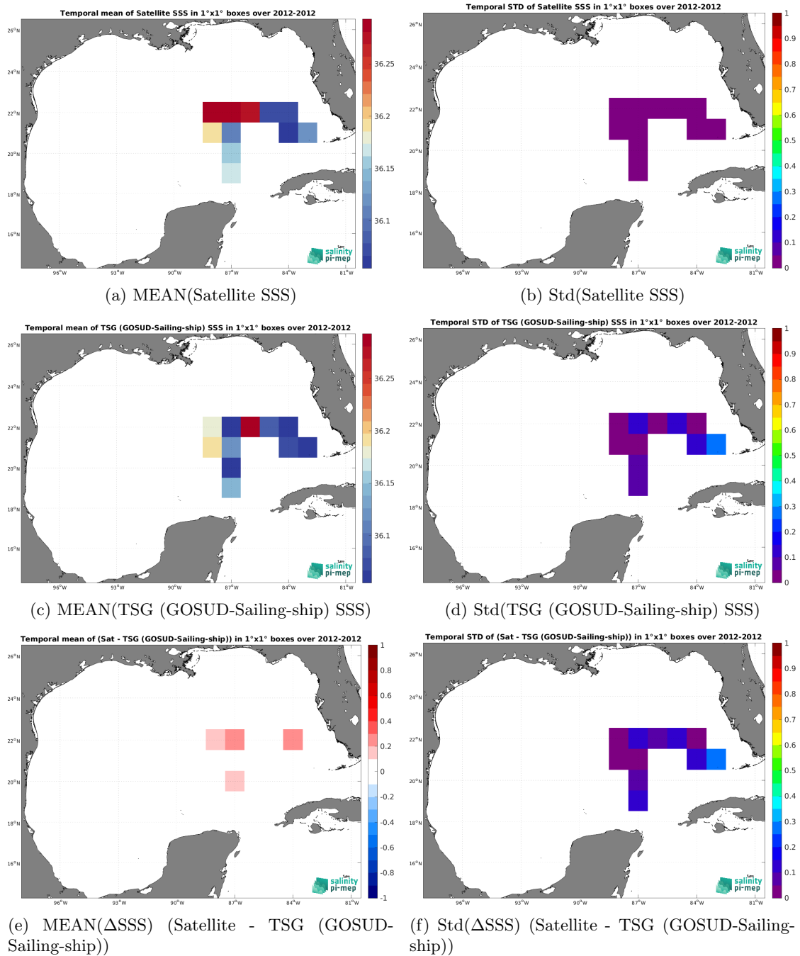
Figure 7: Temporal mean (left) and Std (right) of SSS from CCI SSS L4 Merged-OI v4.41 - 30-day running (ESA) (top), TSG (GOSUD-Sailing-ship) (middle), and of \Delta SSS (Satellite - TSG (GOSUD-Sailing-ship)). Only match-up pairs are used to generate these maps.
