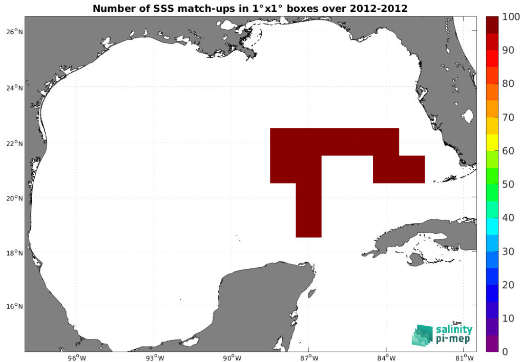
Figure 5: Number of SSS match-ups between TSG (GOSUD-Sailing-ship) SSS and the CCI SSS L4 Merged-OI v4.41 - 30-day running (ESA) SSS product for the Gulf of Mexico Pi-MEP region over 1^\circ \times 1^\circ boxes and for the full satellite product period.
