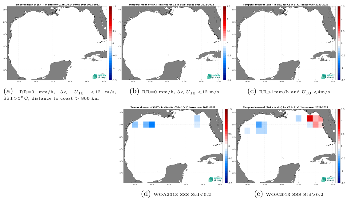
Figure 14: Temporal mean gridded over spatial boxes of size 1^\circ \times 1^\circ of \Delta\text{SSS} (CCI SSS L4 Merged-OI v4.41 - 30-day running (ESA) - Saildrone) for 5 different subdatasets corresponding to:RR=0 mm/h, 3 < U_{10} < 12 m/s, SST>5°C, distance to coast > 800 km (a), RR=0 mm/h, 3 < U_{10} < 12 m/s (b), RR>1mm/h and U_{10} < 4 m/s (c), WOA2013 SSS Std<0.2 (d), WOA2013 SSS Std>0.2 (e).
