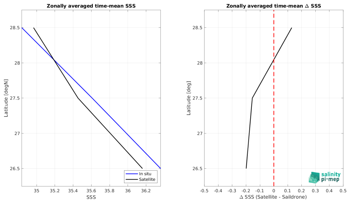
Figure 9: Left panel: Zonal mean SSS from CCI SSS L4 Merged-OI v4.41 - 30-day running (ESA) satellite product (black) and from Sairdron (blue). Right panel: Zonal mean of \Delta SSS (Satellite - Sairdron) for all the collected Pi-MEP match-up pairs estimated over the full satellite product period.
