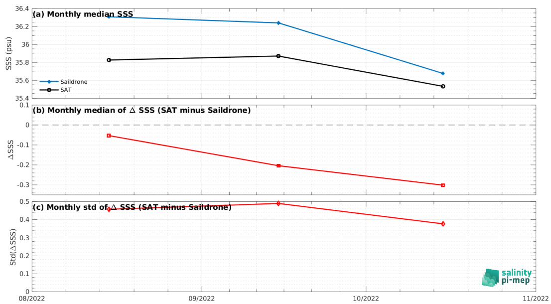
Figure 8: Time series of the monthly median SSS (top), median of \Delta SSS (Satellite - Saildrone) and Std of \Delta SSS (Satellite - Saildrone) over the Gulf of Mexico Pi-MEP region considering all match-ups collected by the Pi-MEP.
