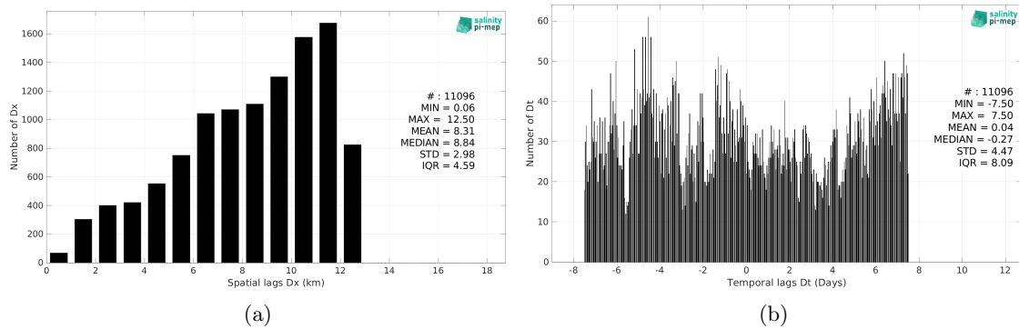
Figure 6: Histograms of the spatial (a) and temporal (b) lags between the location/time of the Saildrone measurement and the date of the corresponding CCI SSS L4 Merged-OI v4.41 - 30-day running (ESA) SSS pixel.
