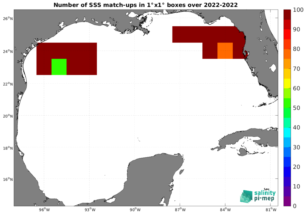
Figure 5: Number of SSS match-ups between Saildrone SSS and the CCI SSS L4 Merged-OI v4.41 - 30-day running (ESA) SSS product for the Gulf of Mexico Pi-MEP region over 1^\circ \times 1^\circ boxes and for the full satellite product period.
