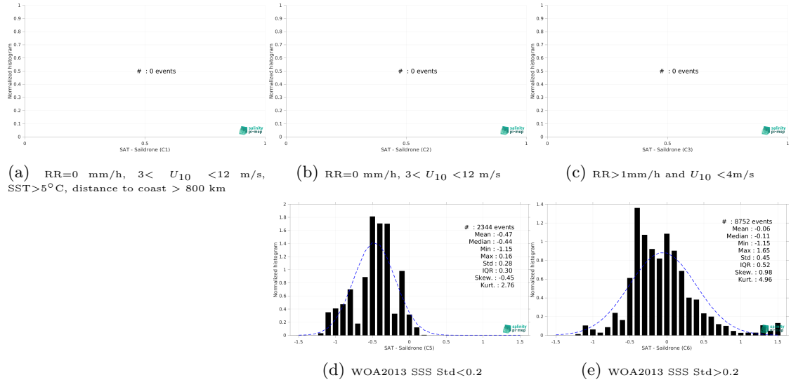
Figure 15: Normalized histogram of \Delta SSS (CCI SSS L4 Merged-OI v4.41 - 30-day running (ESA) - Saldrone) for 5 different subdatasets corresponding to: RR=0 mm/h, 3 < U_{10} < 12 m/s, SST>5°C, distance to coast > 800 km (a), RR=0 mm/h, 3 < U_{10} < 12 m/s (b), RR>1mm/h and U_{10} < 4 m/s (c), WOA2013 SSS Std<0.2 (d), WOA2013 SSS Std>0.2 (e).
