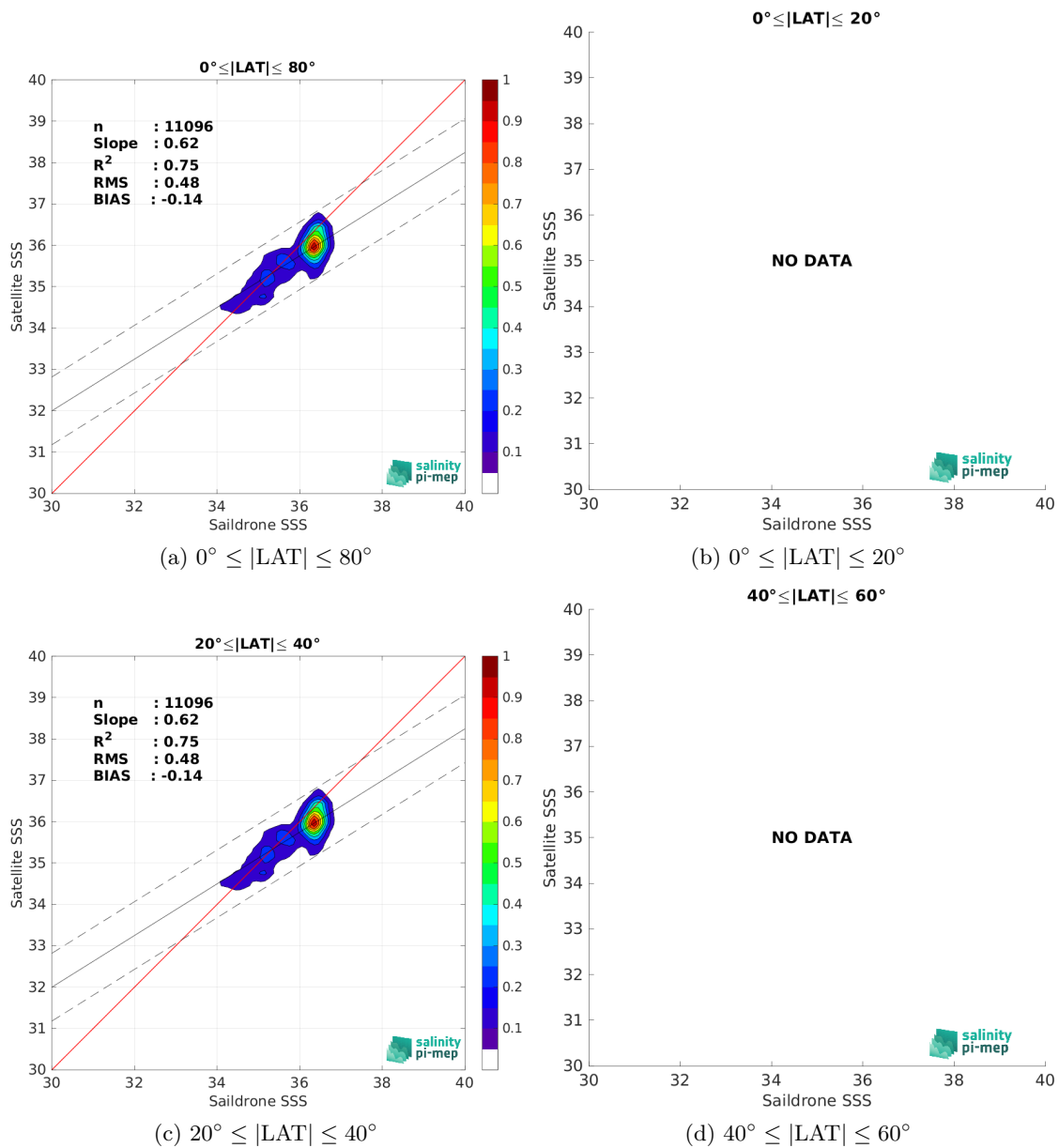
Figure 10: Contour maps of the concentration of CCI SSS L4 Merged-OI v4.41 - 30-day running (ESA) SSS (y-axis) versus Saildrone SSS (x-axis) at match-up pairs for different latitude bands. For each plot, the red line shows x=y . The black thin and dashed lines indicate a linear fit through the data cloud and the \pm 95\% confidence levels, respectively. The number match-up pairs n , the slope and R^2 coefficient of the linear fit, the root mean square (RMS) and the mean bias between satellite and in situ data are indicated for each latitude band in each plots.
