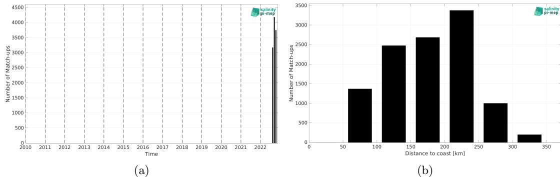
Figure 2: Number of match-ups between Saildrone and CCI SSS L4 Merged-OI v4.41 - 30-day running (ESA) SSS as a function of time (a) and as function of the distance to coast (b) over the Gulf of Mexico Pi-MEP region and for the full satellite product period.
