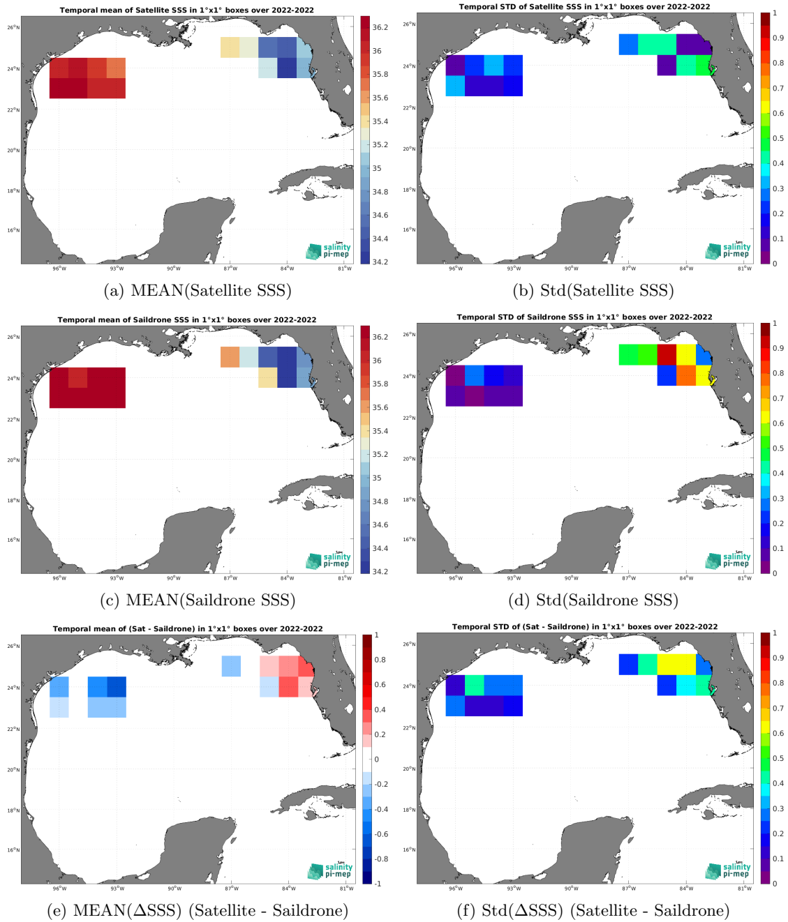
Figure 7: Temporal mean (left) and Std (right) of SSS from CCI SSS L4 Merged-OI v4.41 - 30-day running (ESA) (top), Saildrone (middle), and of \Delta SSS (Satellite - Saildrone). Only match-up pairs are used to generate these maps.
