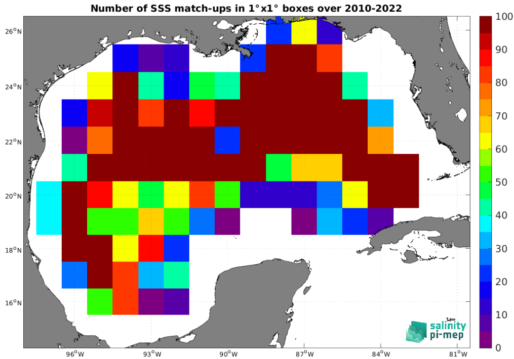
Figure 5: Number of SSS match-ups between Argo SSS and the CCI SSS L4 Merged-OI v4.41 - 30-day running (ESA) SSS product for the Gulf of Mexico Pi-MEP region over 1^\circ \times 1^\circ boxes and for the full satellite product period.
