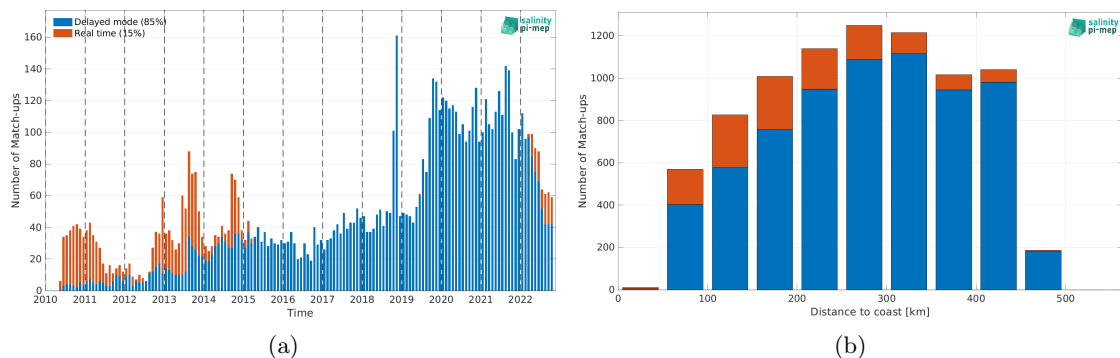
Figure 2: Number of match-ups between Argo and CCI SSS L4 Merged-OI v4.41 - 30-day running (ESA) SSS as a function of time (a) and as function of the distance to coast (b) over the Gulf of Mexico Pi-MEP region and for the full satellite product period.
