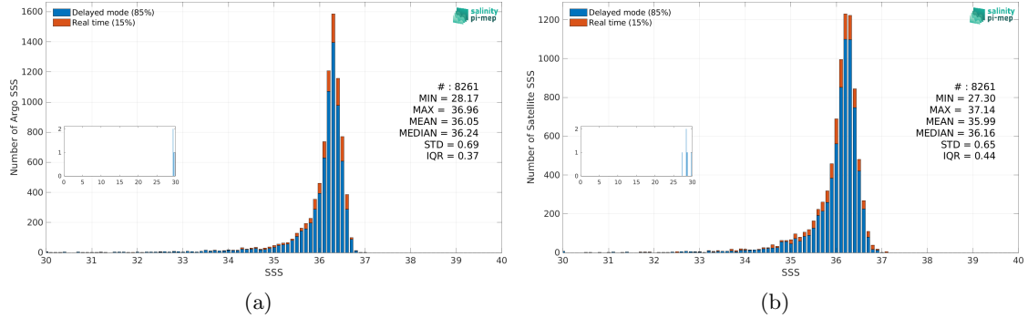
Figure 3: Histograms of SSS from Argo (a) and CCI SSS L4 Merged-OI v4.41 - 30-day running (ESA) (b) considering all match-up pairs per bins of 0.1 over the Gulf of Mexico Pi-MEP region and for the full satellite product period.
