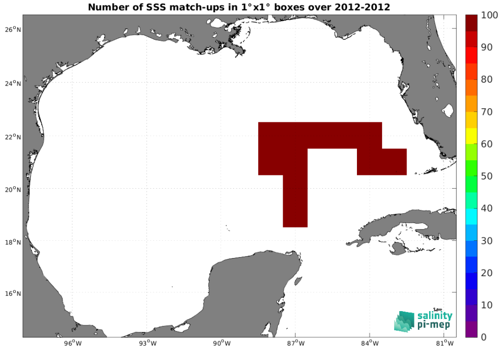
Figure 4: Number of SSS match-ups between TSG (GOSUD-Sailing-ship) SSS and the CCI SSS L4 Merged-OI v4.4 - 7-day running (ESA) SSS product for the Gulf of Mexico Pi-MEP region over 1^\circ \times 1^\circ boxes and for the full satellite product period.
