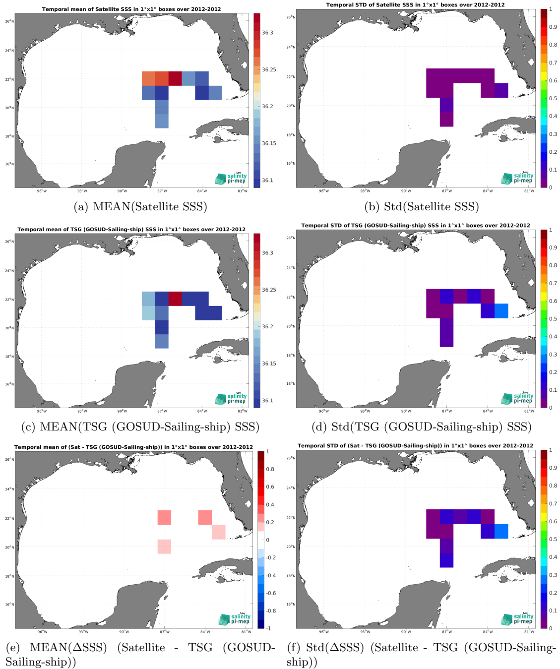
Figure 6: Temporal mean (left) and Std (right) of SSS from CCI SSS L4 Merged-OI v4.4 - 7-day running (ESA) (top), TSG (GOSUD-Sailing-ship) (middle), and of \Delta SSS (Satellite - TSG (GOSUD-Sailing-ship)). Only match-up pairs are used to generate these maps.
