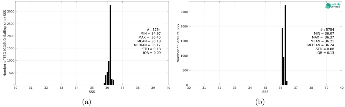
Figure 2: Histograms of SSS from TSG (GOSUD-Sailing-ship) (a) and CCI SSS L4 Merged-OI v4.4 - 7-day running (ESA) (b) considering all match-up pairs per bins of 0.1 over the Gulf of Mexico Pi-MEP region and for the full satellite product period.
