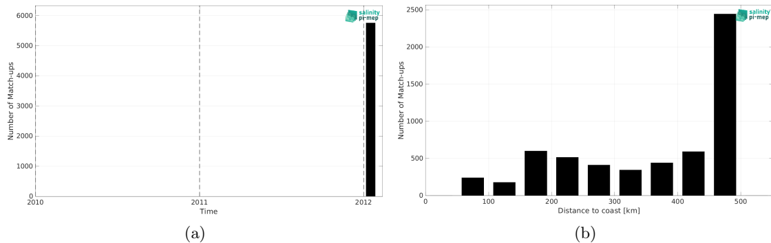
Figure 1: Number of match-ups between TSG (GOSUD-Sailing-ship) and CCI SSS L4 Merged-OI v4.4 - 7-day running (ESA) SSS as a function of time (a) and as function of the distance to coast (b) over the Gulf of Mexico Pi-MEP region and for the full satellite product period.
