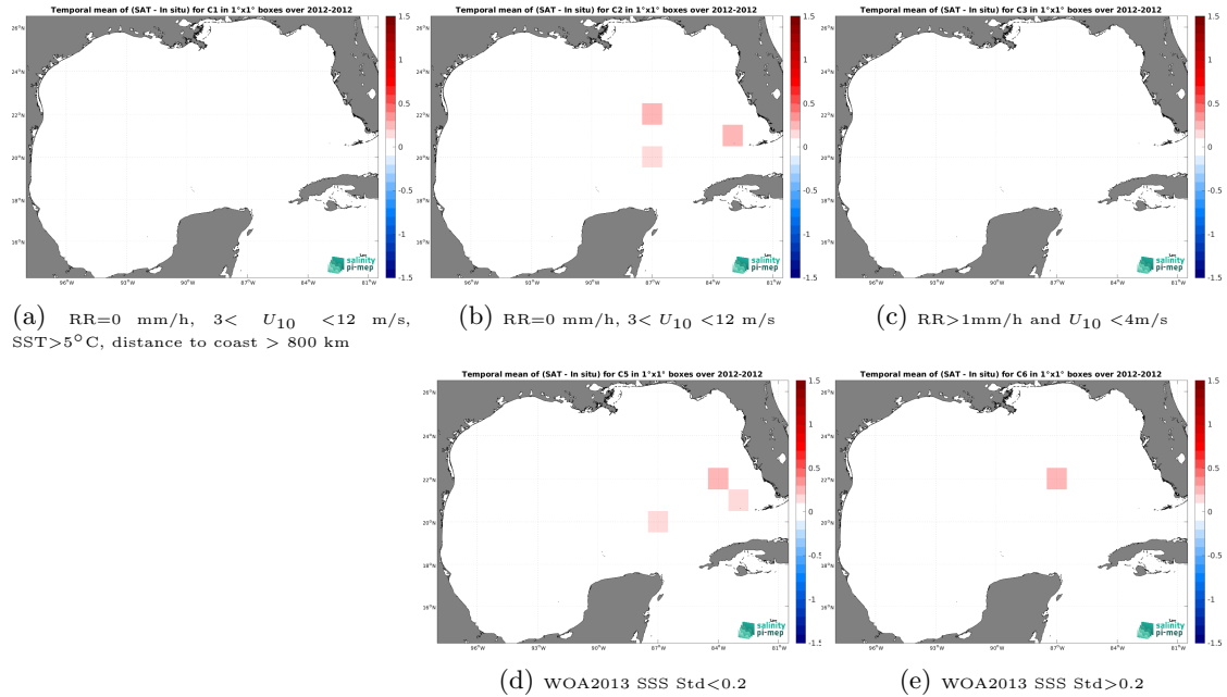
Figure 12: Temporal mean gridded over spatial boxes of size 1^{\circ}\times 1^{\circ} of \Delta SSS (CCI SSS L4 Merged-OI v4.4 - 7-day running (ESA) - TSG (GOSUD-Sailing-ship)) for 5 different subdatasets corresponding to:RR=0 mm/h, 3 < U_{10} < 12 m/s, SST >5^{\circ}\text{C} , distance to coast > 800 km (a), RR=0 mm/h, 3 < U_{10} < 12 m/s (b), RR >1 mm/h and U_{10} < 4 m/s (c), WOA2013 SSS Std <0.2 (d), WOA2013 SSS Std >0.2 (e).
