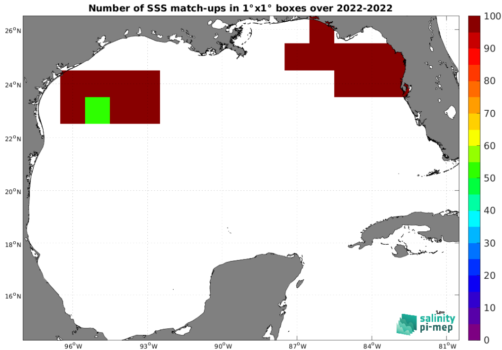
Figure 4: Number of SSS match-ups between Saildrone SSS and the CCI SSS L4 Merged-OI v4.4 - 7-day running (ESA) SSS product for the Gulf of Mexico Pi-MEP region over 1^\circ \times 1^\circ boxes and for the full satellite product period.
