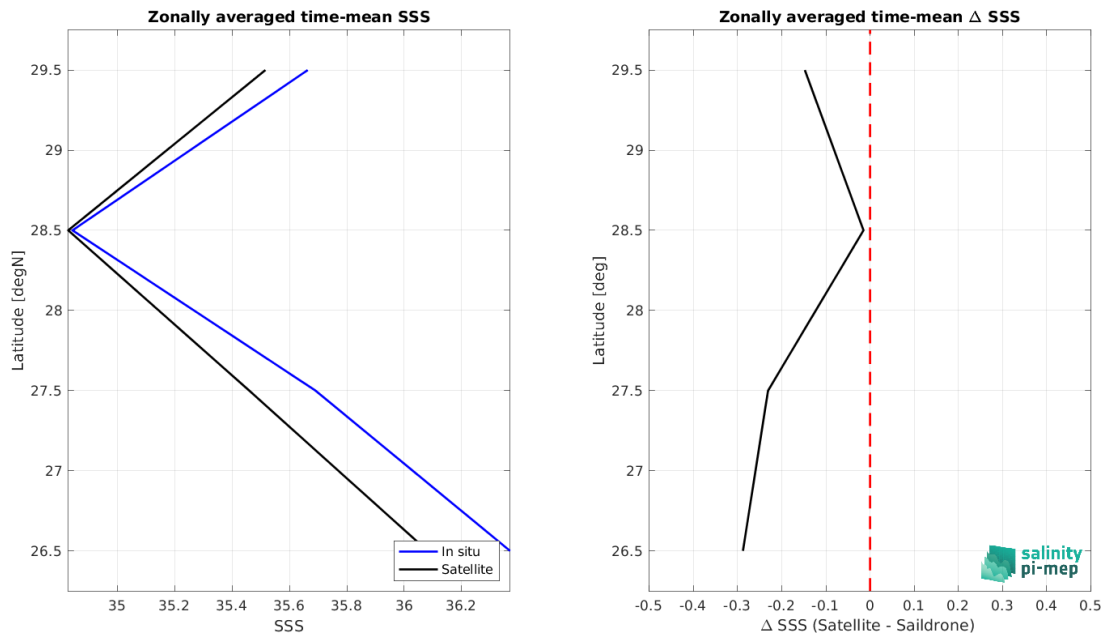
Figure 8: Left panel: Zonal mean SSS from CCI SSS L4 Merged-OI v4.4 - 7-day running (ESA) satellite product (black) and from Sairdron (blue). Right panel: Zonal mean of \Delta SSS (Satellite - Sairdron) for all the collected Pi-MEP match-up pairs estimated over the full satellite product period.
