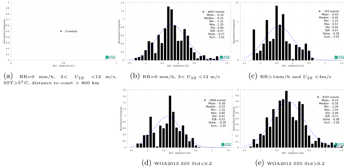
Figure 13: Normalized histogram of \Delta SSS (CCI SSS L4 Merged-OI v4.4 - 7-day running (ESA) - Saildrone) for 5 different subdatasets corresponding to: RR=0 mm/h, 3 < U_{10} < 12 m/s, SST > 5°C, distance to coast > 800 km (a), RR=0 mm/h, 3 < U_{10} < 12 m/s (b), RR > 1mm/h and U_{10} < 4 m/s (c), WOA2013 SSS Std < 0.2 (d), WOA2013 SSS Std > 0.2 (e).
