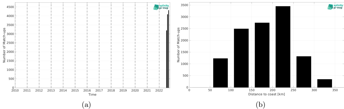
Figure 1: Number of match-ups between Saildrone and CCI SSS L4 Merged-OI v4.4 - 7-day running (ESA) SSS as a function of time (a) and as function of the distance to coast (b) over the Gulf of Mexico Pi-MEP region and for the full satellite product period.
