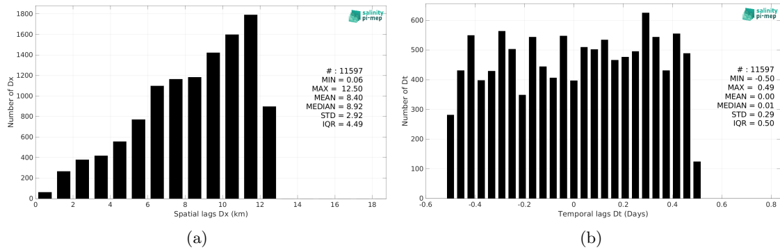
Figure 5: Histograms of the spatial (a) and temporal (b) lags between the location/time of the Saildrone measurement and the date of the corresponding CCI SSS L4 Merged-OI v4.4 - 7-day running (ESA) SSS pixel.
