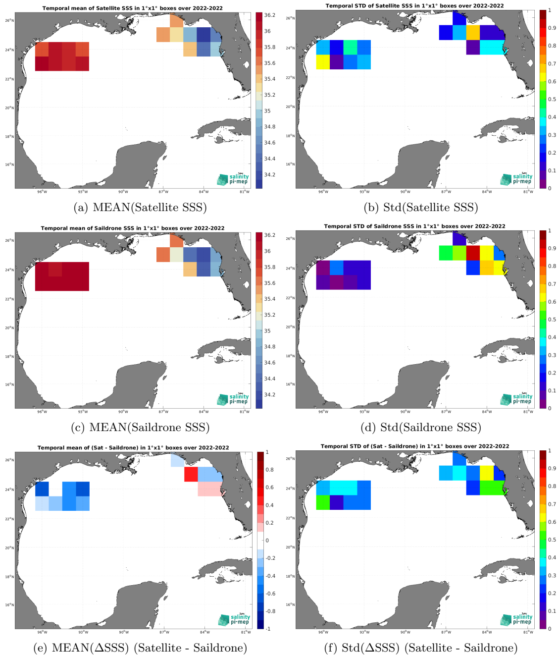
Figure 6: Temporal mean (left) and Std (right) of SSS from CCI SSS L4 Merged-OI v4.4 - 7-day running (ESA) (top), Saildrone (middle), and of \Delta SSS (Satellite - Saildrone). Only match-up pairs are used to generate these maps.
