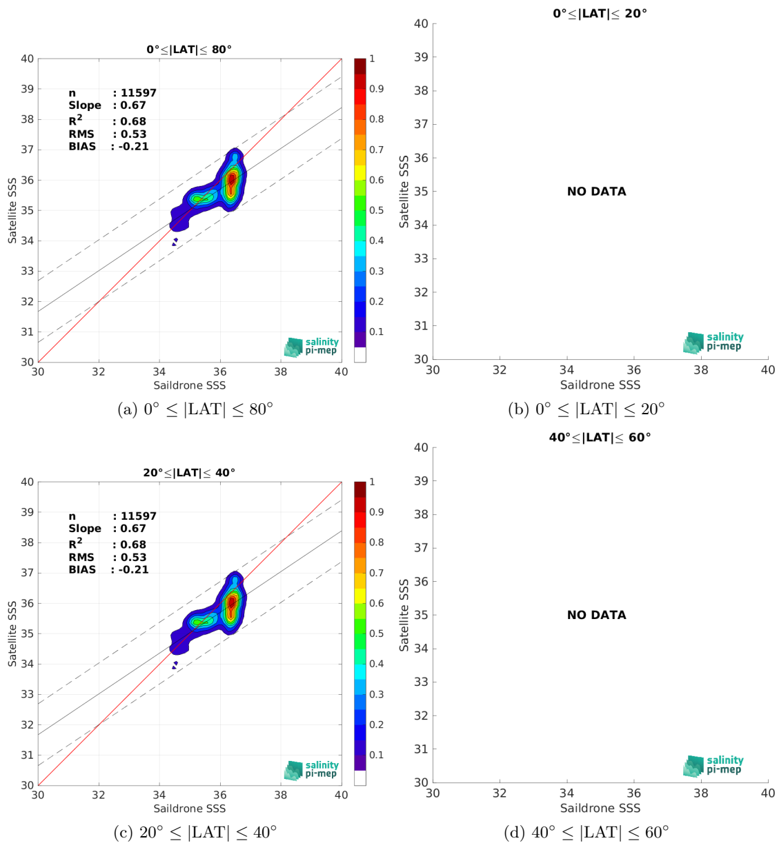
Figure 9: Contour maps of the concentration of CCI SSS L4 Merged-OI v4.4 - 7-day running (ESA) SSS (y-axis) versus Saildrone SSS (x-axis) at match-up pairs for different latitude bands. For each plot, the red line shows x=y . The black thin and dashed lines indicate a linear fit through the data cloud and the \pm 95\% confidence levels, respectively. The number match-up pairs n , the slope and R^2 coefficient of the linear fit, the root mean square (RMS) and the mean bias between satellite and in situ data are indicated for each latitude band in each plots.
