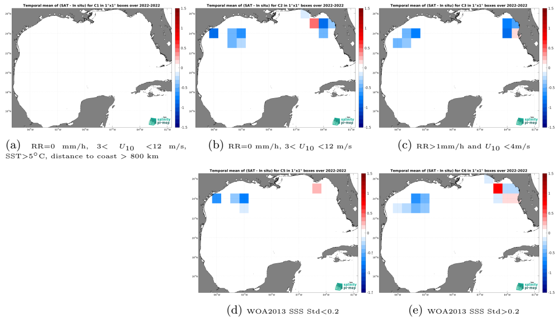
Figure 12: Temporal mean gridded over spatial boxes of size 1^{\circ}\times 1^{\circ} of \Delta\text{SSS} (CCI SSS L4 Merged-OI v4.4 - 7-day running (ESA) - Saildrone) for 5 different subdatasets corresponding to:RR=0 mm/h, 3 < U_{10} < 12 m/s, SST >5^{\circ}\text{C} , distance to coast > 800 km (a), RR=0 mm/h, 3 < U_{10} < 12 m/s (b), RR >1 mm/h and U_{10} < 4 m/s (c), WOA2013 SSS Std <0.2 (d), WOA2013 SSS Std >0.2 (e).
