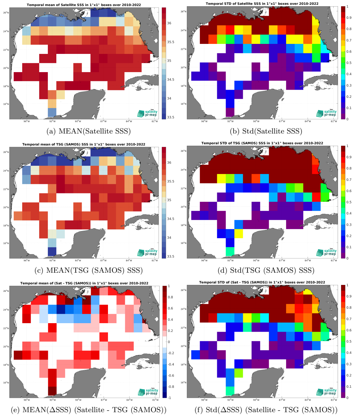
Figure 6: Temporal mean (left) and Std (right) of SSS from CCI SSS L4 Merged-OI v4.4 - 30-day running (ESA) (top), TSG (SAMOS) (middle), and of \Delta SSS (Satellite - TSG (SAMOS)). Only match-up pairs are used to generate these maps.
