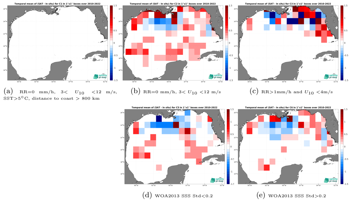
Figure 12: Temporal mean gridded over spatial boxes of size 1^\circ \times 1^\circ of \Delta SSS (CCI SSS L4 Merged-OI v4.4 - 30-day running (ESA) - TSG (SAMOS)) for 5 different subdatasets corresponding to:RR=0 mm/h, 3 < U_{10} < 12 m/s, SST >5^\circ C, distance to coast > 800 km (a), RR=0 mm/h, 3 < U_{10} < 12 m/s (b), RR >1 mm/h and U_{10} < 4 m/s (c), WOA2013 SSS Std <0.2 (d), WOA2013 SSS Std >0.2 (e).
