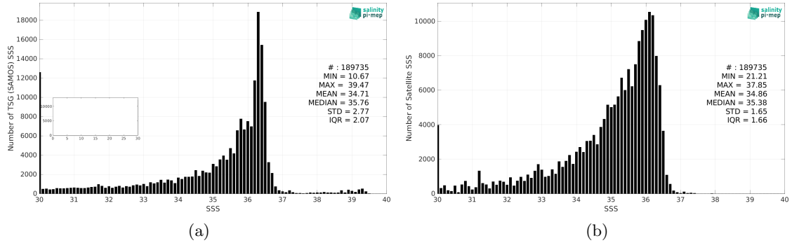
Figure 2: Histograms of SSS from TSG (SAMOS) (a) and CCI SSS L4 Merged-OI v4.4 - 30-day running (ESA) (b) considering all match-up pairs per bins of 0.1 over the Gulf of Mexico Pi-MEP region and for the full satellite product period.
