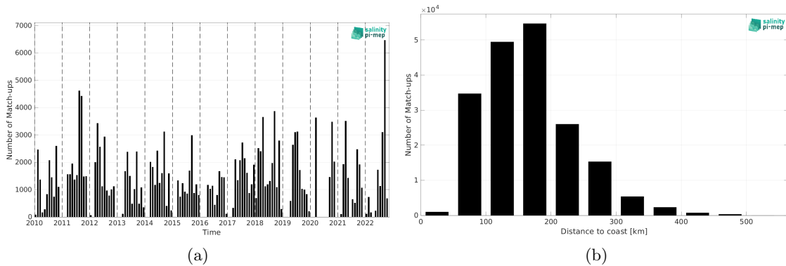
Figure 1: Number of match-ups between TSG (SAMOS) and CCI SSS L4 Merged-OI v4.4 - 30-day running (ESA) SSS as a function of time (a) and as function of the distance to coast (b) over the Gulf of Mexico Pi-MEP region and for the full satellite product period.
