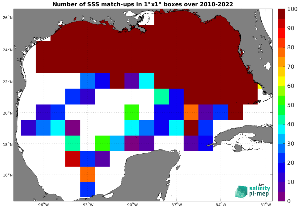
Figure 4: Number of SSS match-ups between TSG (SAMOS) SSS and the CCI SSS L4 Merged-OI v4.4 - 30-day running (ESA) SSS product for the Gulf of Mexico Pi-MEP region over 1^\circ \times 1^\circ boxes and for the full satellite product period.
