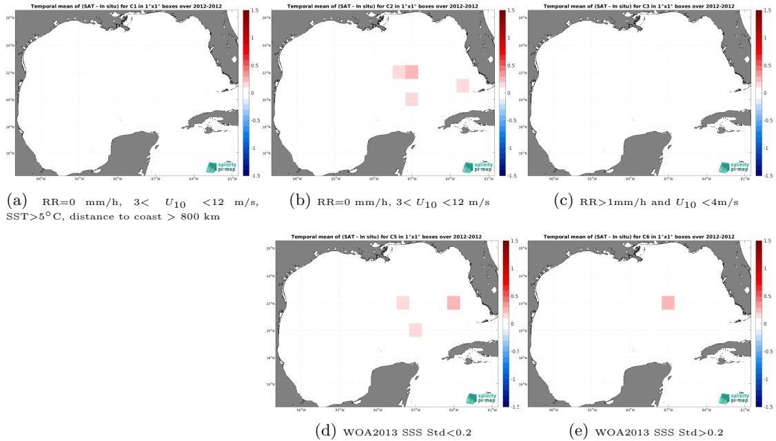
Figure 12: Temporal mean gridded over spatial boxes of size 1^{\circ}\times 1^{\circ} of \Delta SSS (CCI SSS L4 Merged-OI v4.4 - 30-day running (ESA) - TSG (GOSUD-Sailing-ship)) for 5 different subdatasets corresponding to:RR=0 mm/h, 3 < U_{10} < 12 m/s, SST >5^{\circ}\text{C} , distance to coast > 800 km (a), RR=0 mm/h, 3 < U_{10} < 12 m/s (b), RR >1 mm/h and U_{10} < 4 m/s (c), WOA2013 SSS Std <0.2 (d), WOA2013 SSS Std >0.2 (e).
