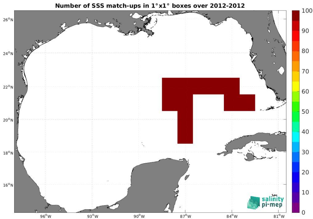
Figure 4: Number of SSS match-ups between TSG (GOSUD-Sailing-ship) SSS and the CCI SSS L4 Merged-OI v4.4 - 30-day running (ESA) SSS product for the Gulf of Mexico Pi-MEP region over 1^\circ \times 1^\circ boxes and for the full satellite product period.
