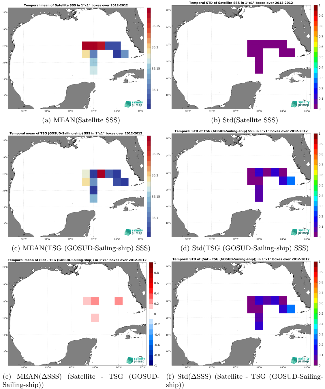
Figure 6: Temporal mean (left) and Std (right) of SSS from CCI SSS L4 Merged-OI v4.4 - 30-day running (ESA) (top), TSG (GOSUD-Sailing-ship) (middle), and of \Delta SSS (Satellite - TSG (GOSUD-Sailing-ship)). Only match-up pairs are used to generate these maps.
