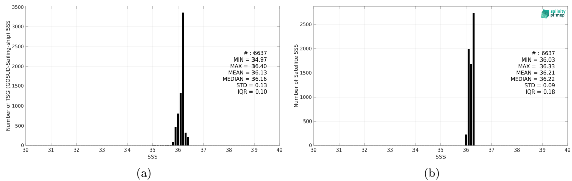
Figure 2: Histograms of SSS from TSG (GOSUD-Sailing-ship) (a) and CCI SSS L4 Merged-OI v4.4 - 30-day running (ESA) (b) considering all match-up pairs per bins of 0.1 over the Gulf of Mexico Pi-MEP region and for the full satellite product period.
