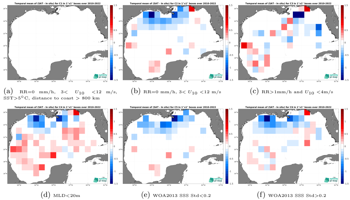
Figure 12: Temporal mean gridded over spatial boxes of size 1^\circ \times 1^\circ of \Delta SSS (CCI SSS L4 Merged-OI v4.4 - 30-day running (ESA) - Argo) for 6 different subdatasets corresponding to:RR=0 mm/h, 3 < U_{10} < 12 m/s, SST > 5^\circ\text{C} , distance to coast > 800 km (a), RR=0 mm/h, 3 < U_{10} < 12 m/s (b), RR > 1 mm/h and U_{10} < 4 m/s (c),MLD < 20 m (d),WOA2013 SSS Std < 0.2 (e),WOA2013 SSS Std > 0.2 (f).
