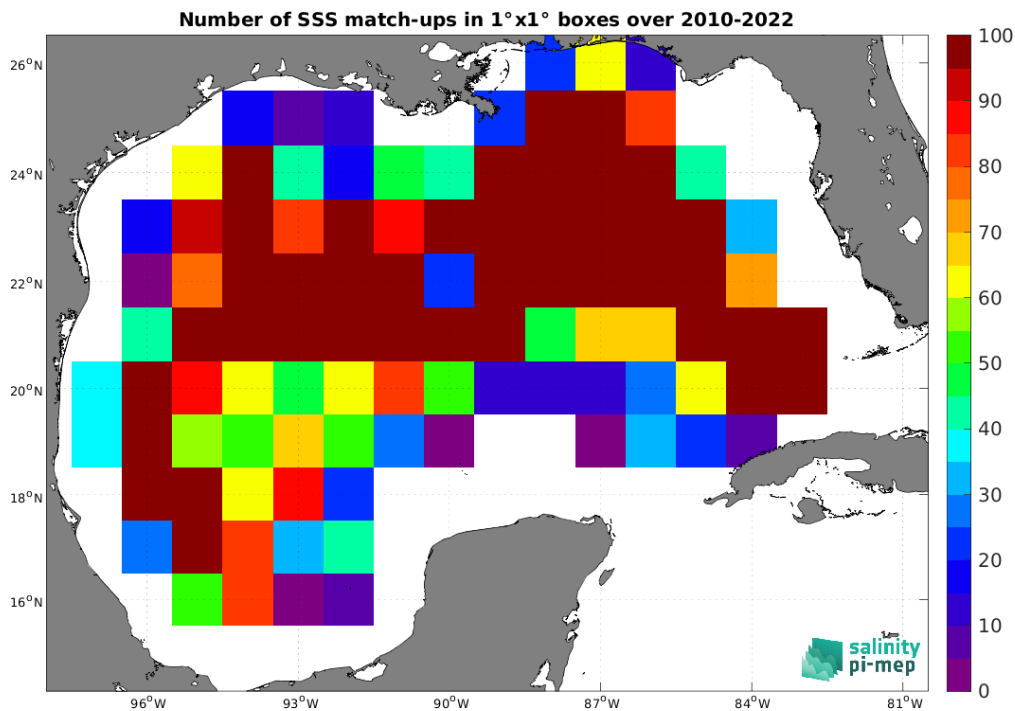
Figure 4: Number of SSS match-ups between Argo SSS and the CCI SSS L4 Merged-OI v4.4 - 30-day running (ESA) SSS product for the Gulf of Mexico Pi-MEP region over 1^\circ \times 1^\circ boxes and for the full satellite product period.
