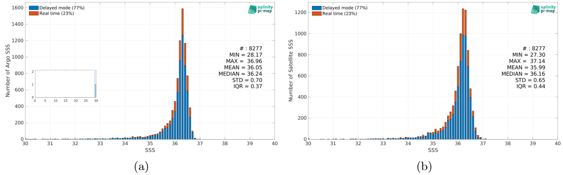
Figure 2: Histograms of SSS from Argo (a) and CCI SSS L4 Merged-OI v4.4 - 30-day running (ESA) (b) considering all match-up pairs per bins of 0.1 over the Gulf of Mexico Pi-MEP region and for the full satellite product period.
