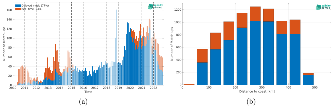
Figure 1: Number of match-ups between Argo and CCI SSS L4 Merged-OI v4.4 - 30-day running (ESA) SSS as a function of time (a) and as function of the distance to coast (b) over the Gulf of Mexico Pi-MEP region and for the full satellite product period.
