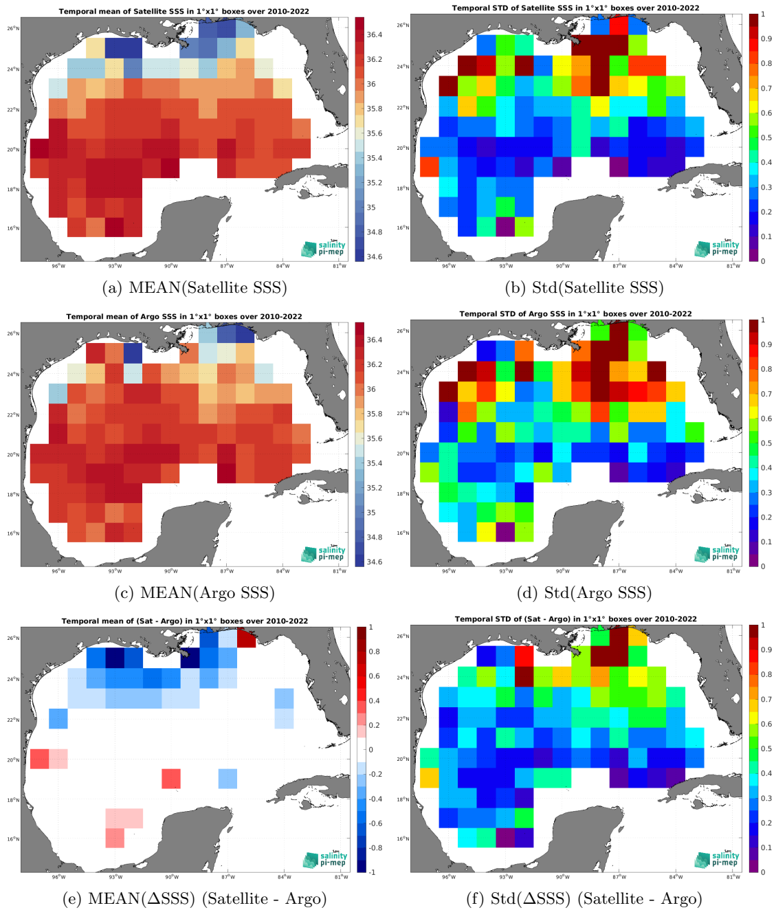
Figure 6: Temporal mean (left) and Std (right) of SSS from CCI SSS L4 Merged-OI v4.4 - 30-day running (ESA) (top), Argo (middle), and of \Delta SSS (Satellite - Argo). Only match-up pairs are used to generate these maps.
