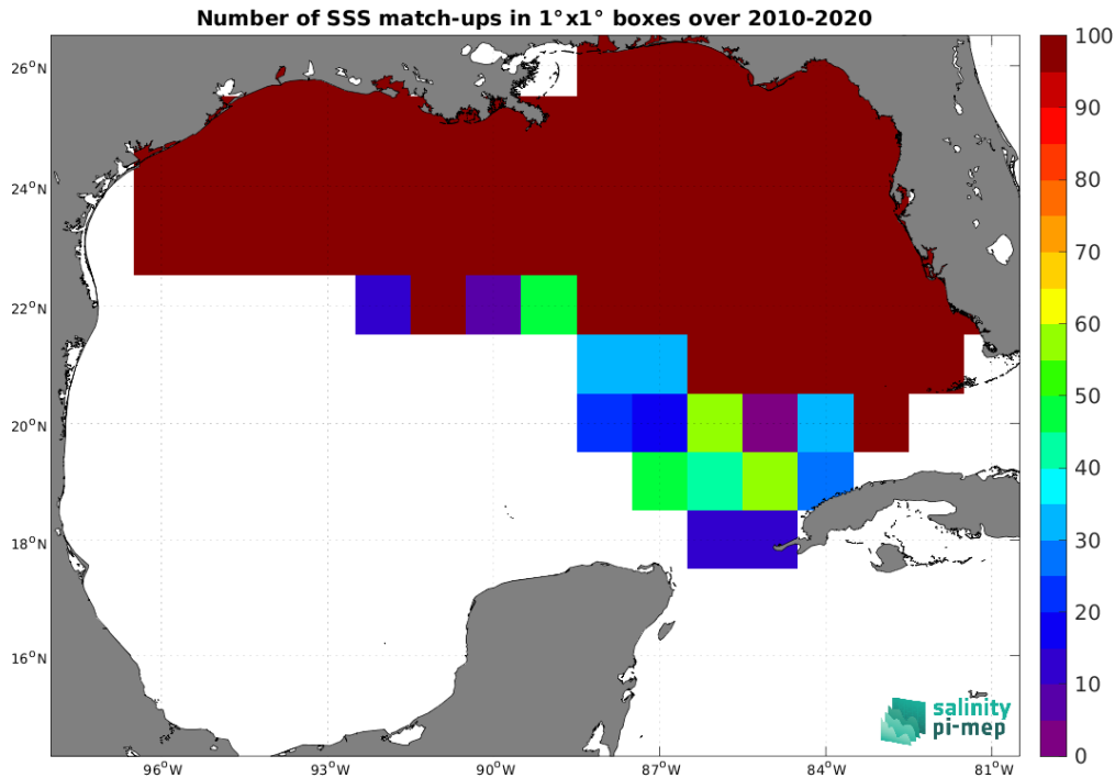
Figure 4: Number of SSS match-ups between TSG (SAMOS) SSS and the CCI SSS L4 Merged-OI v3.2 - 7-day running (ESA) SSS product for the Gulf of Mexico Pi-MEP region over 1^\circ \times 1^\circ boxes and for the full satellite product period.
