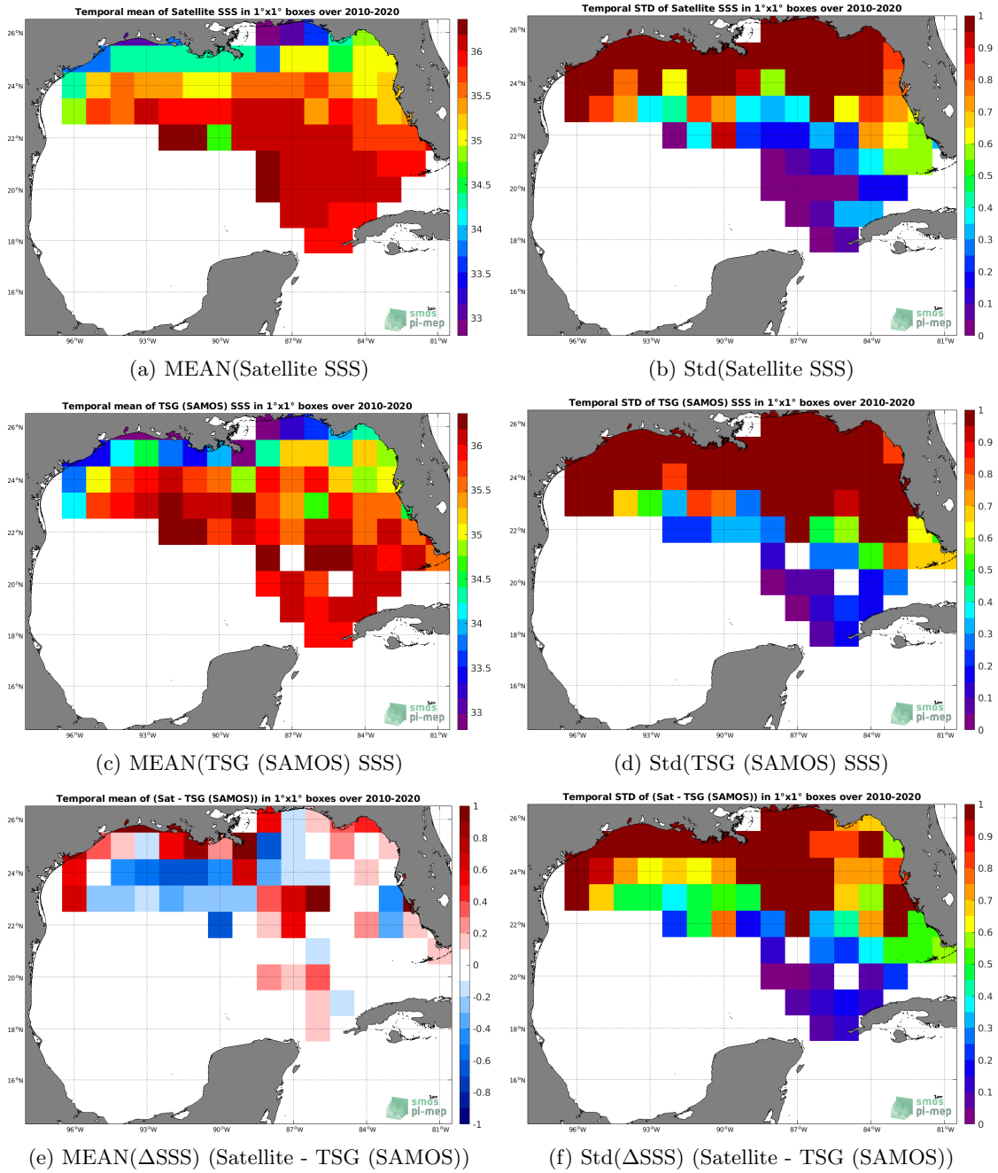
Figure 6: Temporal mean (left) and Std (right) of SSS from CCI SSS L4 Merged-OI v3.2 - 7-day running (ESA) (top), TSG (SAMOS) (middle), and of \Delta SSS (Satellite - TSG (SAMOS)). Only match-up pairs are used to generate these maps.
