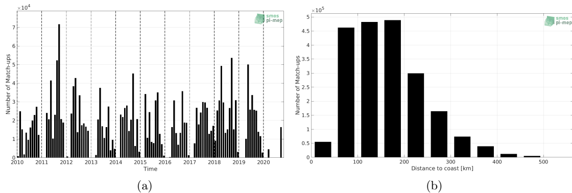
Figure 1: Number of match-ups between TSG (SAMOS) and CCI SSS L4 Merged-OI v3.2 - 7-day running (ESA) SSS as a function of time (a) and as function of the distance to coast (b) over the Gulf of Mexico Pi-MEP region and for the full satellite product period.
