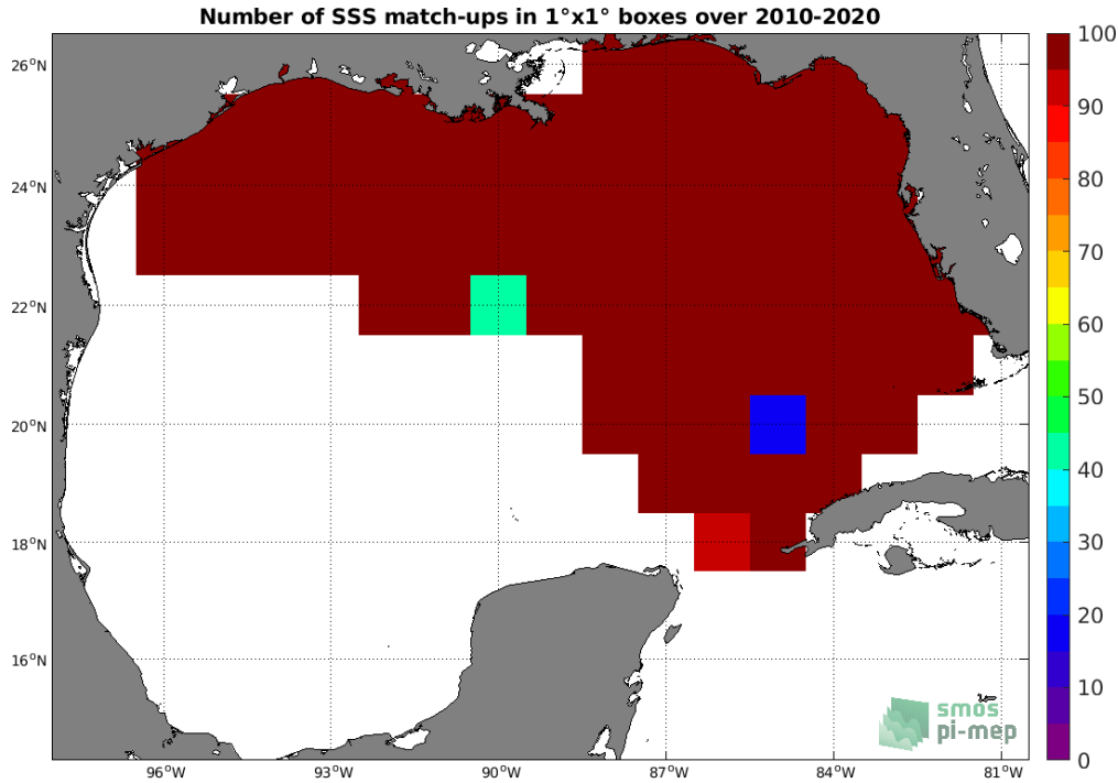
Figure 4: Number of SSS match-ups between TSG (SAMOS) SSS and the CCI SSS L4 Merged-OI v3.2 - 7-day running (ESA) SSS product for the Gulf of Mexico Pi-MEP region over 1°x1° boxes and for the full satellite product period.
