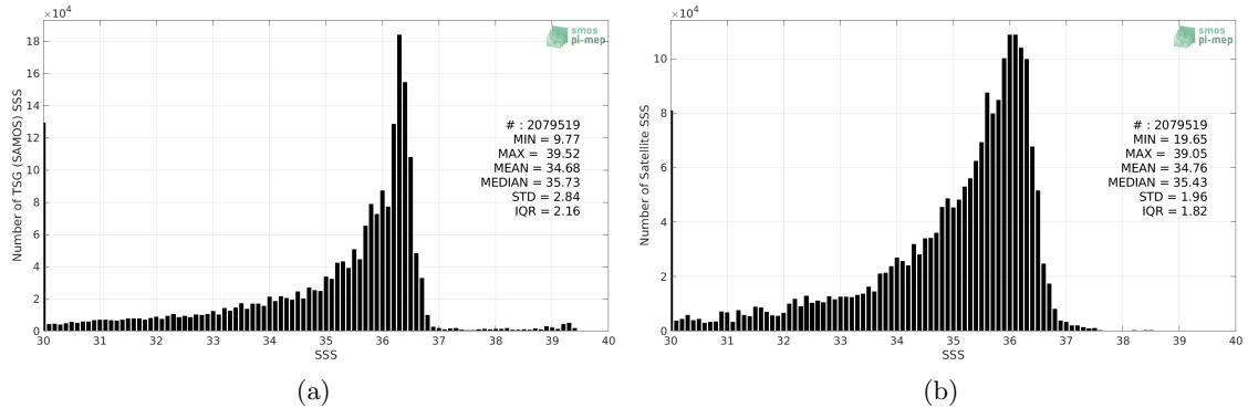
Figure 2: Histograms of SSS from TSG (SAMOS) (a) and CCI SSS L4 Merged-OI v3.2 - 7-day running (ESA) (b) considering all match-up pairs per bins of 0.1 over the Gulf of Mexico Pi-MEP region and for the full satellite product period.
