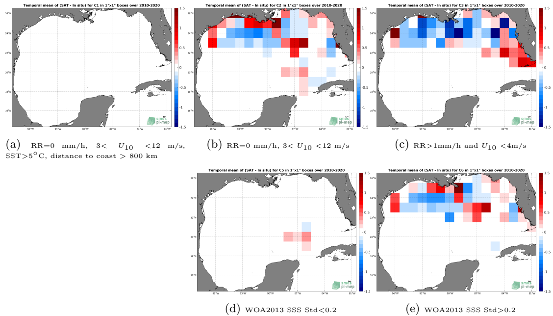
Figure 12: Temporal mean gridded over spatial boxes of size 1^{\circ}\times 1^{\circ} of \Delta\text{SSS} (CCI SSS L4 Merged-OI v3.2 - 7-day running (ESA) - TSG (SAMOS)) for 5 different subdatasets corresponding to:RR=0 mm/h, 3 < U_{10} < 12 m/s, SST >5^{\circ}\text{C} , distance to coast > 800 km (a), RR=0 mm/h, 3 < U_{10} < 12 m/s (b), RR >1 mm/h and U_{10} < 4 m/s (c), WOA2013 SSS Std <0.2 (d), WOA2013 SSS Std >0.2 (e).
