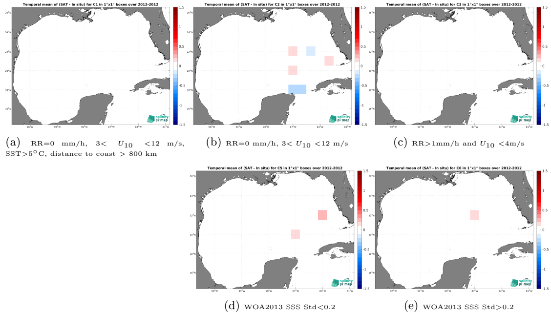
Figure 12: Temporal mean gridded over spatial boxes of size 1^{\circ}\times 1^{\circ} of \Delta SSS (CCI SSS L4 Merged-OI v3.2 - 7-day running (ESA) - TSG (GOSUD-Sailing-ship)) for 5 different subdatasets corresponding to:RR=0 mm/h, 3 < U_{10} < 12 m/s, SST >5^{\circ}\text{C} , distance to coast > 800 km (a), RR=0 mm/h, 3 < U_{10} < 12 m/s (b), RR >1 mm/h and U_{10} < 4 m/s (c), WOA2013 SSS Std <0.2 (d), WOA2013 SSS Std >0.2 (e).
