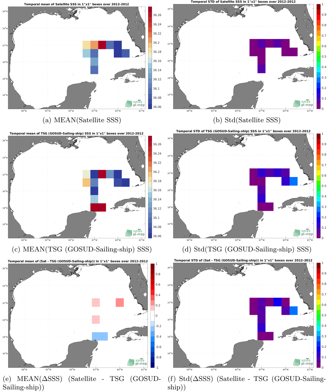
Figure 6: Temporal mean (left) and Std (right) of SSS from CCI SSS L4 Merged-OI v3.2 - 7-day running (ESA) (top), TSG (GOSUD-Sailing-ship) (middle), and of \Delta SSS (Satellite - TSG (GOSUD-Sailing-ship)). Only match-up pairs are used to generate these maps.
