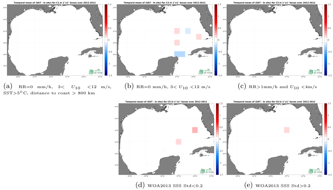
Figure 12: Temporal mean gridded over spatial boxes of size 1^\circ \times 1^\circ of \Delta SSS (CCI SSS L4 Merged-OI v3.2 - 7-day running (ESA) - TSG (GOSUD-Sailing-ship)) for 5 different subdatasets corresponding to: RR=0 mm/h, 3 < U_{10} < 12 m/s, SST >5^\circ\text{C} , distance to coast > 800 km (a), RR=0 mm/h, 3 < U_{10} < 12 m/s (b), RR >1 mm/h and U_{10} < 4 m/s (c), WOA2013 SSS Std <0.2 (d), WOA2013 SSS Std >0.2 (e).
