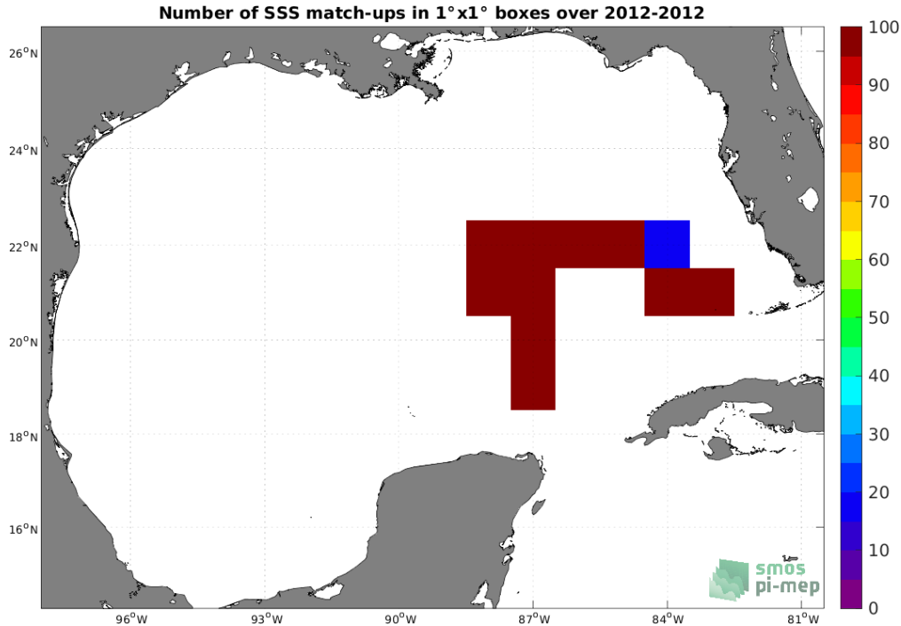
Figure 4: Number of SSS match-ups between TSG (GOSUD-Sailing-ship) SSS and the CCI SSS L4 Merged-OI v3.2 - 7-day running (ESA) SSS product for the Gulf of Mexico Pi-MEP region over 1^\circ \times 1^\circ boxes and for the full satellite product period.
