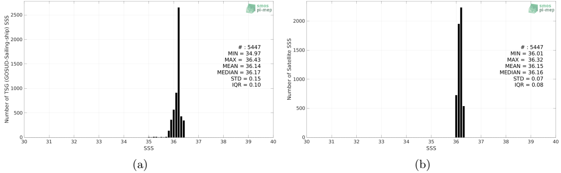
Figure 2: Histograms of SSS from TSG (GOSUD-Sailing-ship) (a) and CCI SSS L4 Merged-OI v3.2 - 7-day running (ESA) (b) considering all match-up pairs per bins of 0.1 over the Gulf of Mexico Pi-MEP region and for the full satellite product period.
