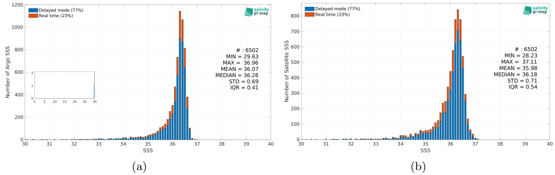
Figure 2: Histograms of SSS from Argo (a) and CCI SSS L4 Merged-OI v3.2 - 7-day running (ESA) (b) considering all match-up pairs per bins of 0.1 over the Gulf of Mexico Pi-MEP region and for the full satellite product period.
