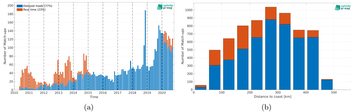
Figure 1: Number of match-ups between Argo and CCI SSS L4 Merged-OI v3.2 - 7-day running (ESA) SSS as a function of time (a) and as function of the distance to coast (b) over the Gulf of Mexico Pi-MEP region and for the full satellite product period.
