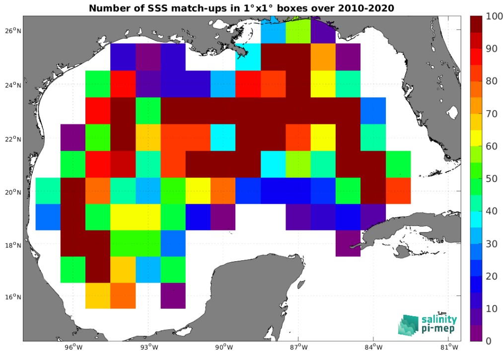
Figure 4: Number of SSS match-ups between Argo SSS and the CCI SSS L4 Merged-OI v3.2 - 7-day running (ESA) SSS product for the Gulf of Mexico Pi-MEP region over 1^\circ \times 1^\circ boxes and for the full satellite product period.
