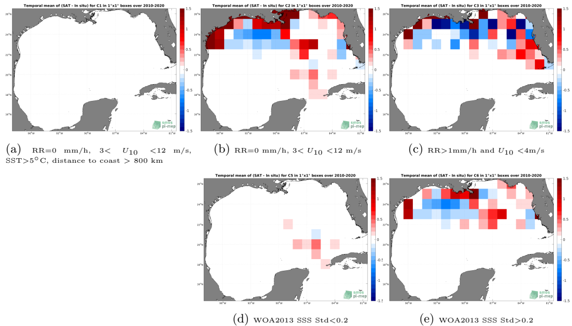
Figure 12: Temporal mean gridded over spatial boxes of size 1^{\circ}\times 1^{\circ} of \Delta\text{SSS} (CCI SSS L4 Merged-OI v3.2 - 30-day running (ESA) - TSG (SAMOS)) for 5 different subdatasets corresponding to:RR=0 mm/h, 3 < U_{10} < 12 m/s, SST >5^{\circ}\text{C} , distance to coast > 800 km (a), RR=0 mm/h, 3 < U_{10} < 12 m/s (b), RR >1 mm/h and U_{10} < 4 m/s (c), WOA2013 SSS Std <0.2 (d), WOA2013 SSS Std >0.2 (e).
