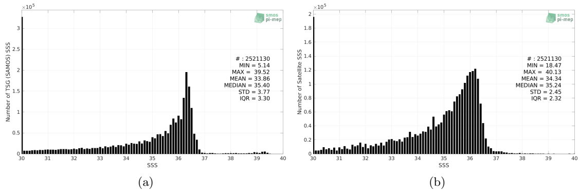
Figure 2: Histograms of SSS from TSG (SAMOS) (a) and CCI SSS L4 Merged-OI v3.2 - 30-day running (ESA) (b) considering all match-up pairs per bins of 0.1 over the Gulf of Mexico Pi-MEP region and for the full satellite product period.
