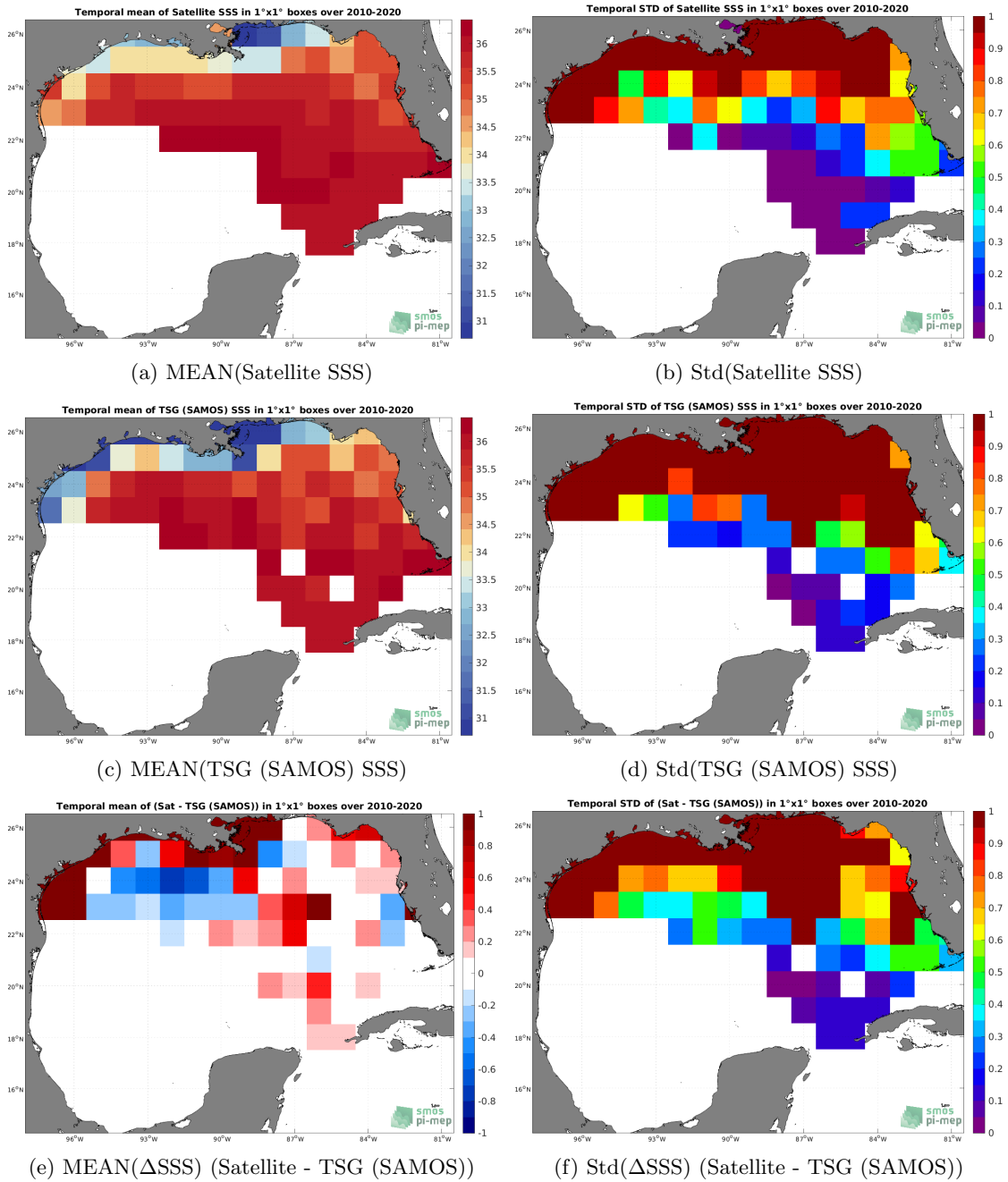
Figure 6: Temporal mean (left) and Std (right) of SSS from CCI SSS L4 Merged-OI v3.2 - 30-day running (ESA) (top), TSG (SAMOS) (middle), and of \Delta SSS (Satellite - TSG (SAMOS)). Only match-up pairs are used to generate these maps.
