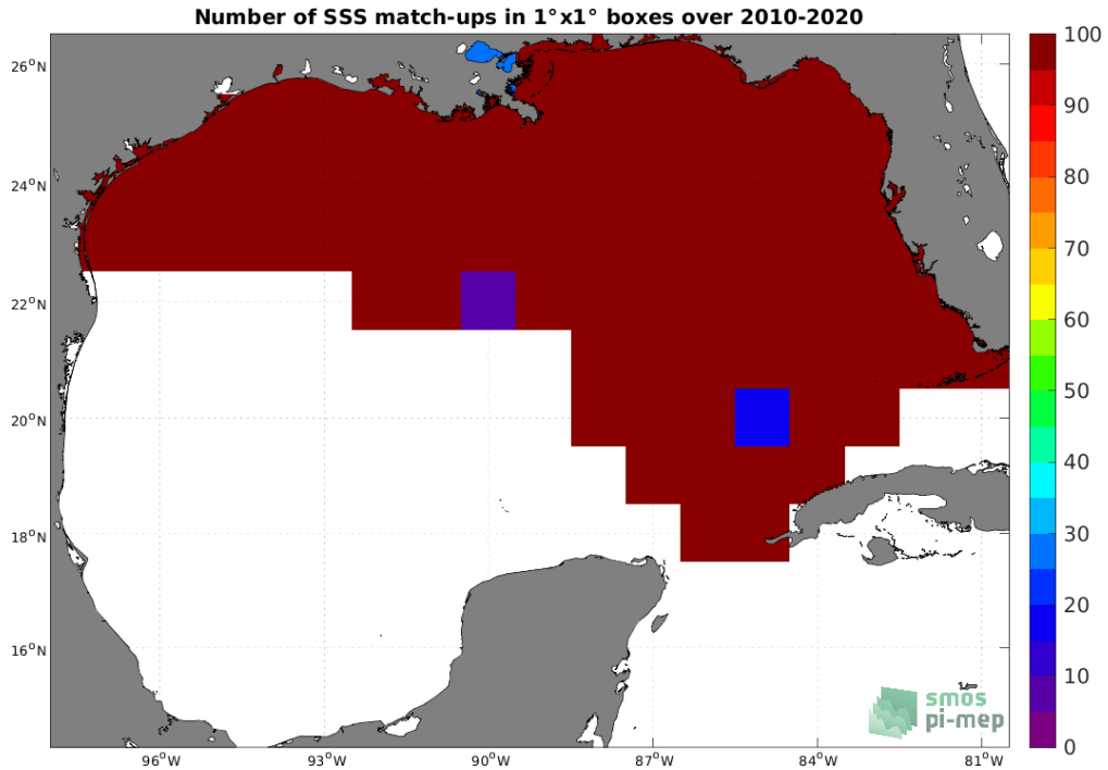
Figure 4: Number of SSS match-ups between TSG (SAMOS) SSS and the CCI SSS L4 Merged-OI v3.2 - 30-day running (ESA) SSS product for the Gulf of Mexico Pi-MEP region over 1^\circ \times 1^\circ boxes and for the full satellite product period.
