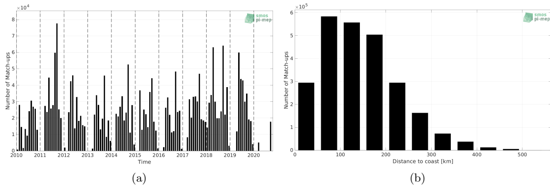
Figure 1: Number of match-ups between TSG (SAMOS) and CCI SSS L4 Merged-OI v3.2 - 30-day running (ESA) SSS as a function of time (a) and as function of the distance to coast (b) over the Gulf of Mexico Pi-MEP region and for the full satellite product period.
