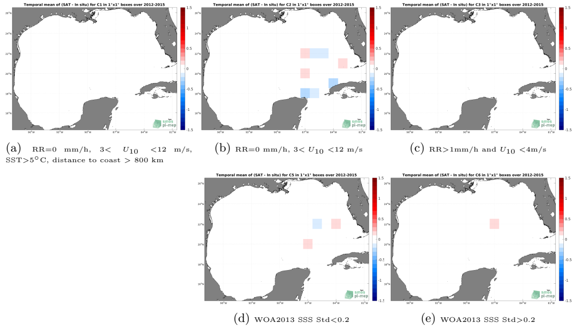
Figure 12: Temporal mean gridded over spatial boxes of size 1^{\circ}\times 1^{\circ} of \Delta SSS (CCI SSS L4 Merged-OI v3.2 - 30-day running (ESA) - TSG (GOSUD-Sailing-ship)) for 5 different subdatasets corresponding to:RR=0 mm/h, 3 < U_{10} < 12 m/s, SST >5^{\circ}\text{C} , distance to coast > 800 km (a), RR=0 mm/h, 3 < U_{10} < 12 m/s (b), RR >1 mm/h and U_{10} < 4 m/s (c), WOA2013 SSS Std <0.2 (d), WOA2013 SSS Std >0.2 (e).
