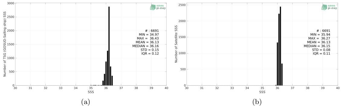
Figure 2: Histograms of SSS from TSG (GOSUD-Sailing-ship) (a) and CCI SSS L4 Merged-OI v3.2 - 30-day running (ESA) (b) considering all match-up pairs per bins of 0.1 over the Gulf of Mexico Pi-MEP region and for the full satellite product period.
