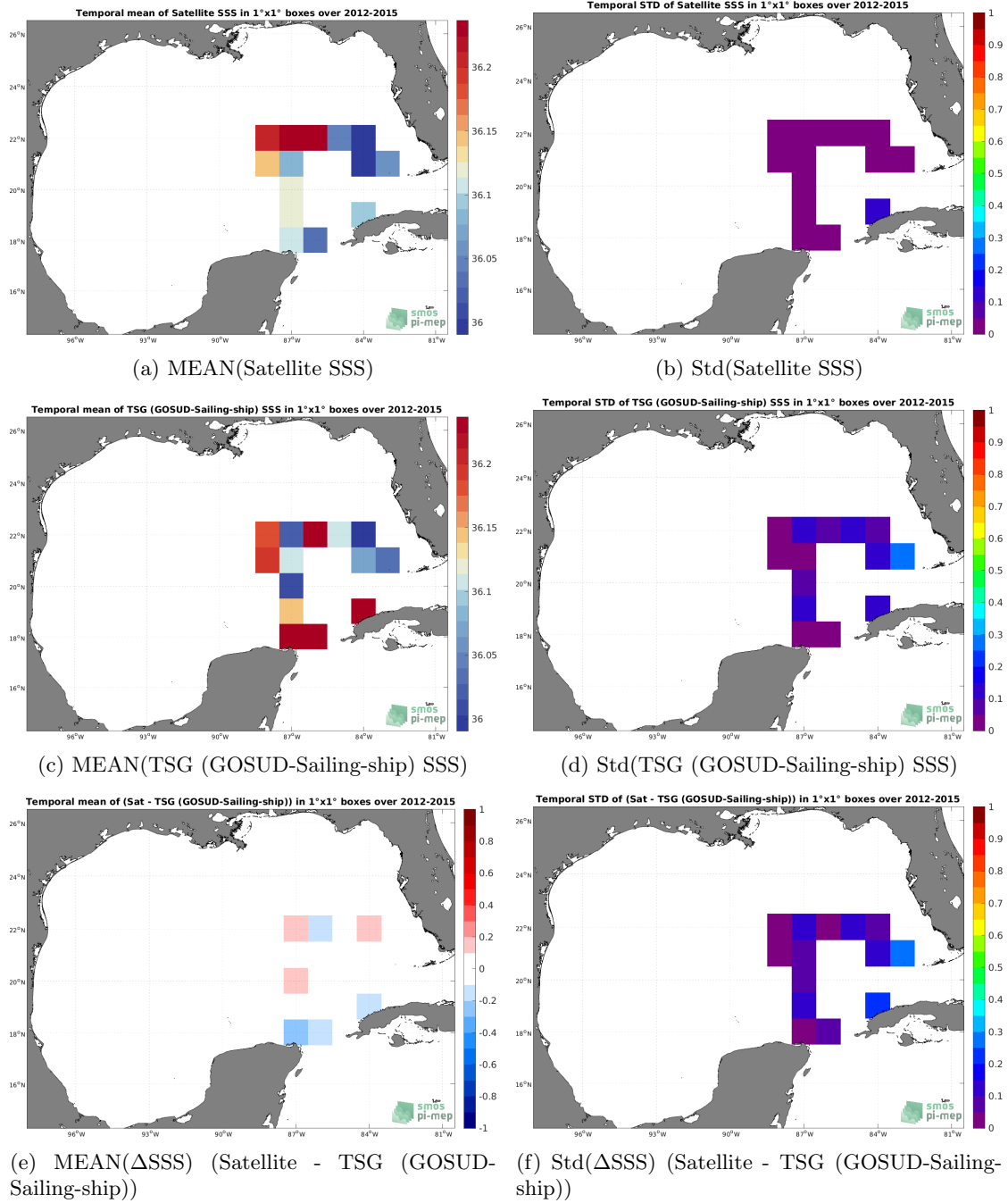
Figure 6: Temporal mean (left) and Std (right) of SSS from CCI SSS L4 Merged-OI v3.2 - 30-day running (ESA) (top), TSG (GOSUD-Sailing-ship) (middle), and of \Delta SSS (Satellite - TSG (GOSUD-Sailing-ship)). Only match-up pairs are used to generate these maps.
