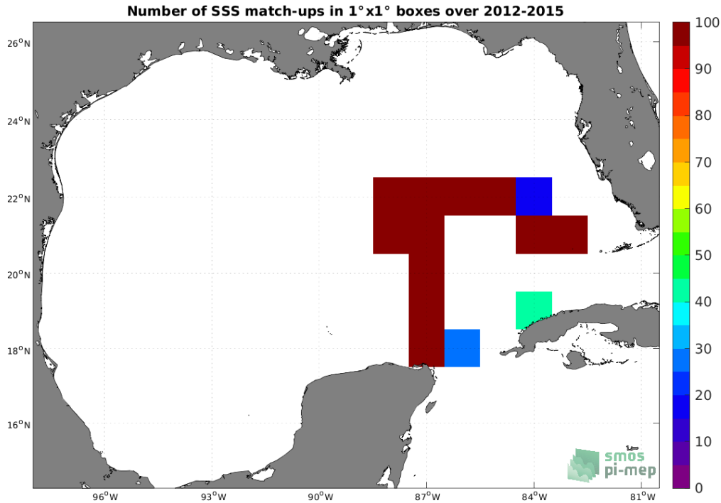
Figure 4: Number of SSS match-ups between TSG (GOSUD-Sailing-ship) SSS and the CCI SSS L4 Merged-OI v3.2 - 30-day running (ESA) SSS product for the Gulf of Mexico Pi-MEP region over 1^\circ \times 1^\circ boxes and for the full satellite product period.
