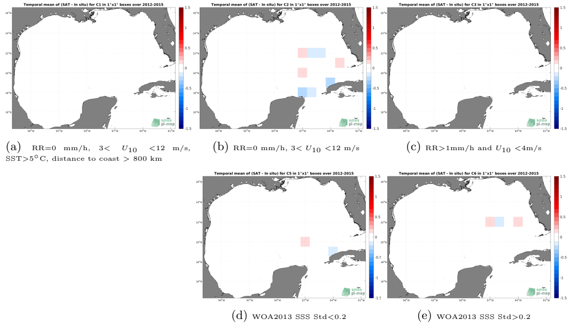
Figure 12: Temporal mean gridded over spatial boxes of size 1^\circ \times 1^\circ of \Delta SSS (CCI SSS L4 Merged-OI v3.2 - 30-day running (ESA) - TSG (GOSUD-Sailing-ship)) for 5 different subdatasets corresponding to: RR=0 mm/h, 3 < U_{10} < 12 m/s, SST >5^\circ\text{C} , distance to coast > 800 km (a), RR=0 mm/h, 3 < U_{10} < 12 m/s (b), RR >1 mm/h and U_{10} < 4 m/s (c), WOA2013 SSS Std <0.2 (d), WOA2013 SSS Std >0.2 (e).
