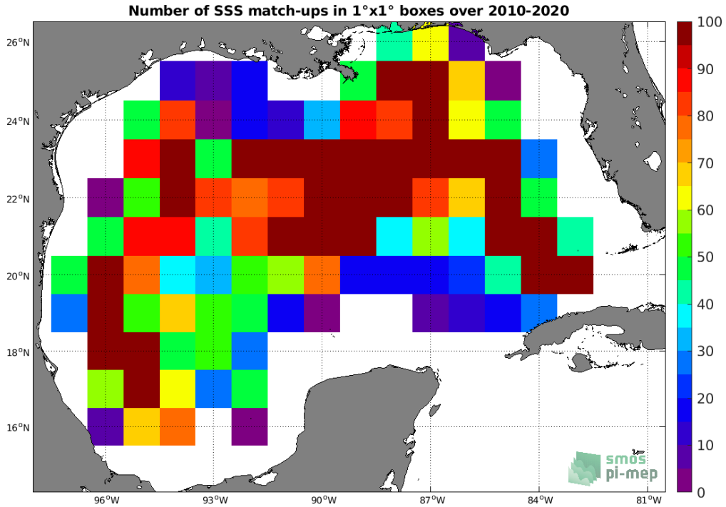
Figure 4: Number of SSS match-ups between Argo SSS and the CCI SSS L4 Merged-OI v3.2 - 30-day running (ESA) SSS product for the Gulf of Mexico Pi-MEP region over 1^\circ \times 1^\circ boxes and for the full satellite product period.
