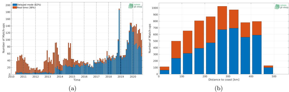
Figure 1: Number of match-ups between Argo and CCI SSS L4 Merged-OI v3.2 - 30-day running (ESA) SSS as a function of time (a) and as function of the distance to coast (b) over the Gulf of Mexico Pi-MEP region and for the full satellite product period.
