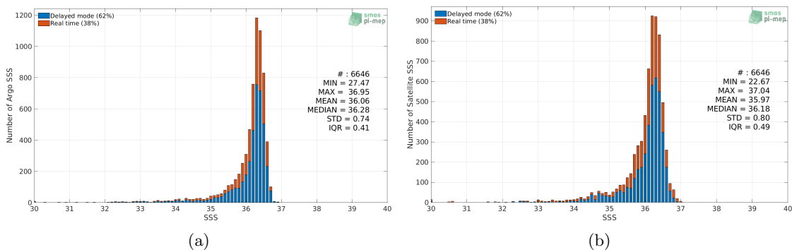
Figure 2: Histograms of SSS from Argo (a) and CCI SSS L4 Merged-OI v3.2 - 30-day running (ESA) (b) considering all match-up pairs per bins of 0.1 over the Gulf of Mexico Pi-MEP region and for the full satellite product period.
