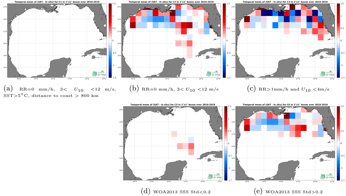
Figure 12: Temporal mean gridded over spatial boxes of size 1^{\circ}\times 1^{\circ} of \Delta\text{SSS} (CCI SSS L4 Merged-OI v2.31 - 30-day running (ESA) - TSG (SAMOS)) for 5 different subdatasets corresponding to: RR=0 mm/h, 3 < U_{10} < 12 m/s, SST >5^{\circ}\text{C} , distance to coast > 800 km (a), RR=0 mm/h, 3 < U_{10} < 12 m/s (b), RR >1 mm/h and U_{10} < 4 m/s (c), WOA2013 SSS Std <0.2 (d), WOA2013 SSS Std >0.2 (e).
