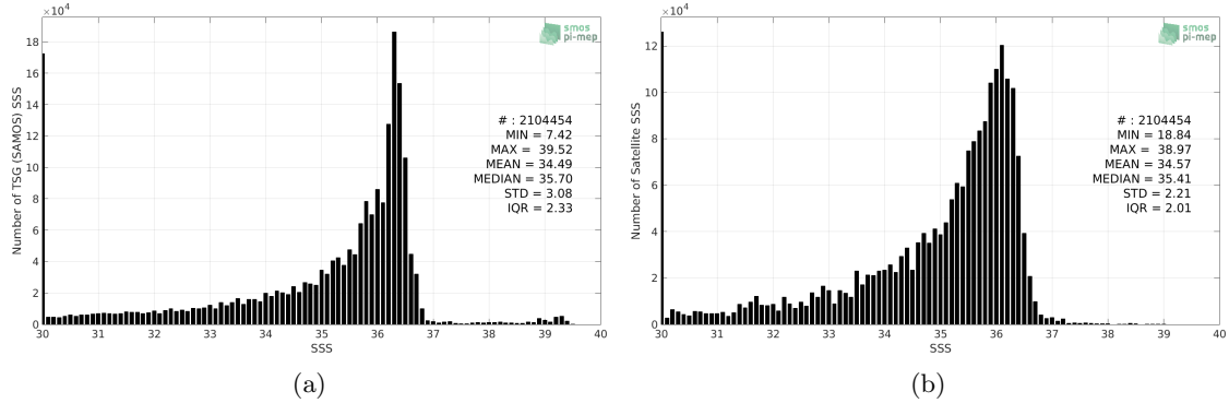
Figure 2: Histograms of SSS from TSG (SAMOS) (a) and CCI SSS L4 Merged-OI v2.31 - 30-day running (ESA) (b) considering all match-up pairs per bins of 0.1 over the Gulf of Mexico Pi-MEP region and for the full satellite product period.
