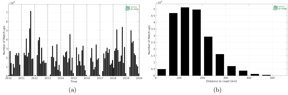
Figure 1: Number of match-ups between TSG (SAMOS) and CCI SSS L4 Merged-OI v2.31 - 30-day running (ESA) SSS as a function of time (a) and as function of the distance to coast (b) over the Gulf of Mexico Pi-MEP region and for the full satellite product period.
