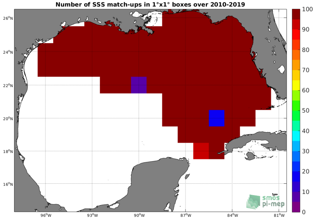
Figure 4: Number of SSS match-ups between TSG (SAMOS) SSS and the CCI SSS L4 Merged-OI v2.31 - 30-day running (ESA) SSS product for the Gulf of Mexico Pi-MEP region over 1^\circ \times 1^\circ boxes and for the full satellite product period.
