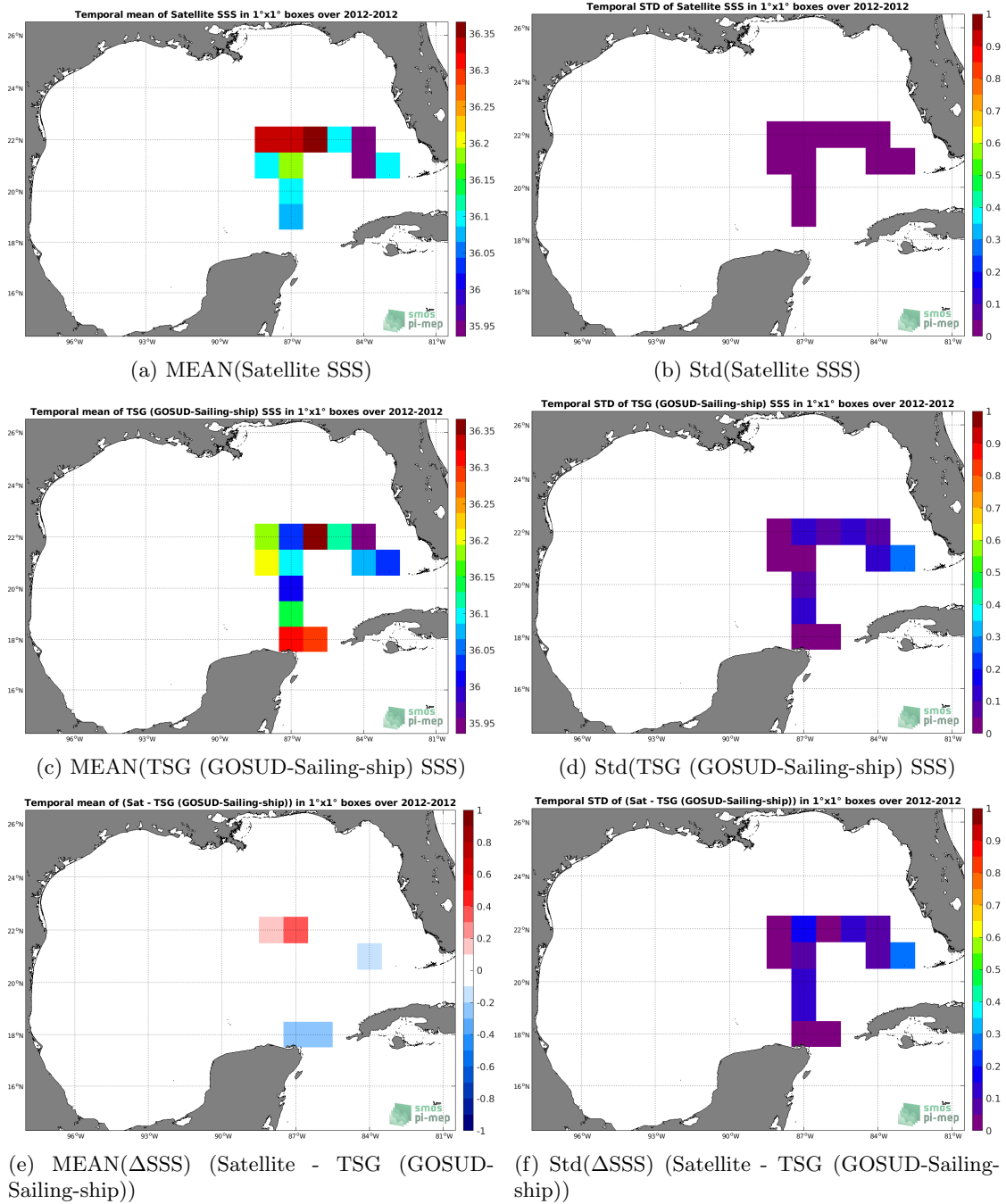
Figure 6: Temporal mean (left) and Std (right) of SSS from CCI SSS L4 Merged-OI v2.31 - 30-day running (ESA) (top), TSG (GOSUD-Sailing-ship) (middle), and of \Delta SSS (Satellite - TSG (GOSUD-Sailing-ship)). Only match-up pairs are used to generate these maps.
