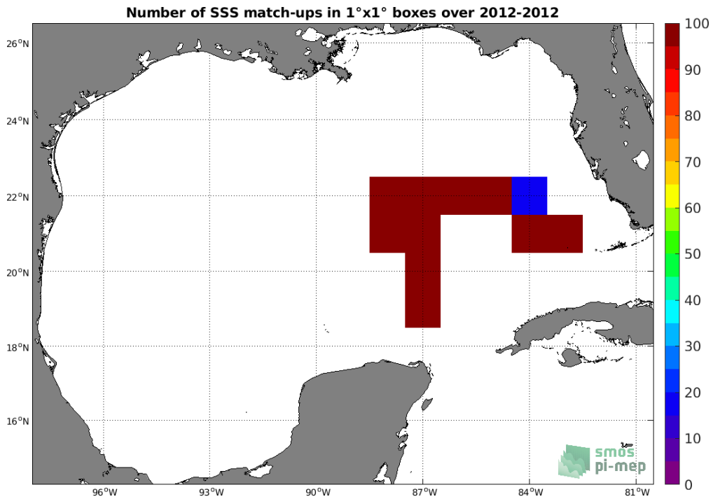
Figure 4: Number of SSS match-ups between TSG (GOSUD-Sailing-ship) SSS and the CCI SSS L4 Merged-OI v2.31 - 30-day running (ESA) SSS product for the Gulf of Mexico Pi-MEP region over 1°x1° boxes and for the full satellite product period.
